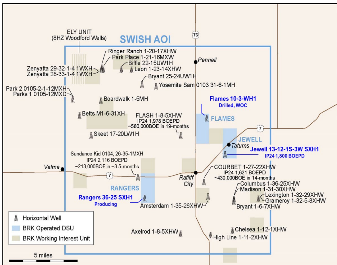
Figure 1. Location map showing the location of the Flames Well and Brookside's three operated SWISH AOI DSU's
