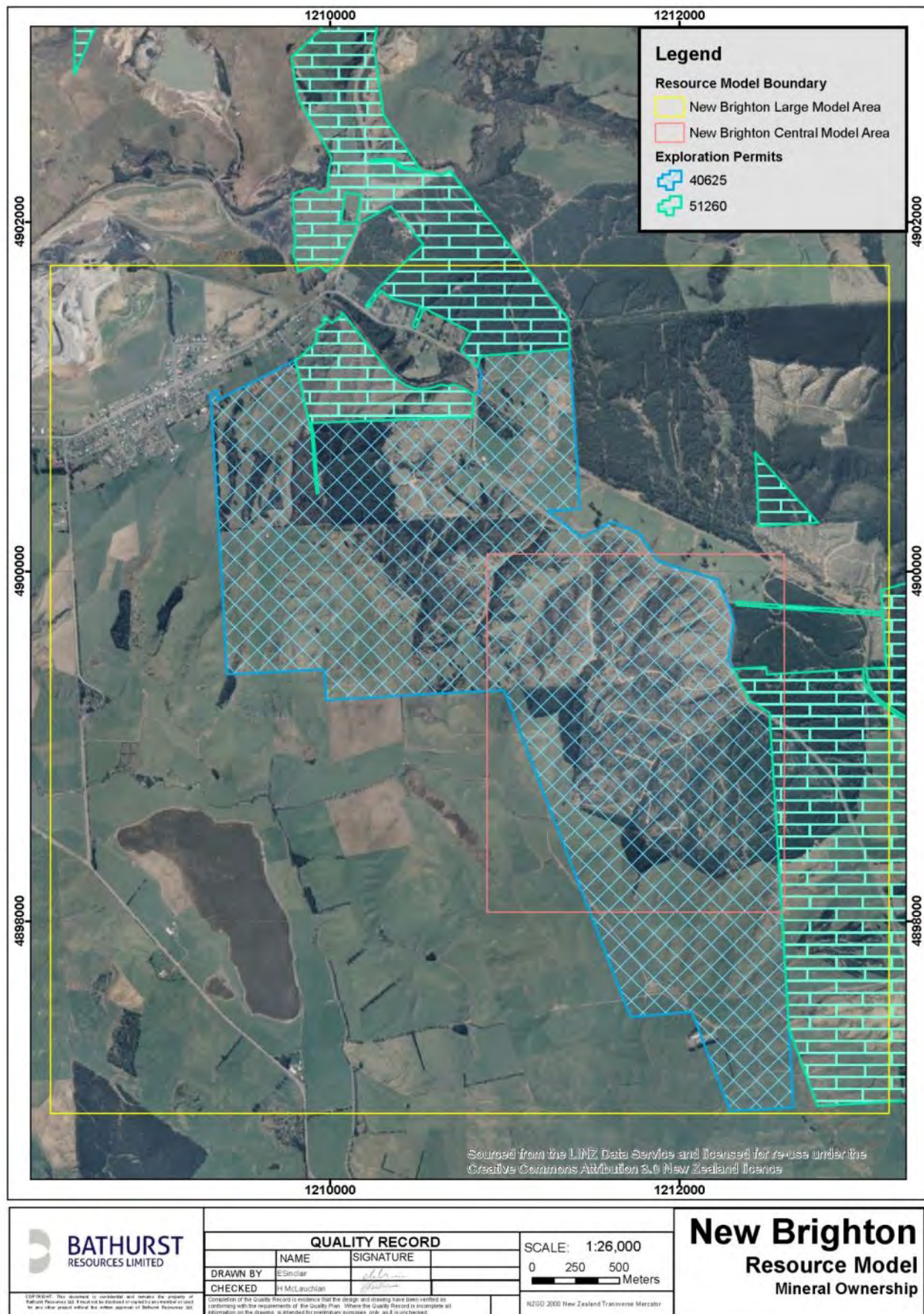
Figure 2 Shows BRL Owned Coal Exploration Permits within the New Brighton Model Area
