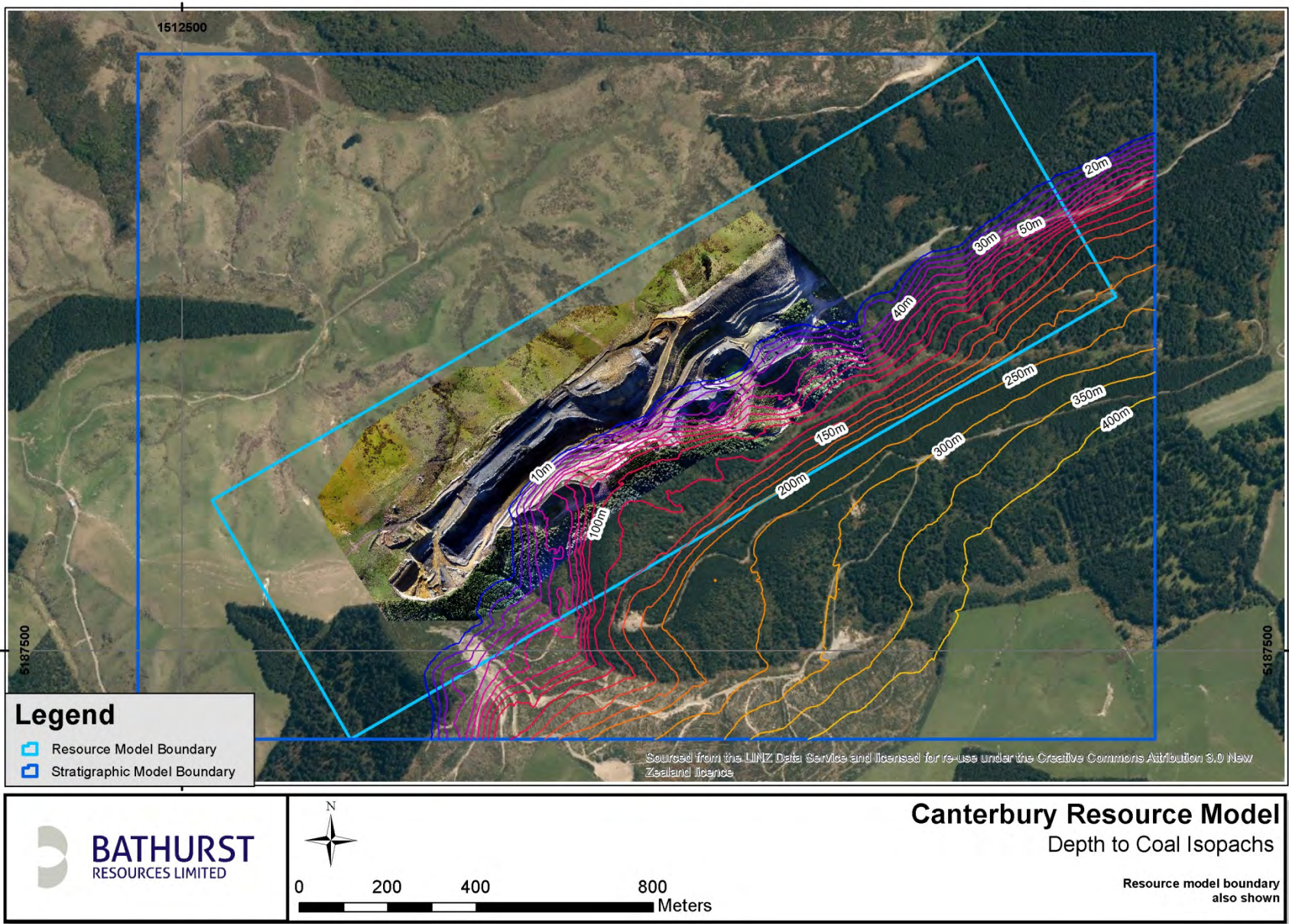
Figure 8 Depth to the upper most coal seam.
