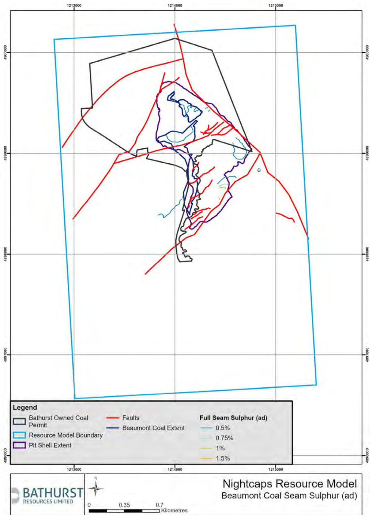
Figure 17: Beaumont Formation full seam Sulphur isopachs
