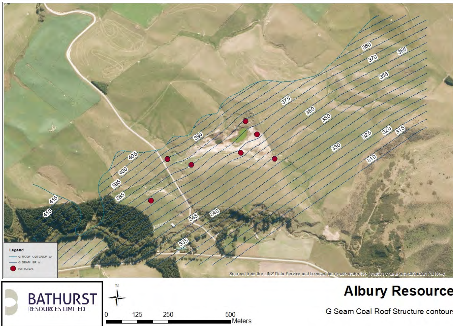
Figure 5: Structure contours of the G Seam roof
