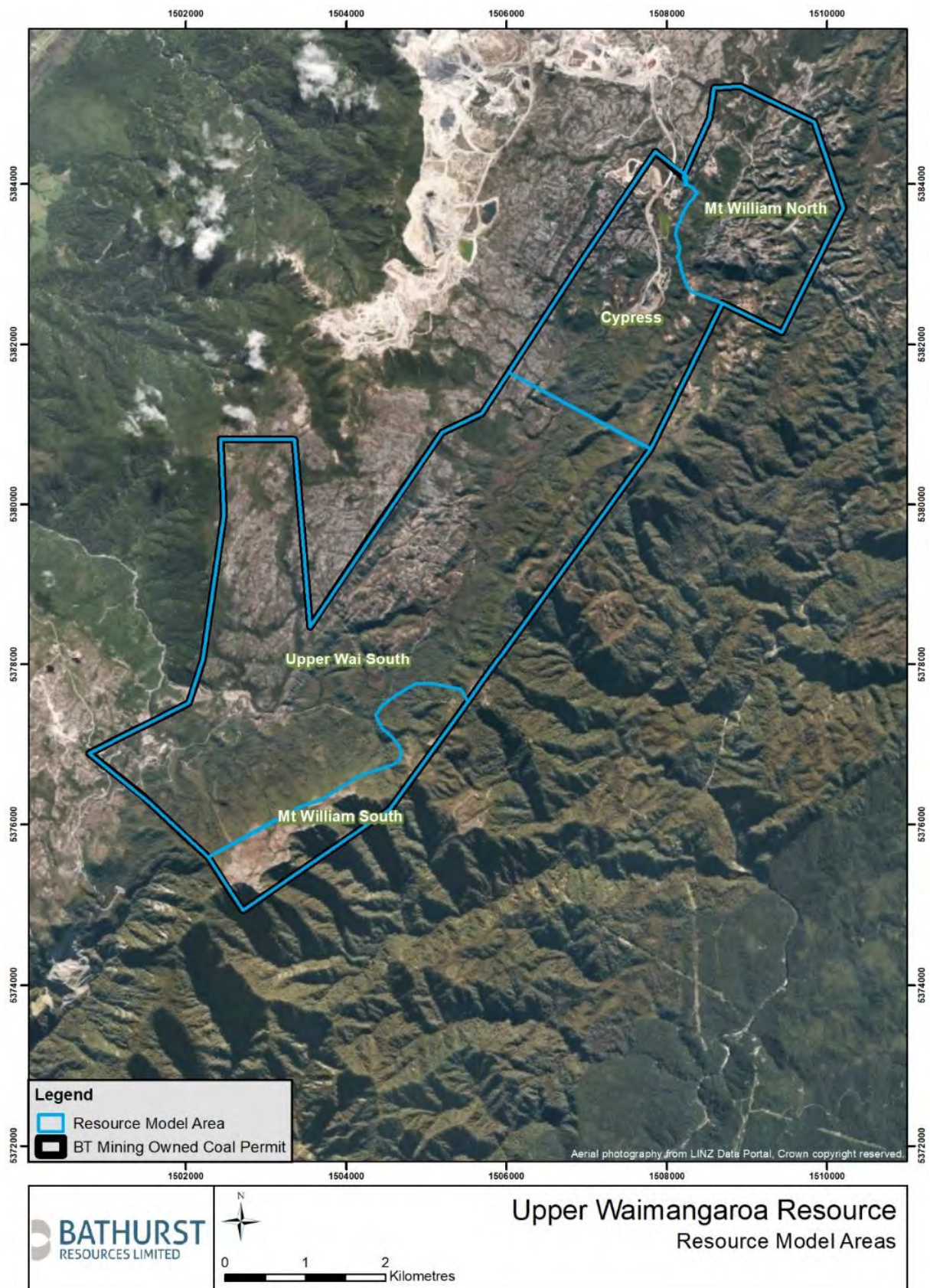
Figure 2: Resource Model Areas
