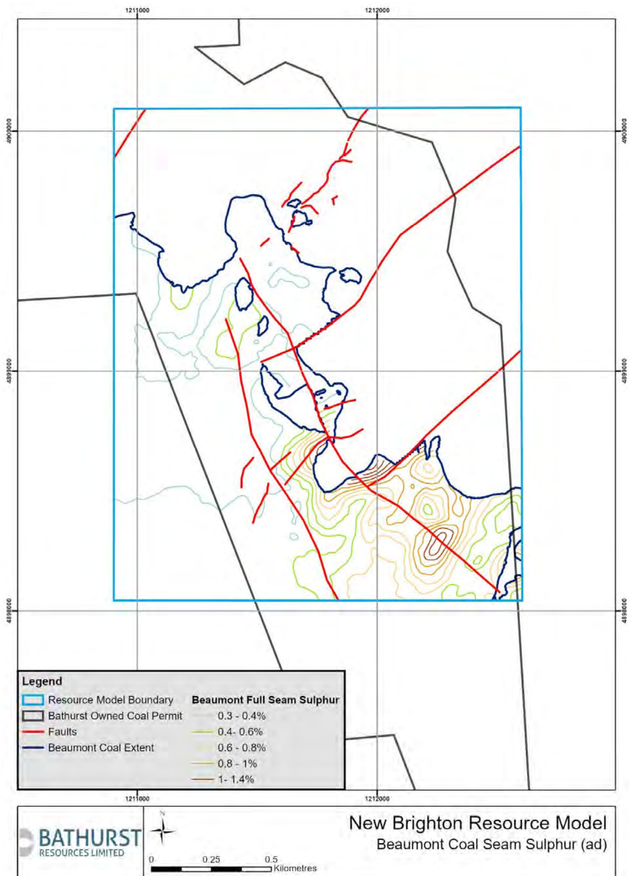
Figure 8: Beaumont Formation full seam sulphur isopachs
