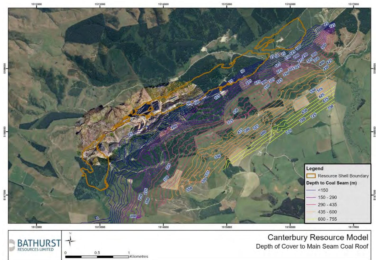
Figure 7: Depth to the Main coal seam roof
