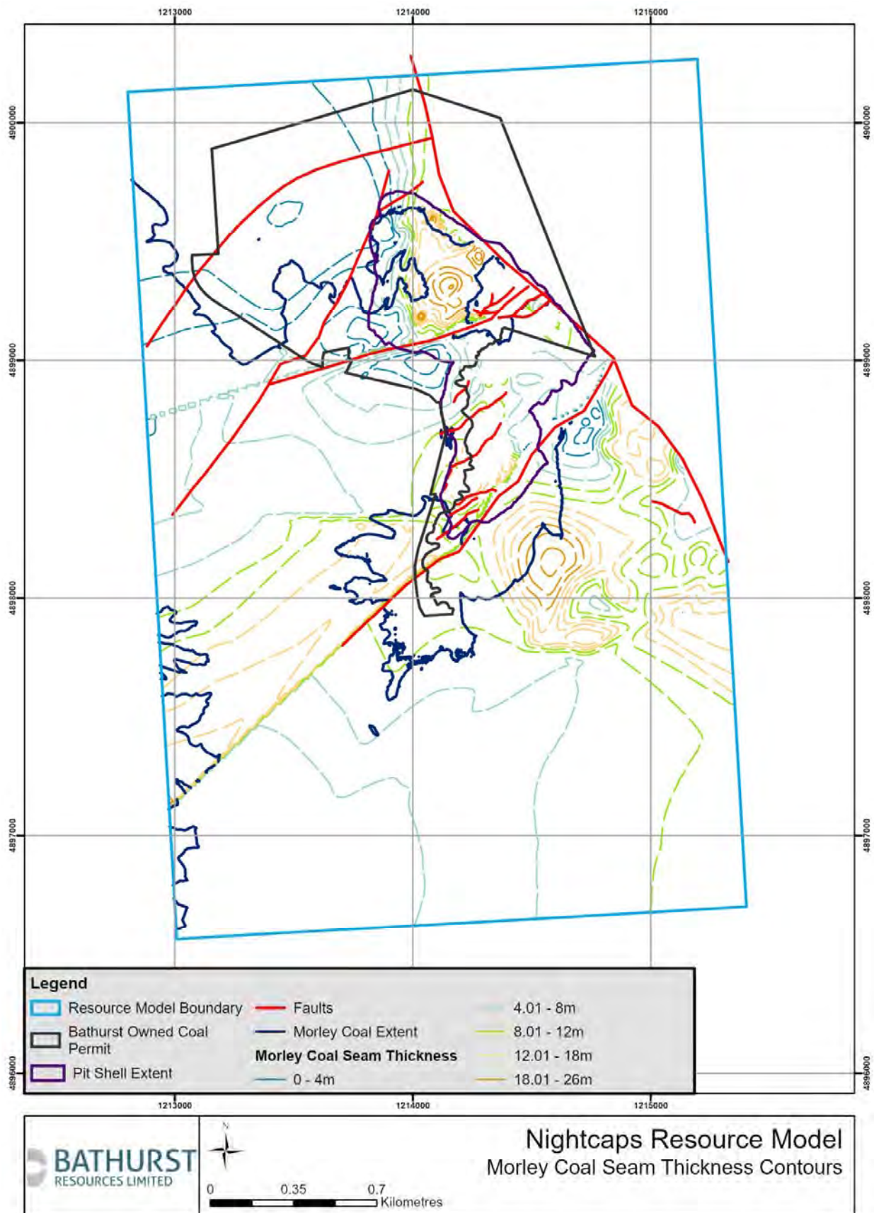
Figure 19: Morley Formation full seam cumulative coal thickness isopachs
