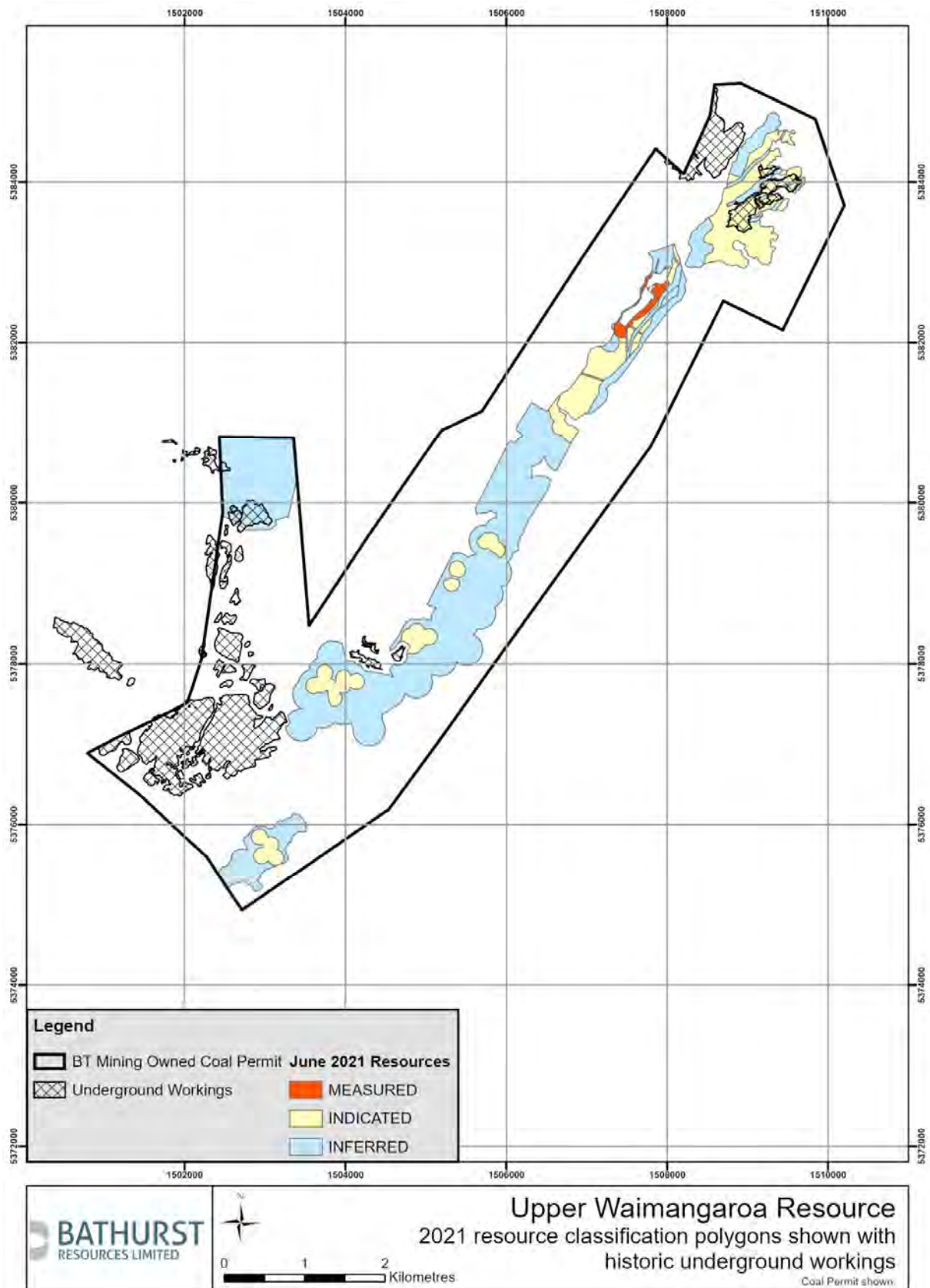
Figure 7: Extent of Underground Workings and 2021 resource classification
