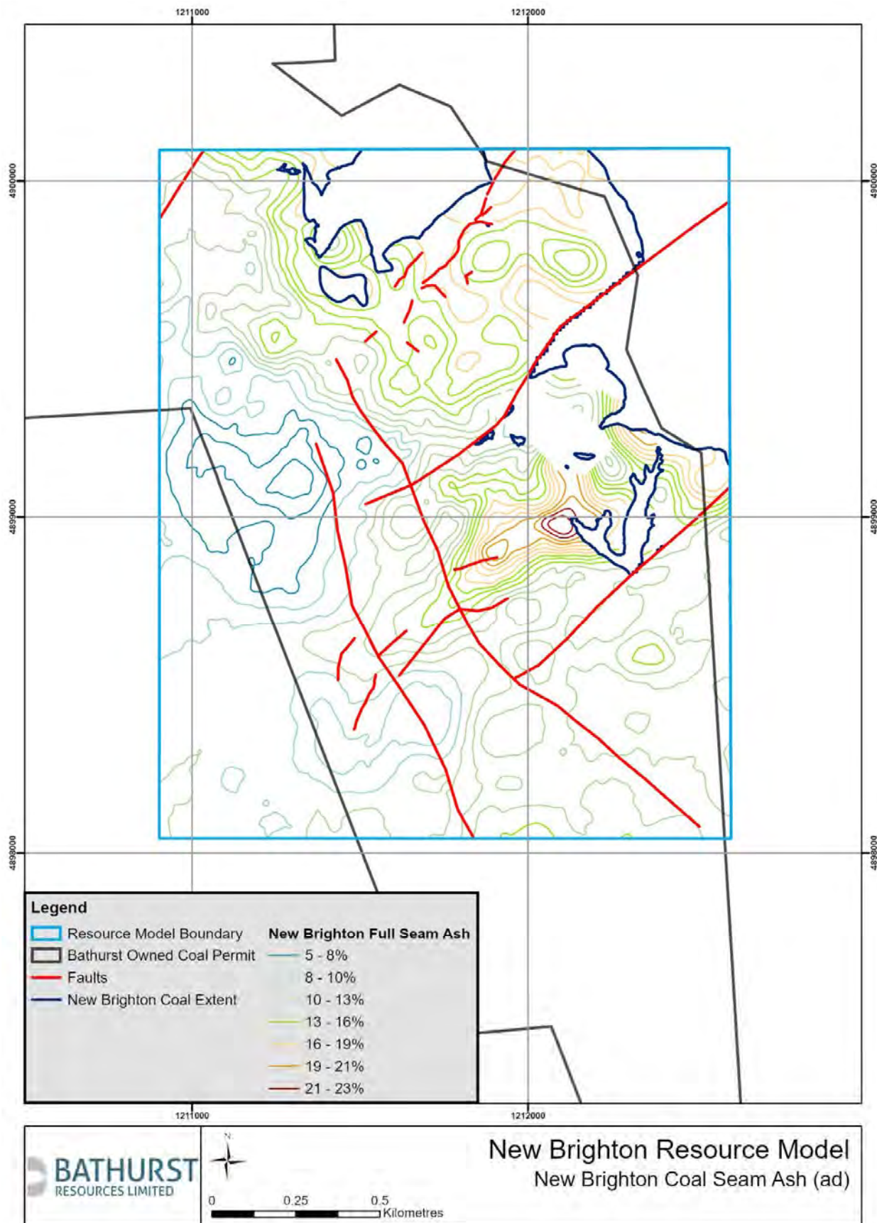
Figure 15: New Brighton Formation full seam ash isopachs
