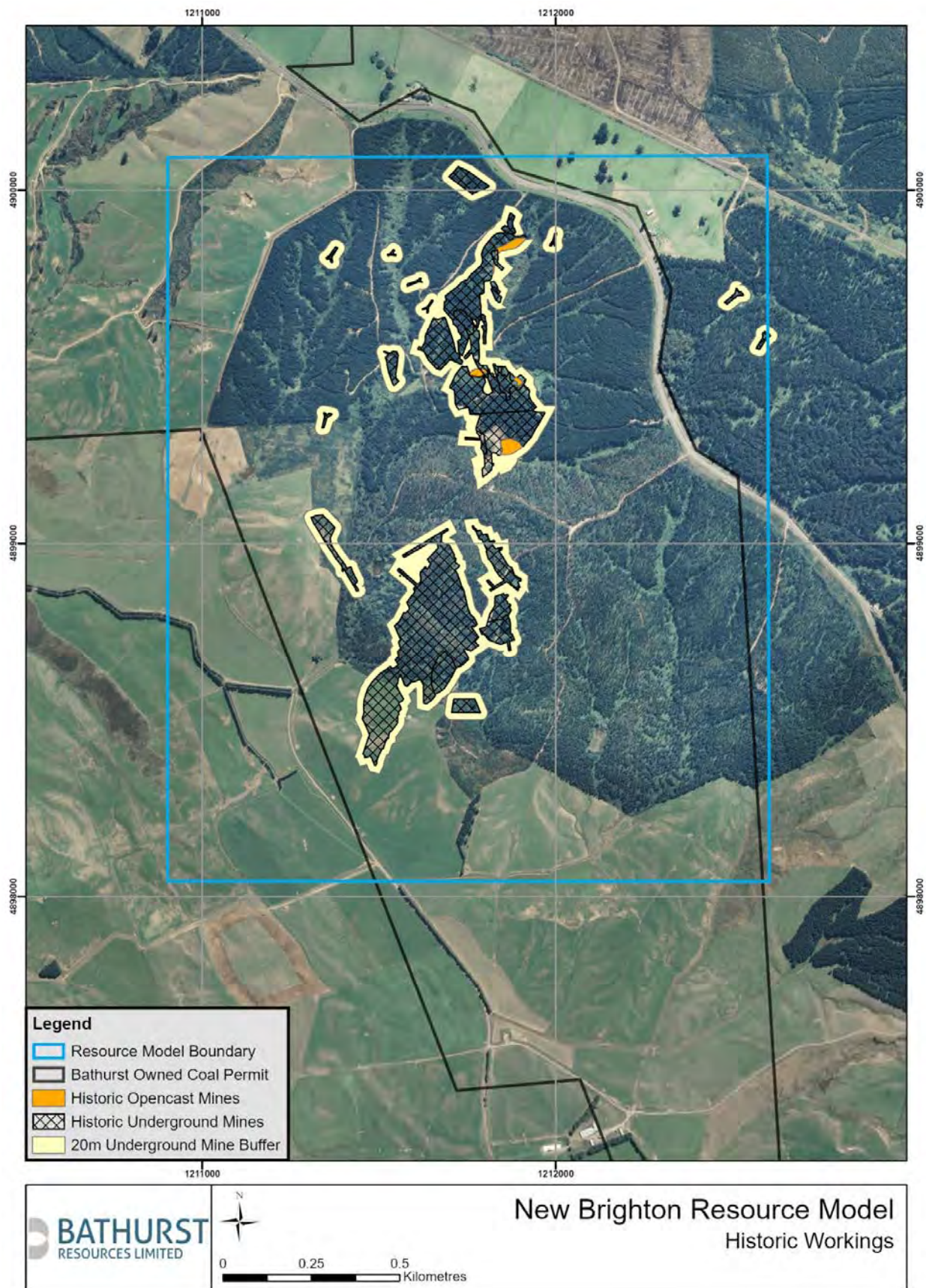
Figure 4: Location of historical mine workings. Note: recent opencast mined areas are not shown
