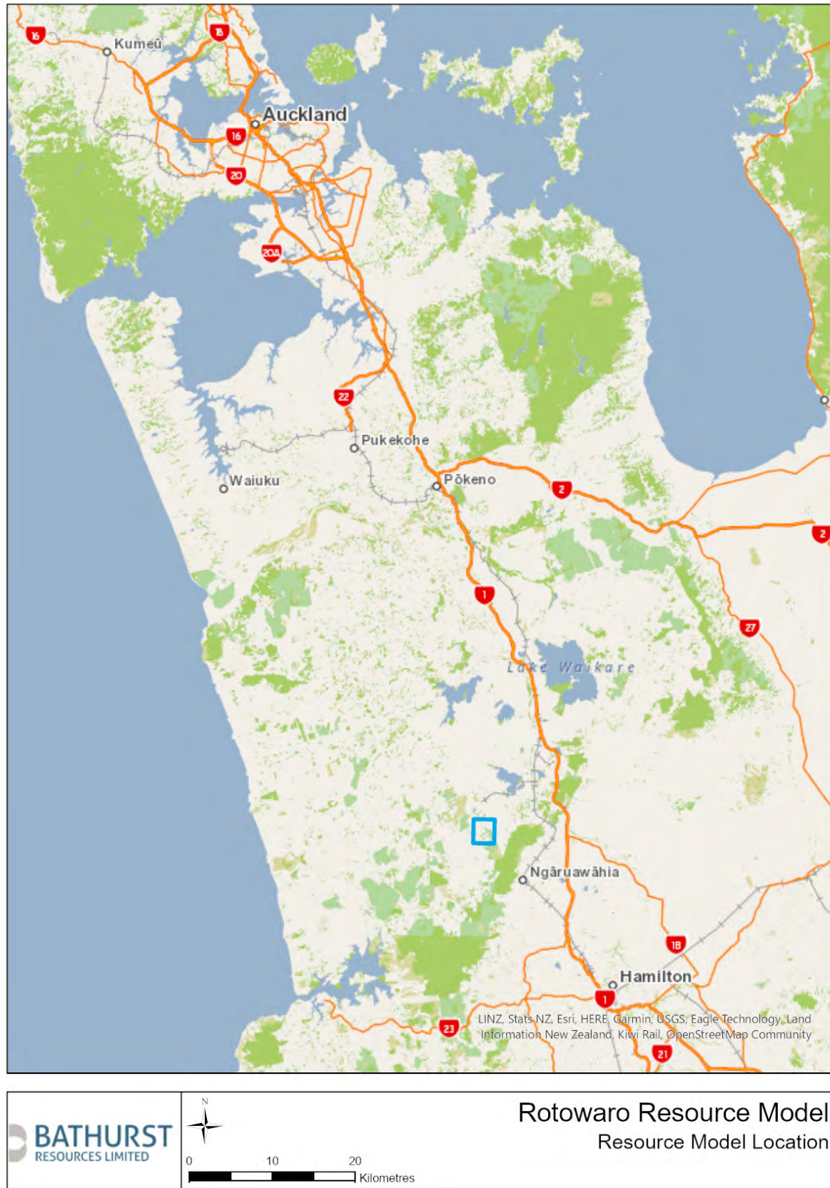
Figure 1: Location map of Rotowaro
