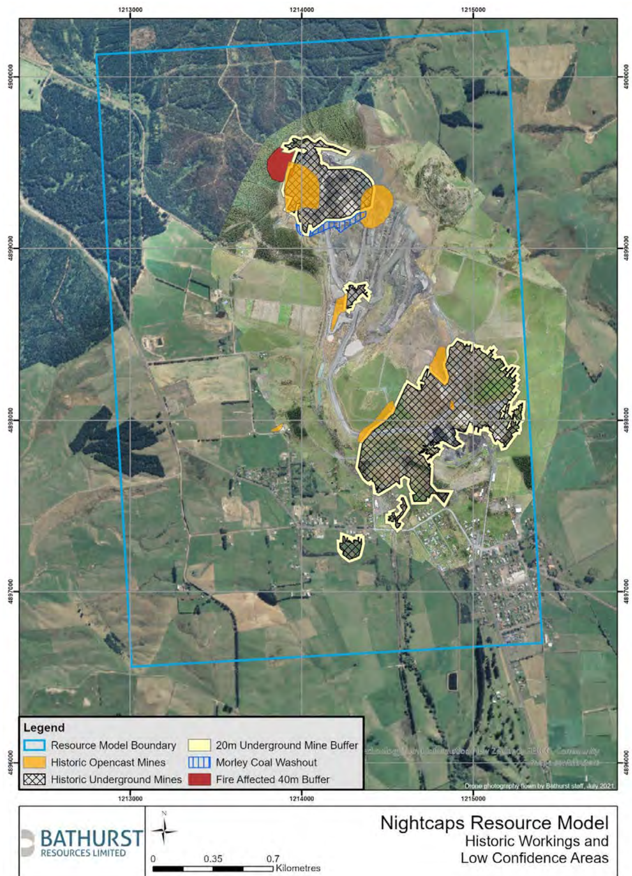
Figure 13: Location of historic mine workings and areas of low confidence. Note: Recent opencast mined areas are not shown.
