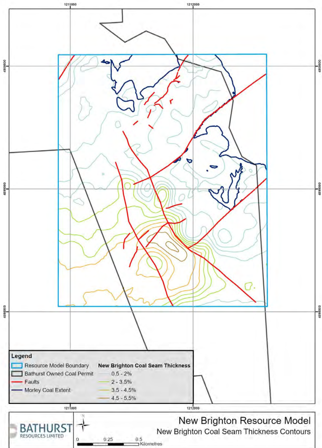
Figure 14: New Brighton Formation cumulative coal thickness isopachs
