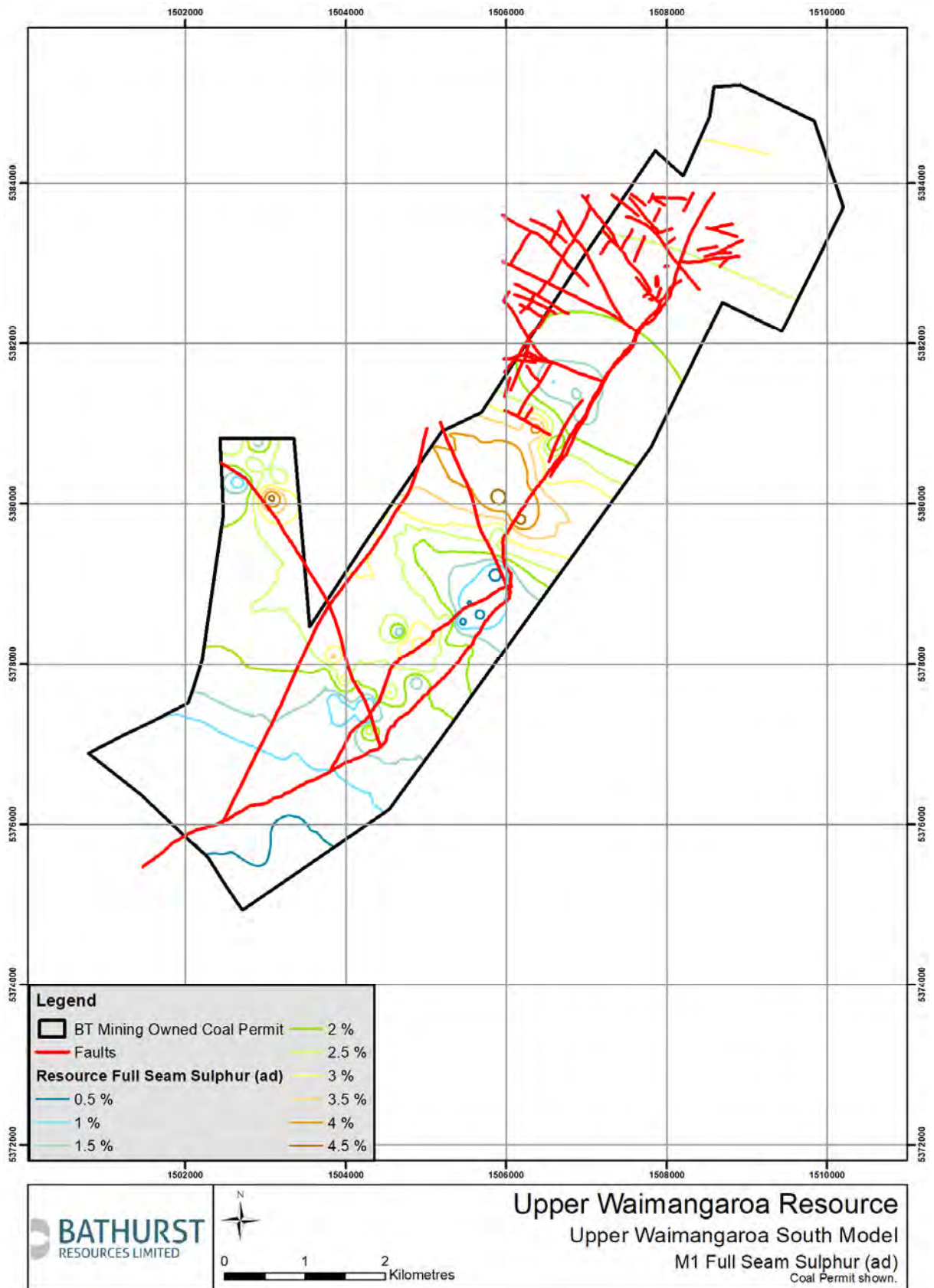
Figure 13: Plan showing full M1 seam sulphur on an air dried basis across the Upper Wiamangaroa South resource
