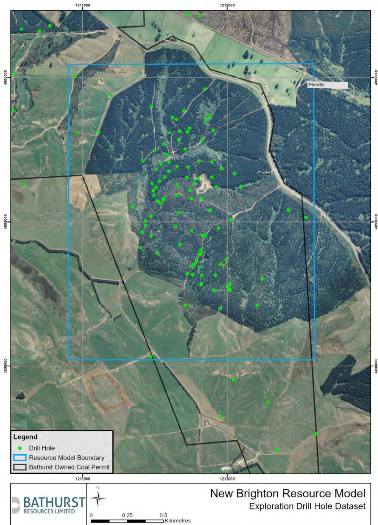
Figure 3: Location of drilling within Coal Resource area
