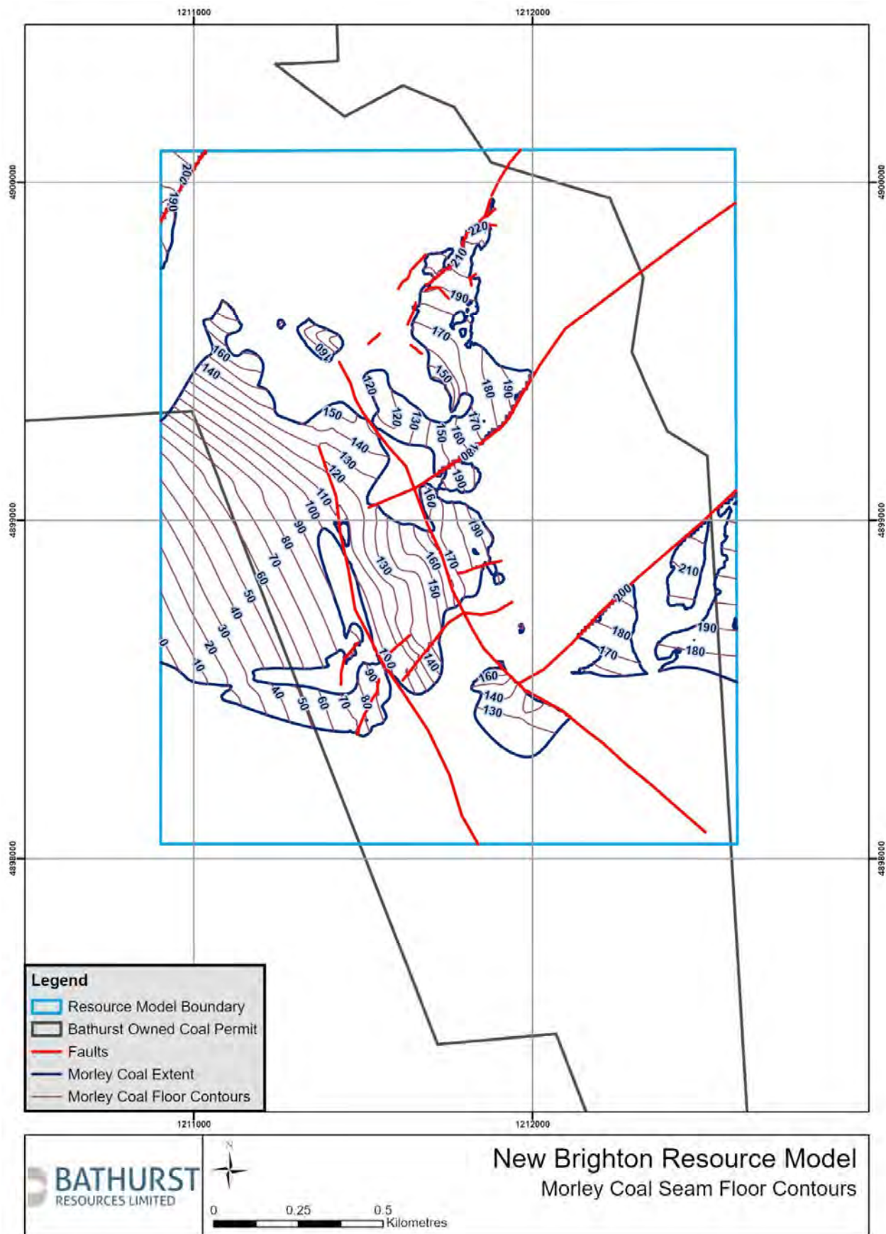
Figure 9: Morley UM1 seam coal floor contours
