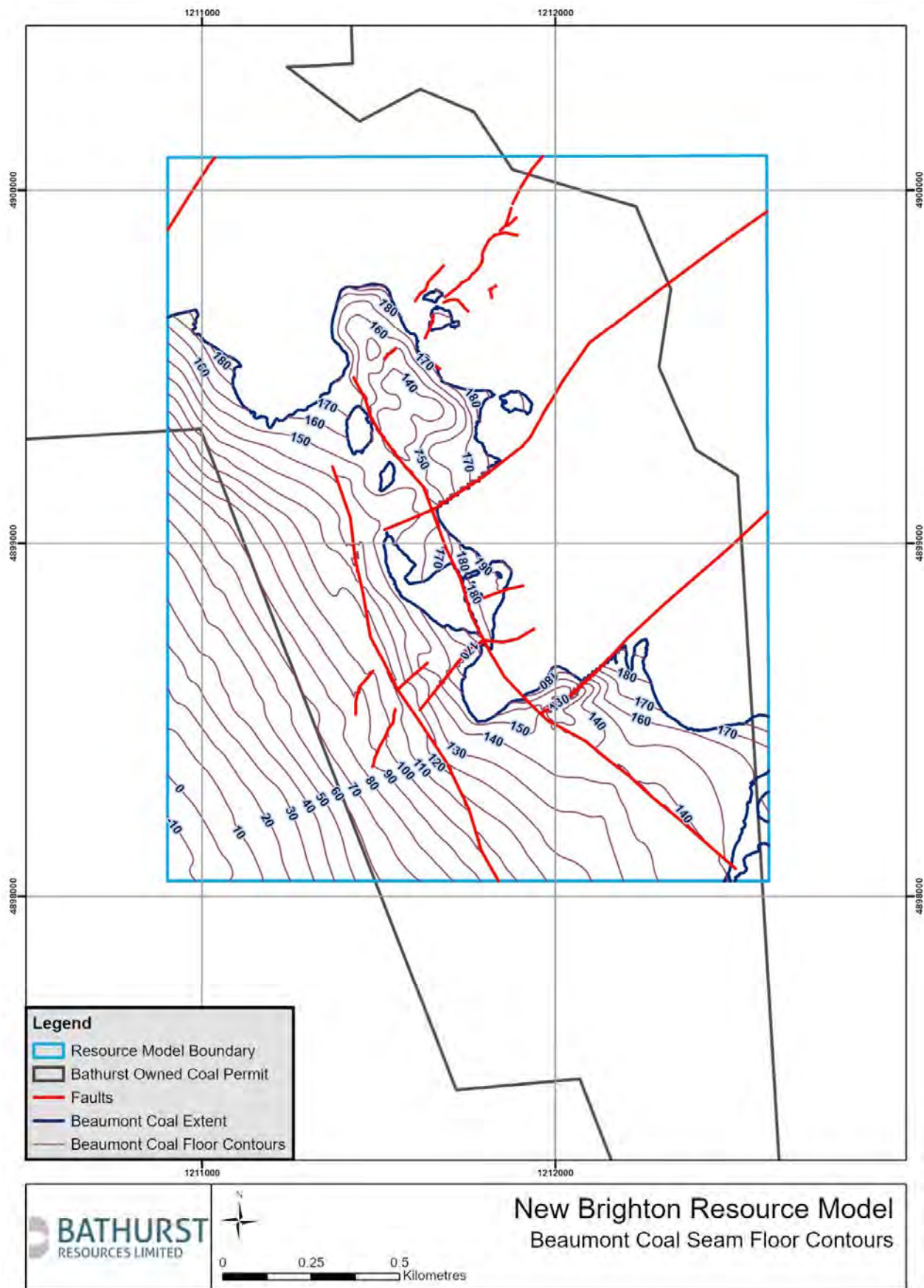
Figure 5: Beaumont Formation coal floor contours
