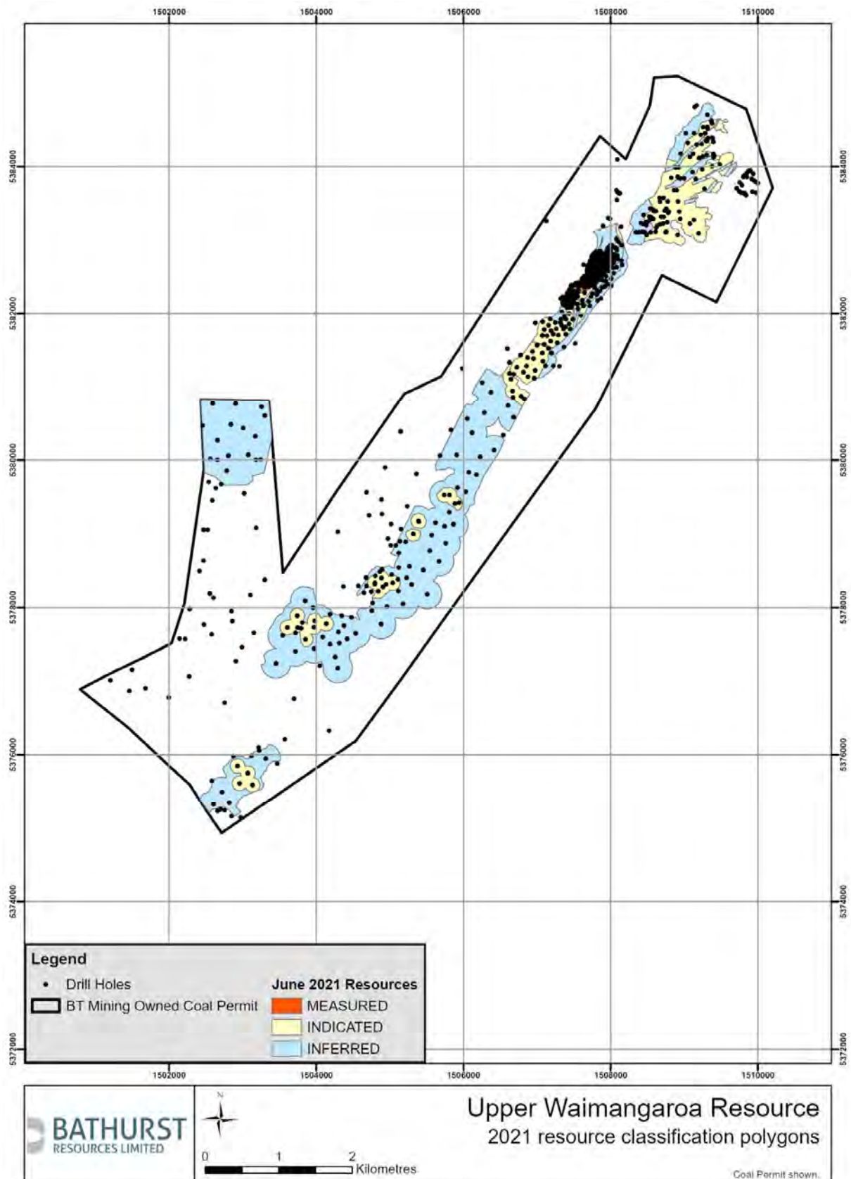
Figure 6: Plan showing the 2021 drillhole coverage and resource classification polygons
