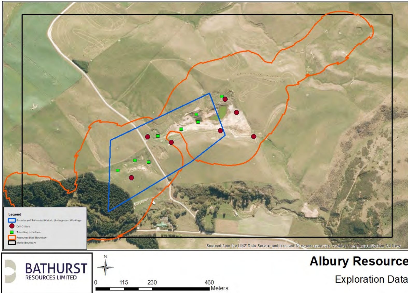
Figure 4: Exploration drill hole dataset and extent of historical underground coal mines for the Albury Project
