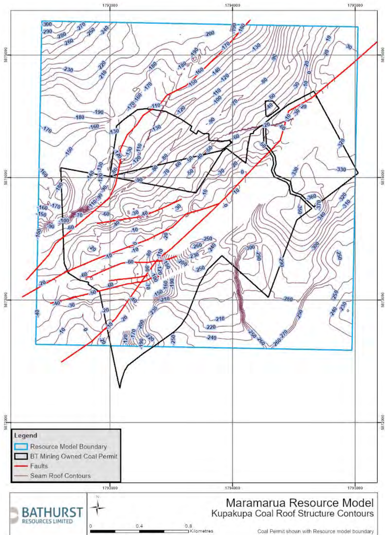
Figure 7: Plan showing the structure contours of the coal seam roof
