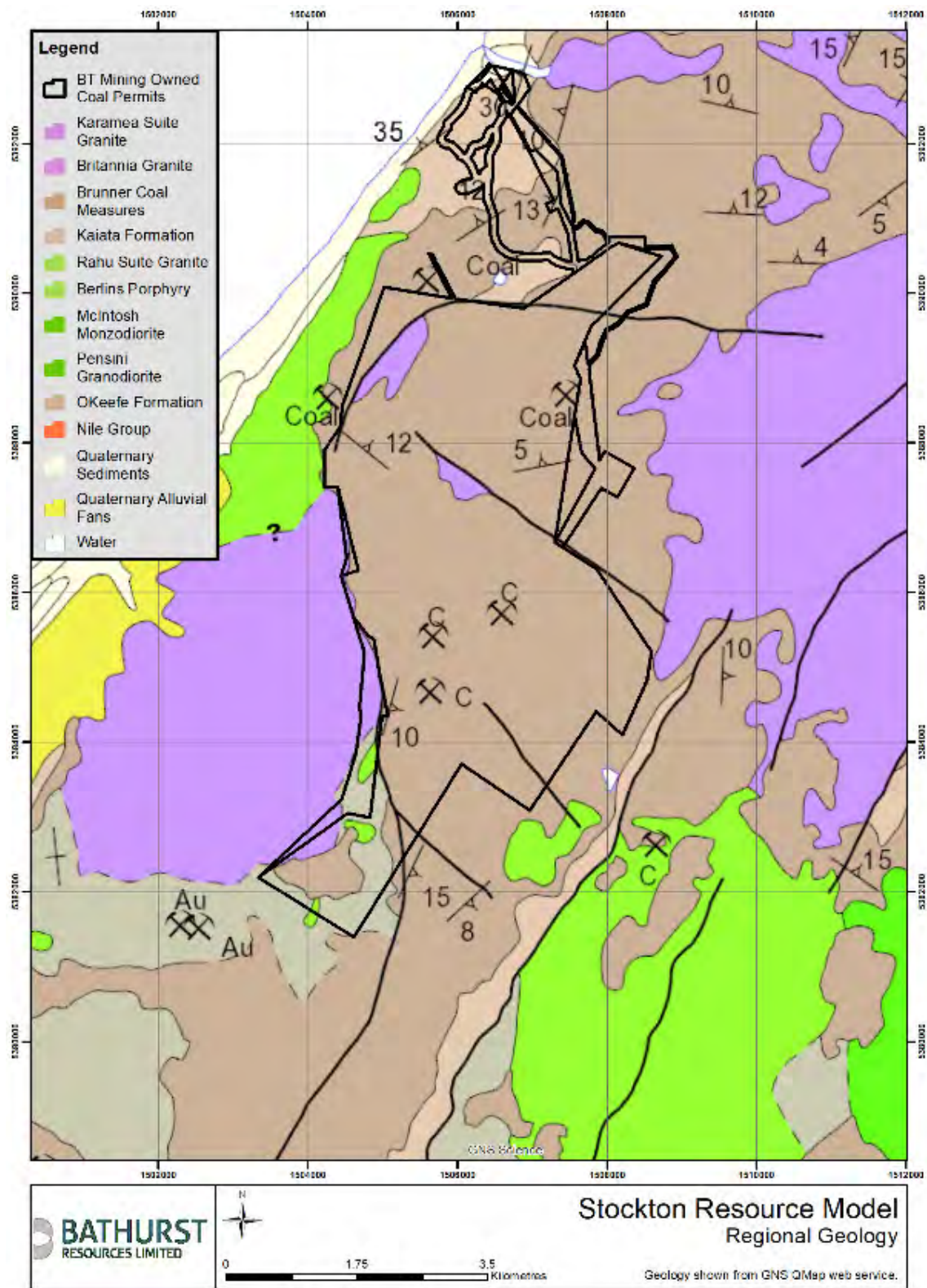
Figure 4: Geological QMap across the mine site
