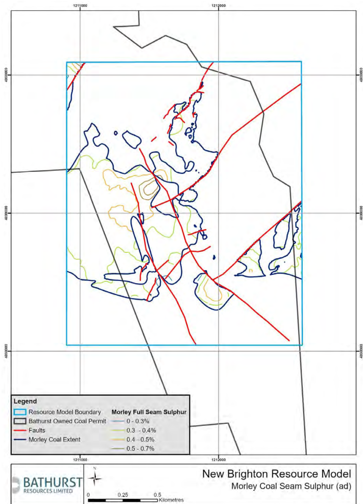
Figure 12: Morley Formation full seam sulphur isopachs
