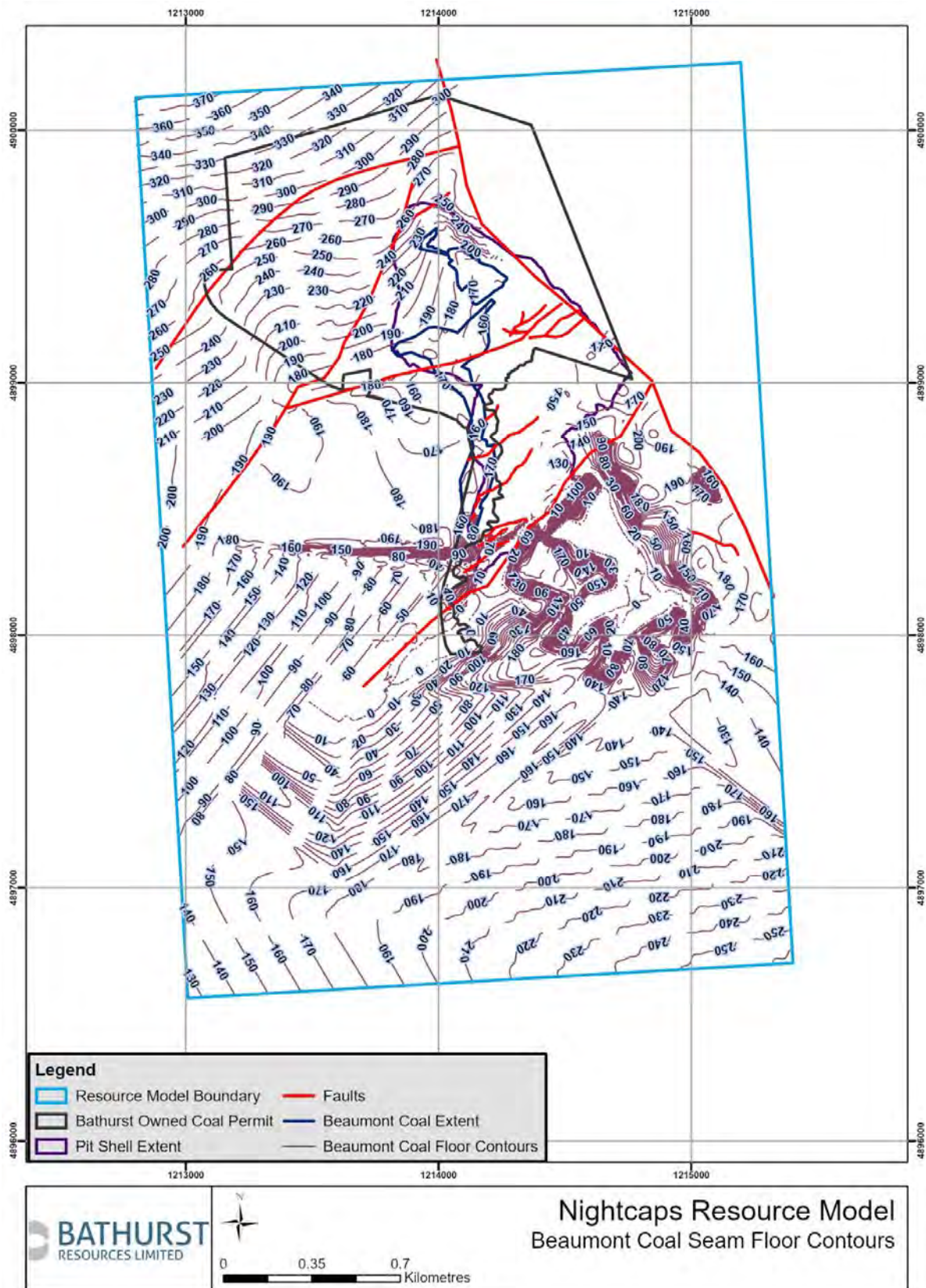
Figure 14: Beaumont Formation coal floor contours
