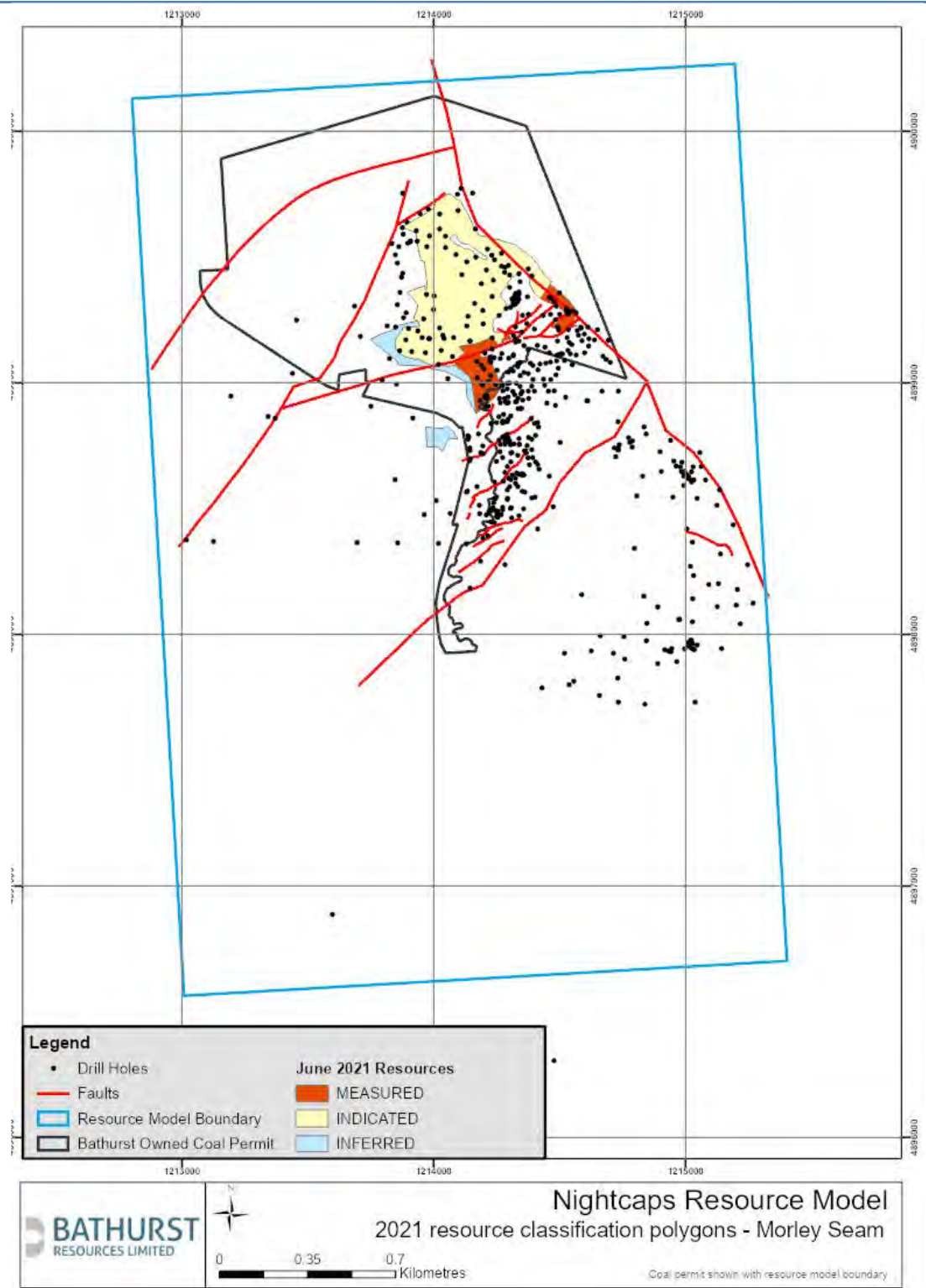
Figure 6: Morley Coal Resource classification areas
