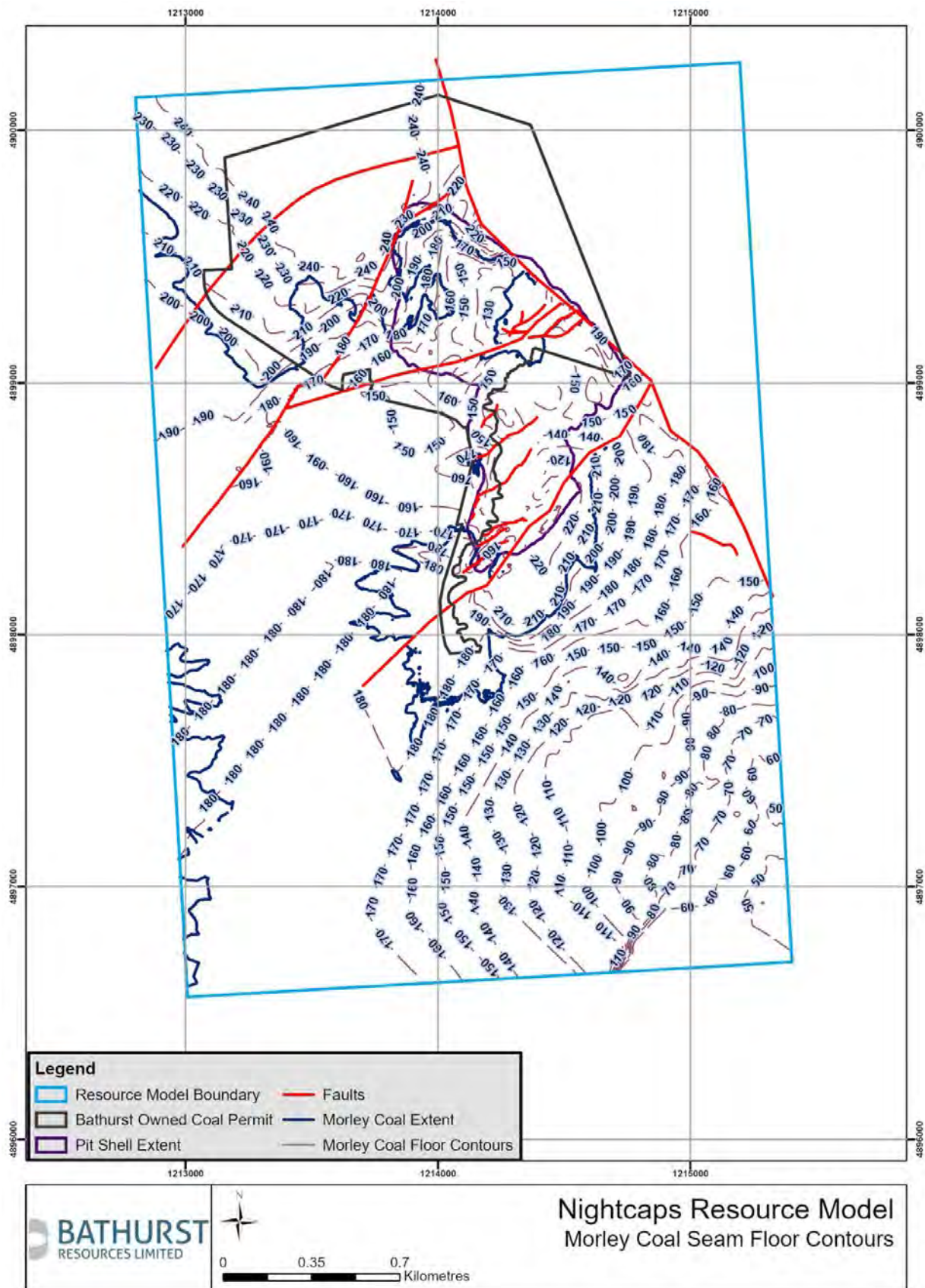
Figure 18: Morley Formation coal floor contours
