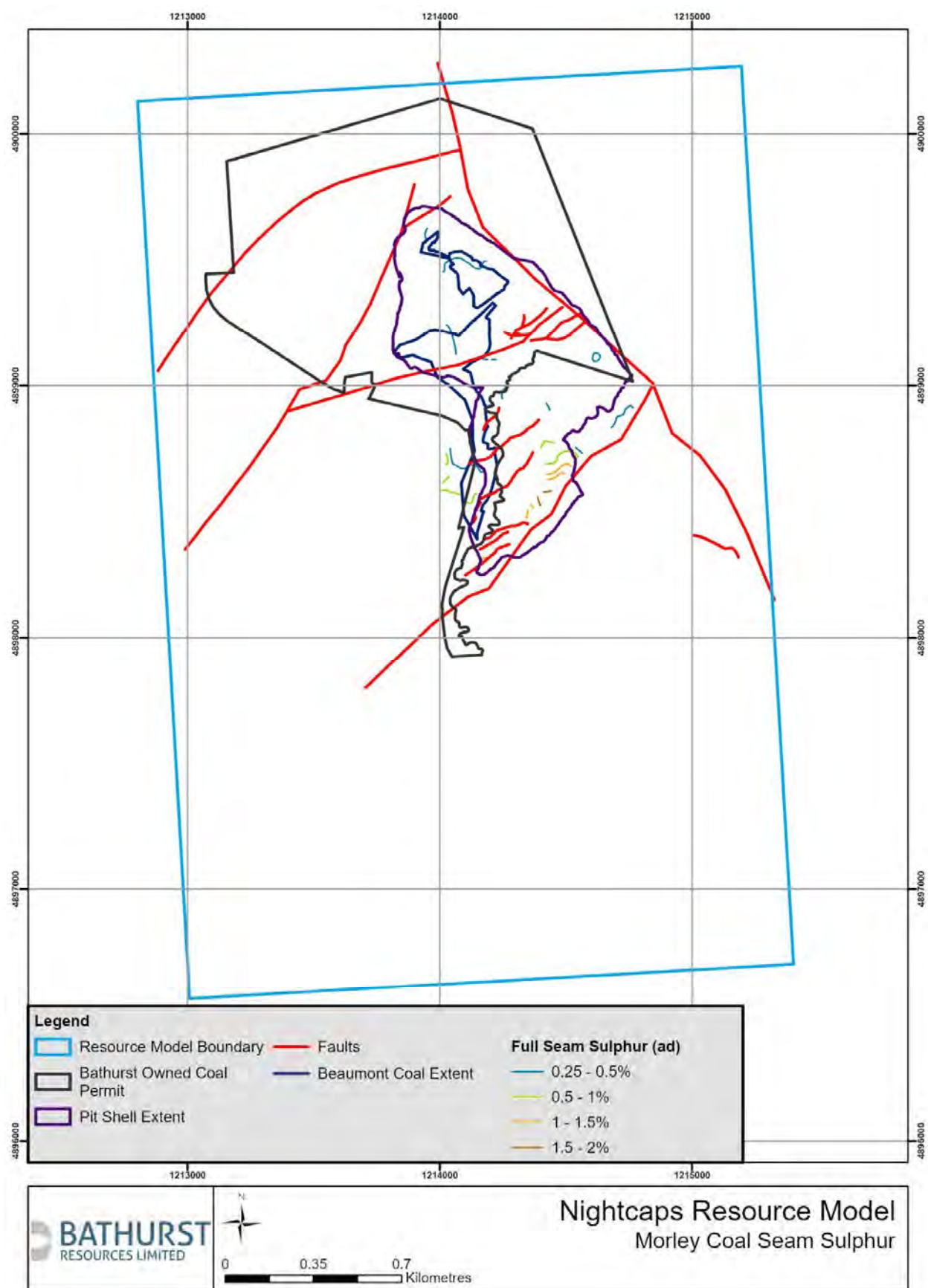
Figure 21: Morley Formation full seam air dried Sulphur isopachs
