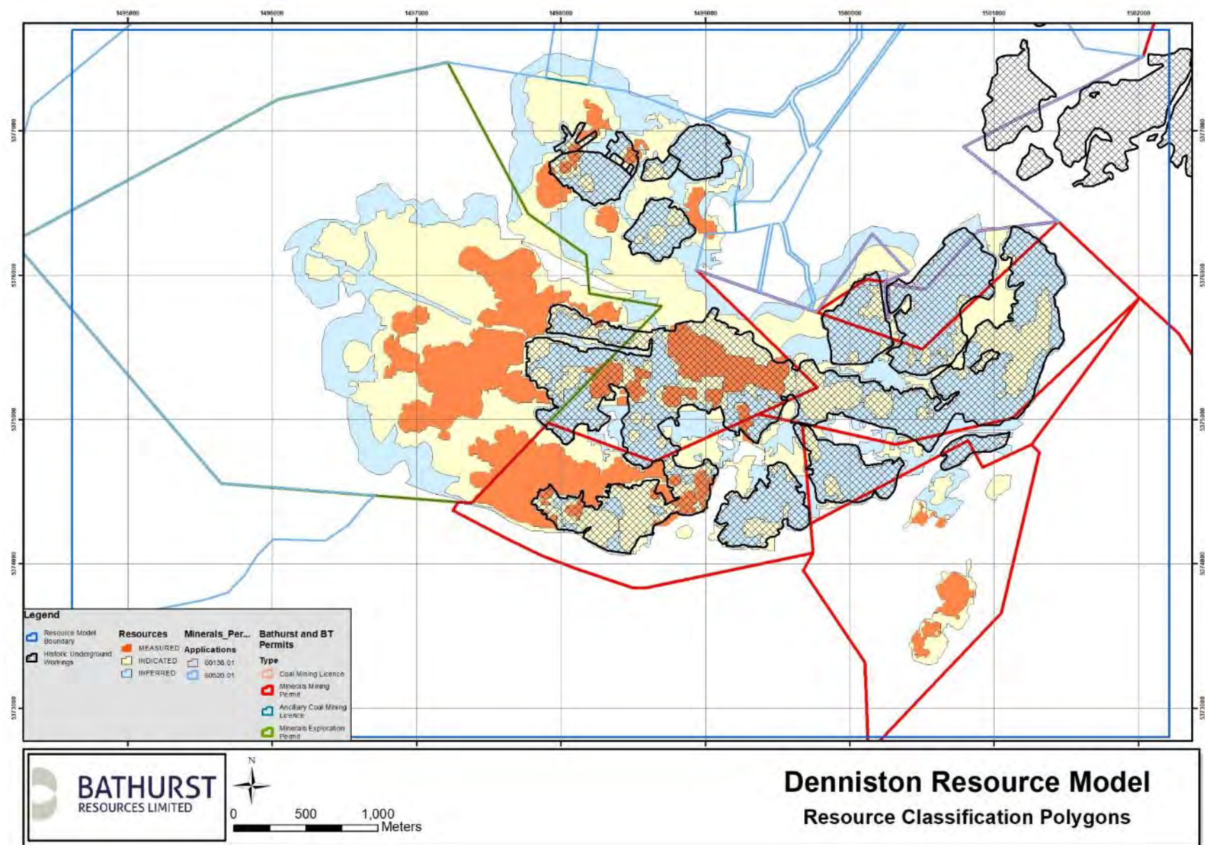
Figure 6: Extent of underground workings and resource classification
