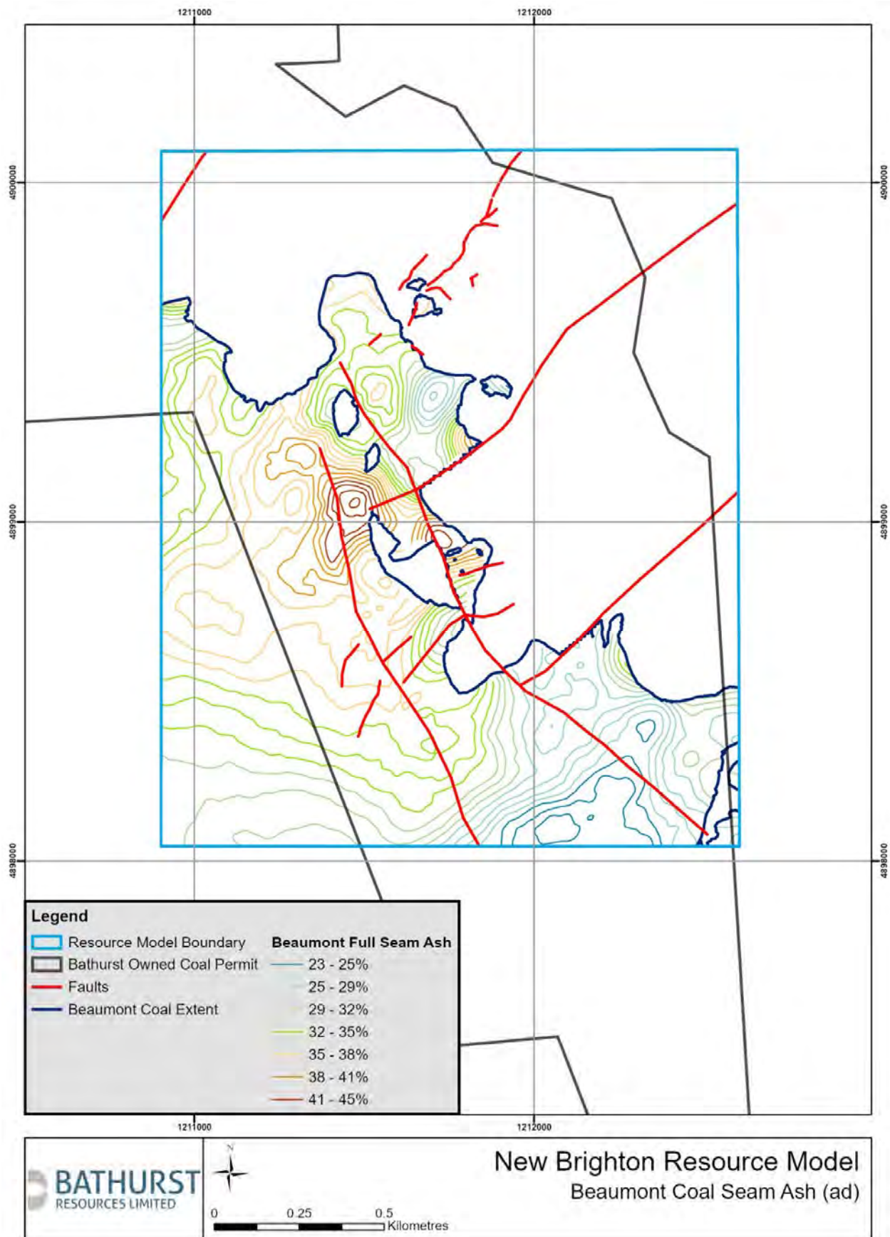
Figure 7: Beaumont Formation full seam ash isopachs
