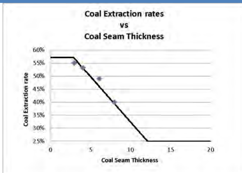
Figure 2: Historical underground extraction rates applied to areas of underground workings based on coal seam thickness
