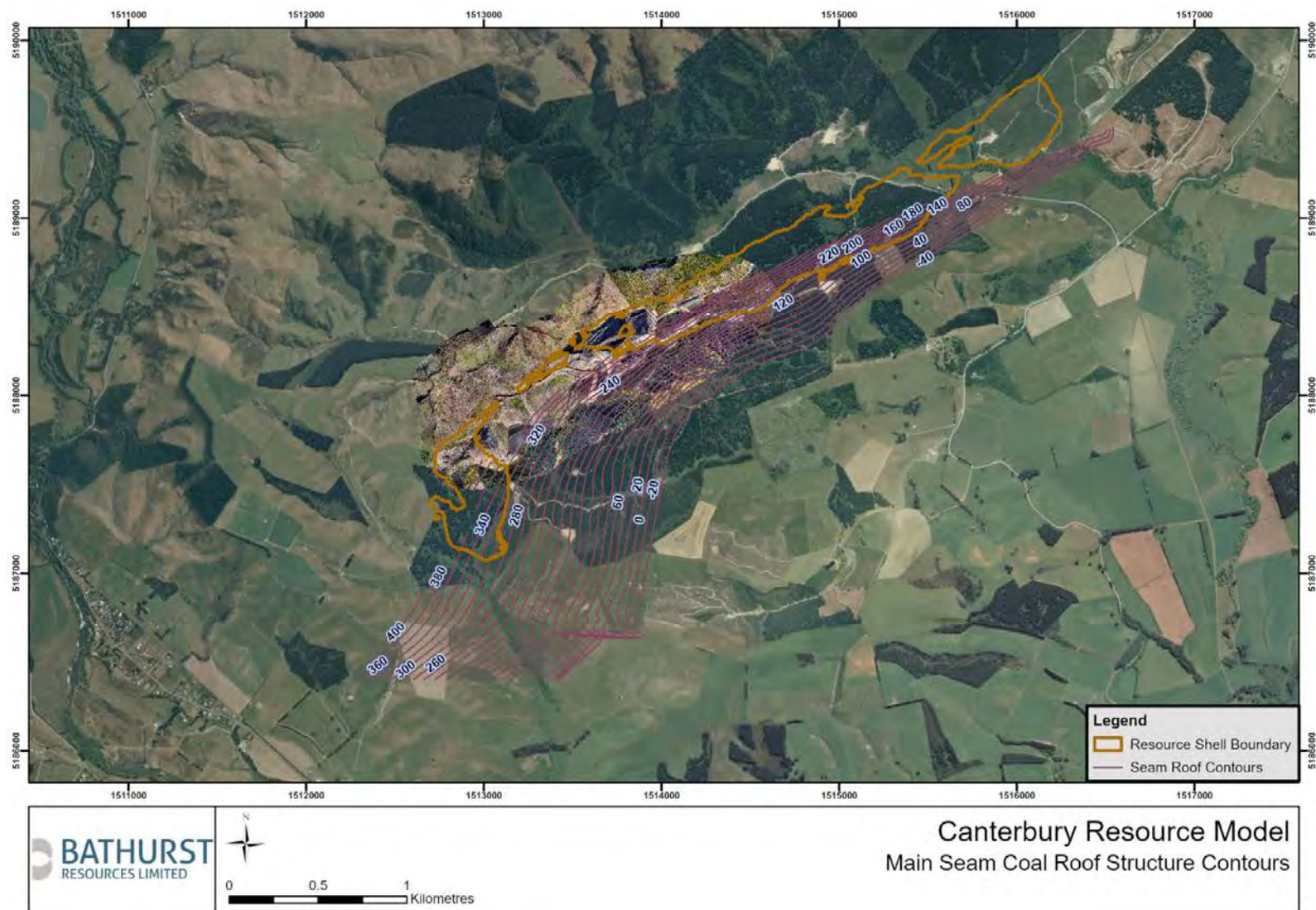
Figure 6: Structure contours of the Main Seam roof
