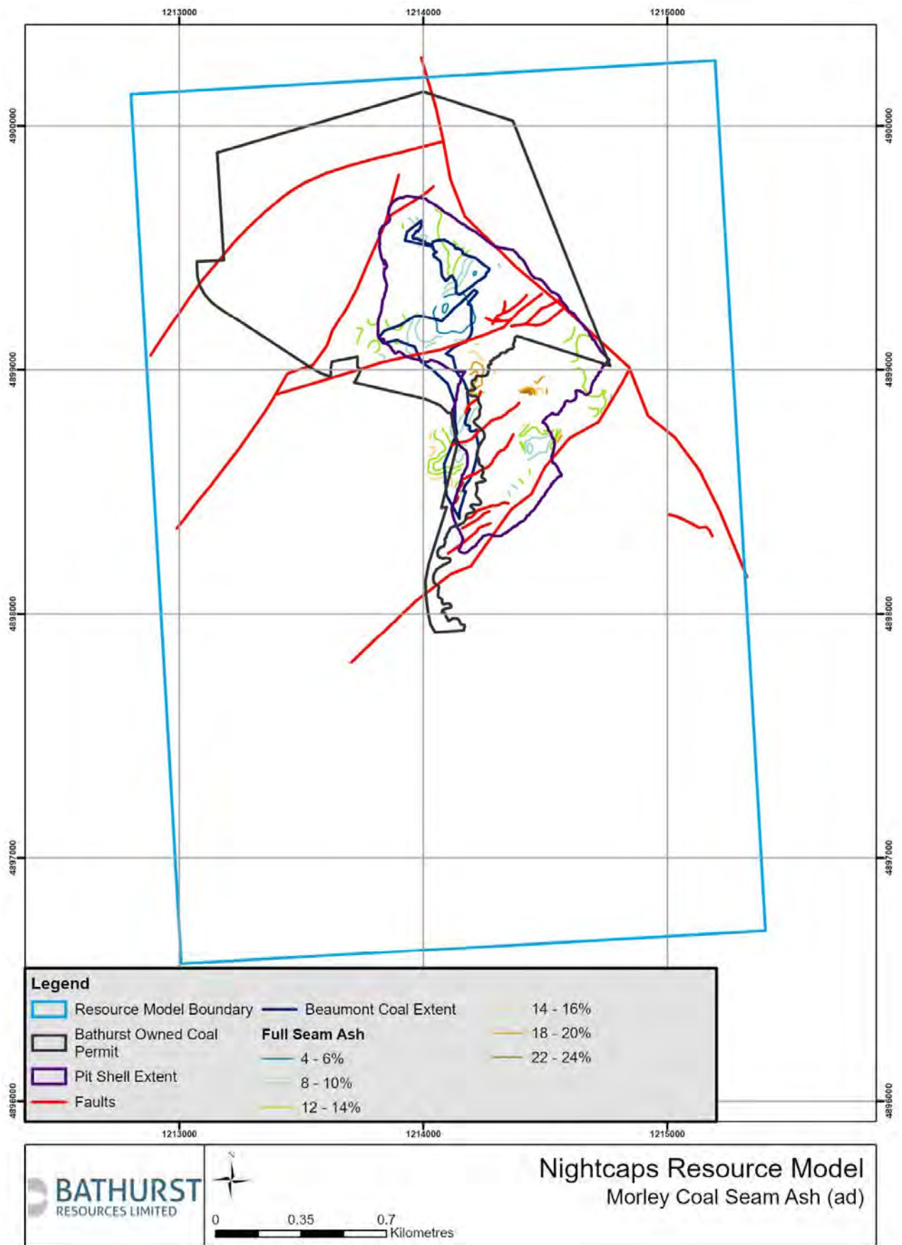
Figure 20: Morley Formation full seam air dried ash isopachs
