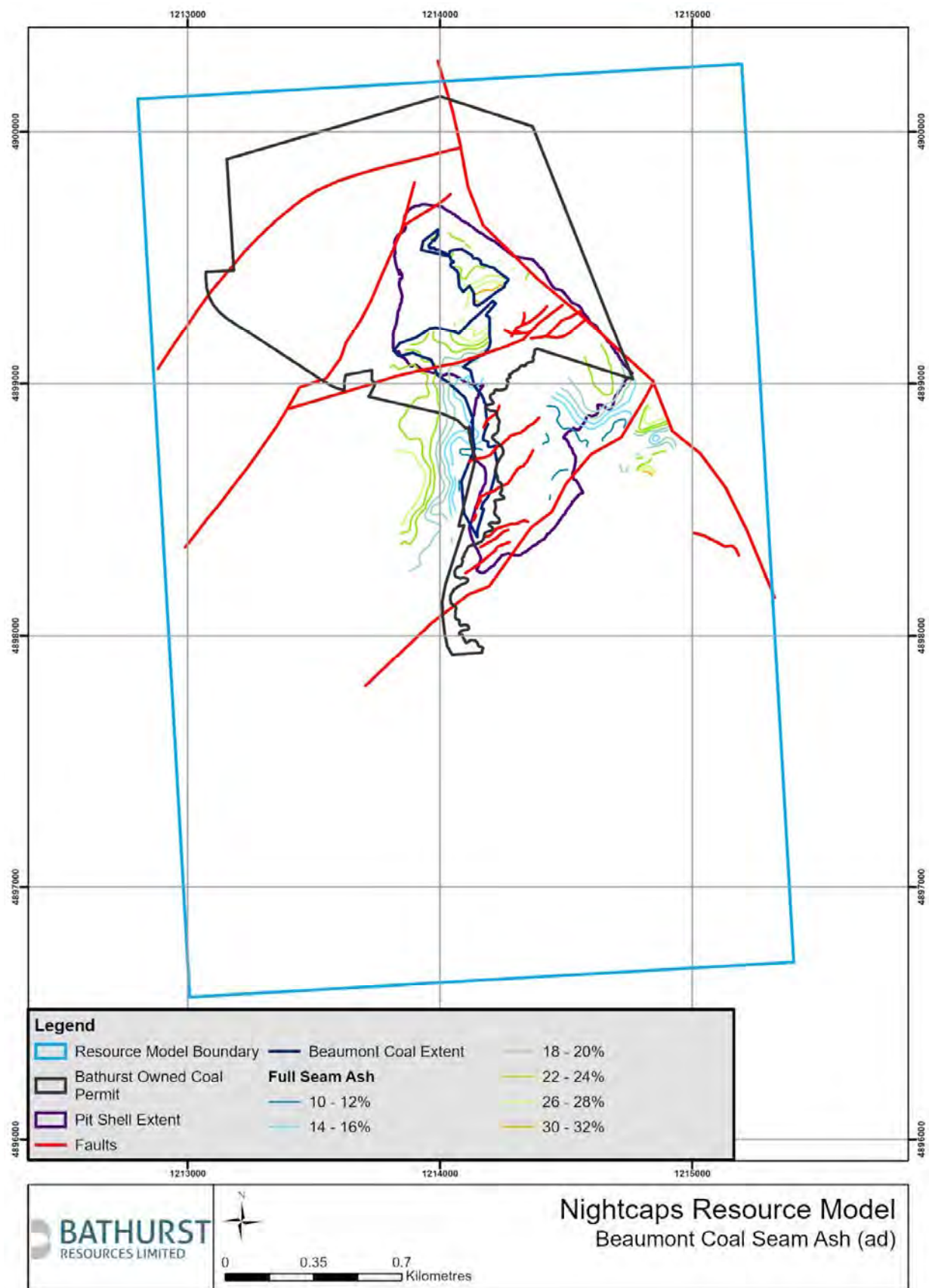
Figure 16: Beaumont Formation full seam ash isopachs
