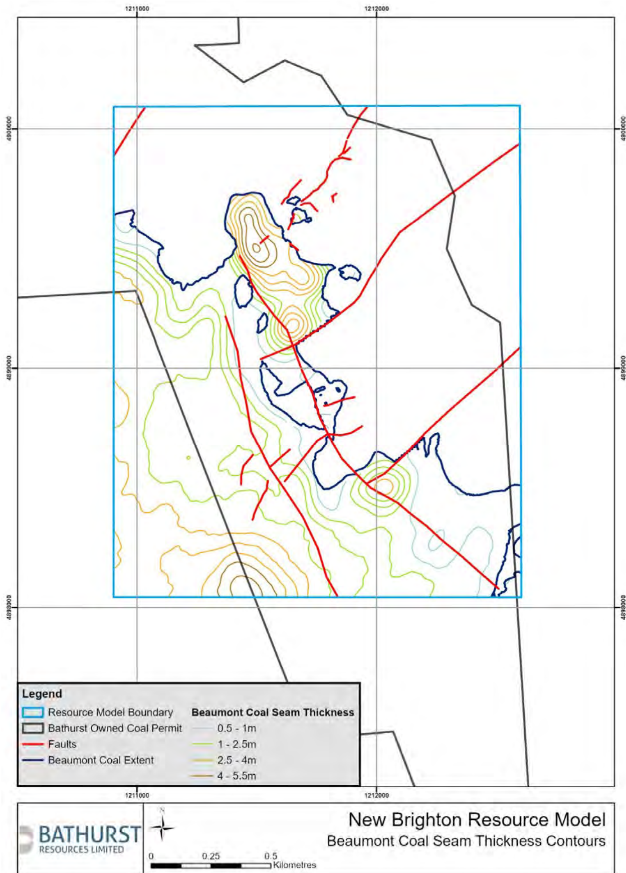
Figure 6: Beaumont Formation full seam cumulative thickness isopachs
