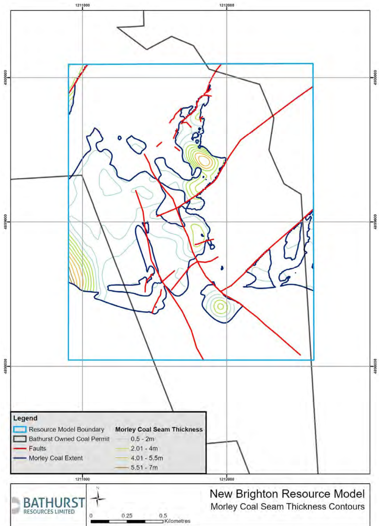
Figure 10: Morley Formation full seam cumulative coal thickness isopachs
