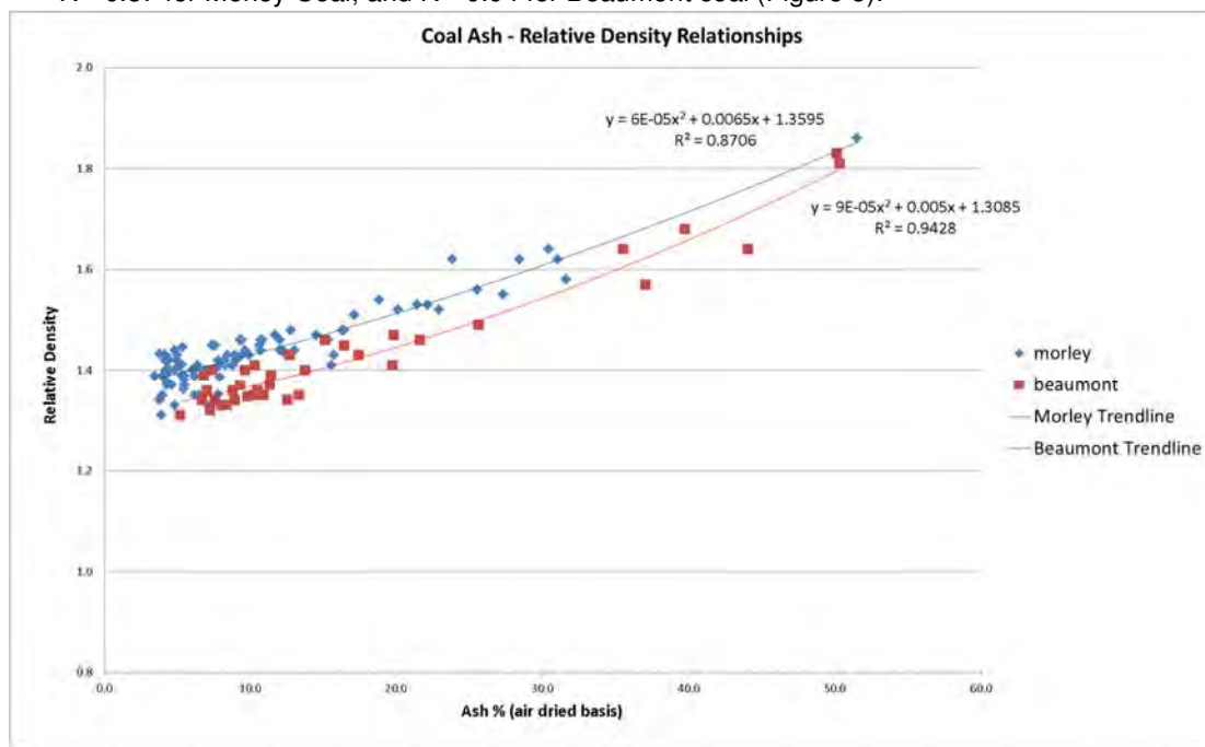
Figure 5: Graph showing Ash (adb) - Relative Density (adb) relationship for both Morley and Beaumont coal
