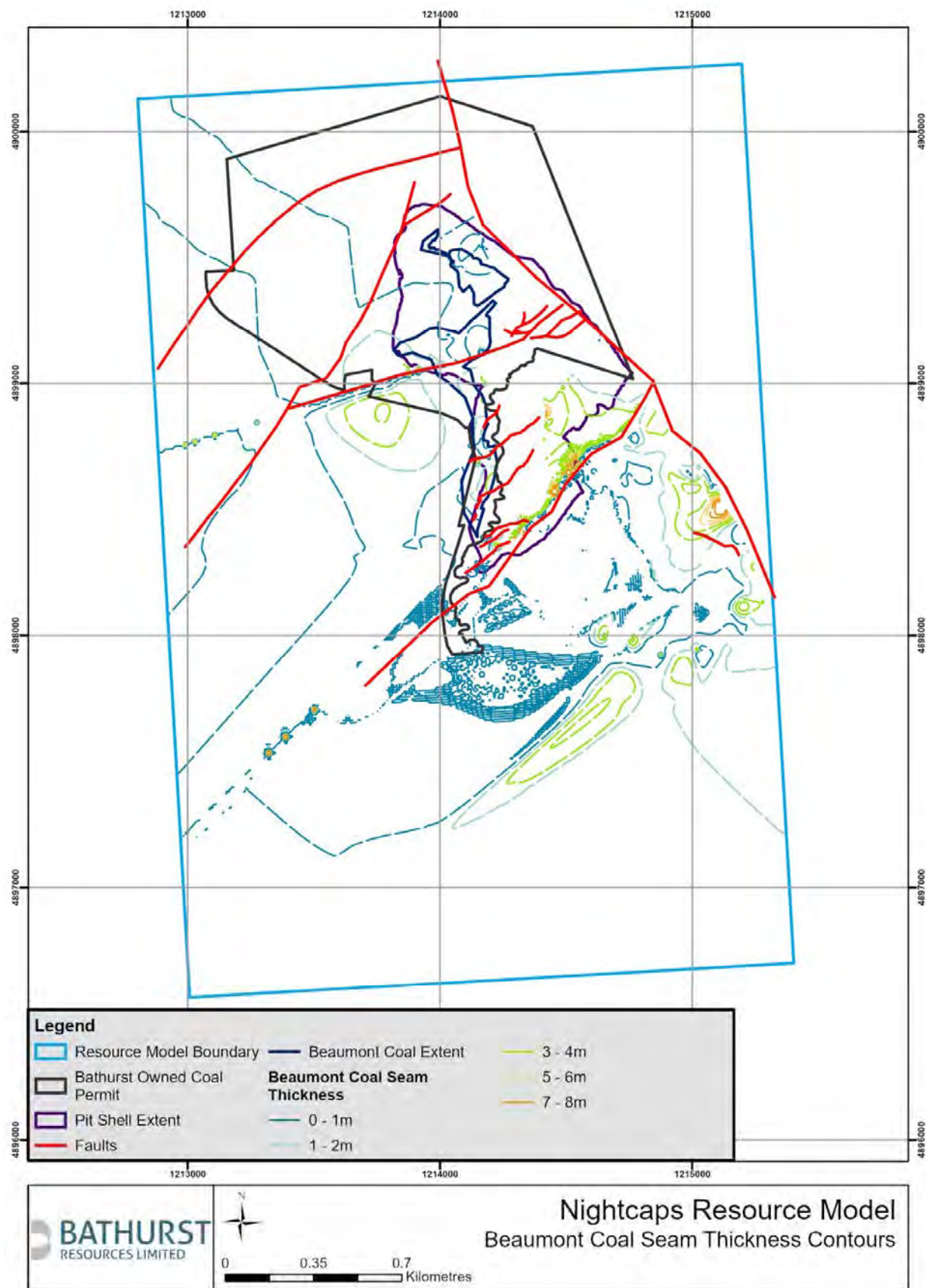
Figure 15: Beaumont Formation full seam cumulative thickness isopachs
