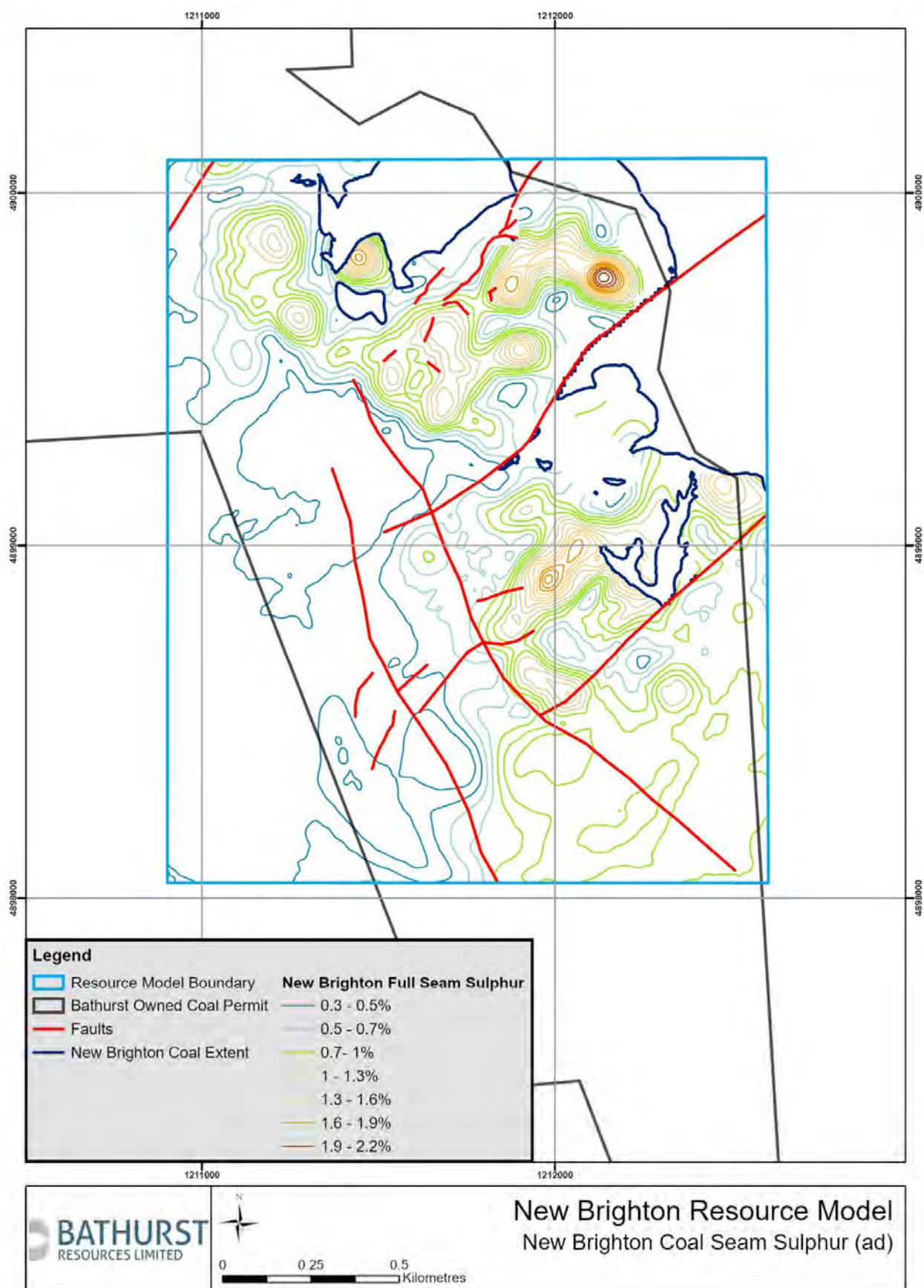
Figure 16: New Brighton Formation full seam sulphur isopachs
