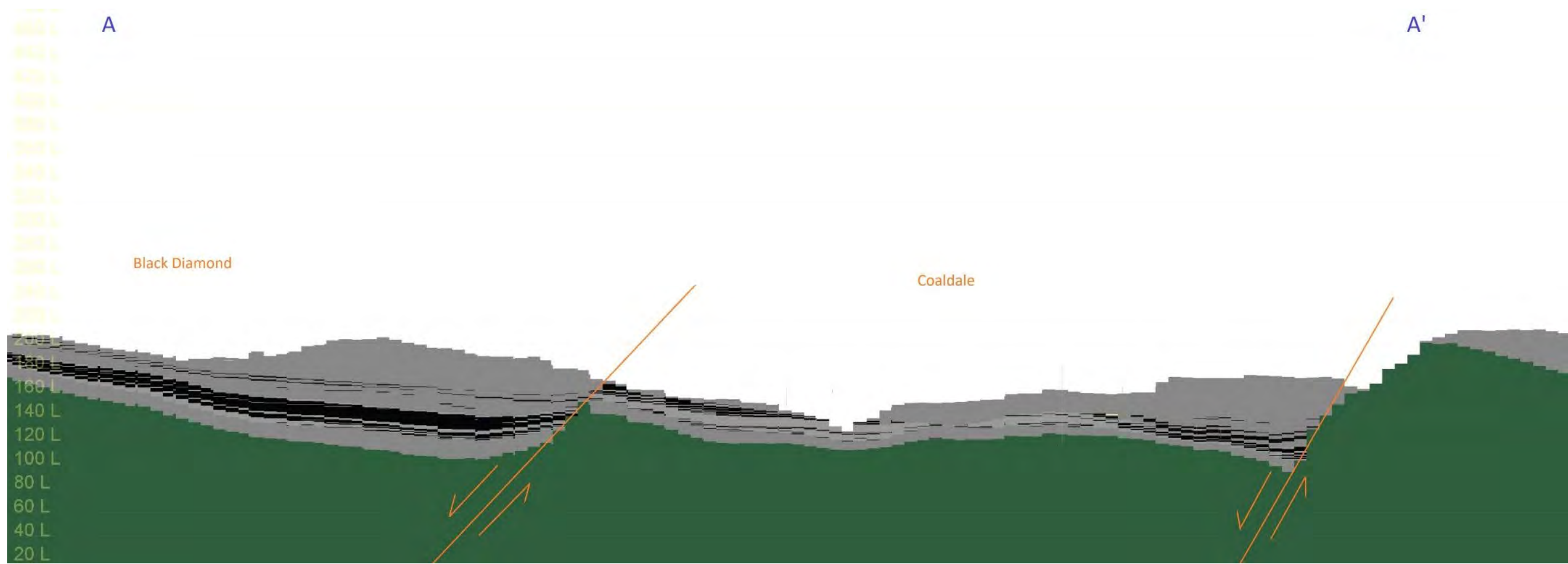
Figure 22: Section view through the deposit. The Black Diamond south fault and Trig E faults are shown
