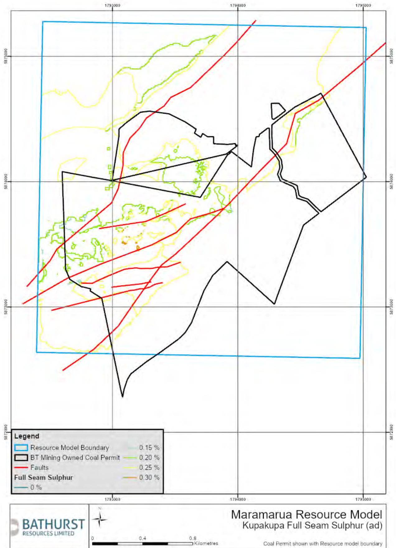
Figure 10: Plan showing full seam sulphur on an air-dried basis across the resource area
