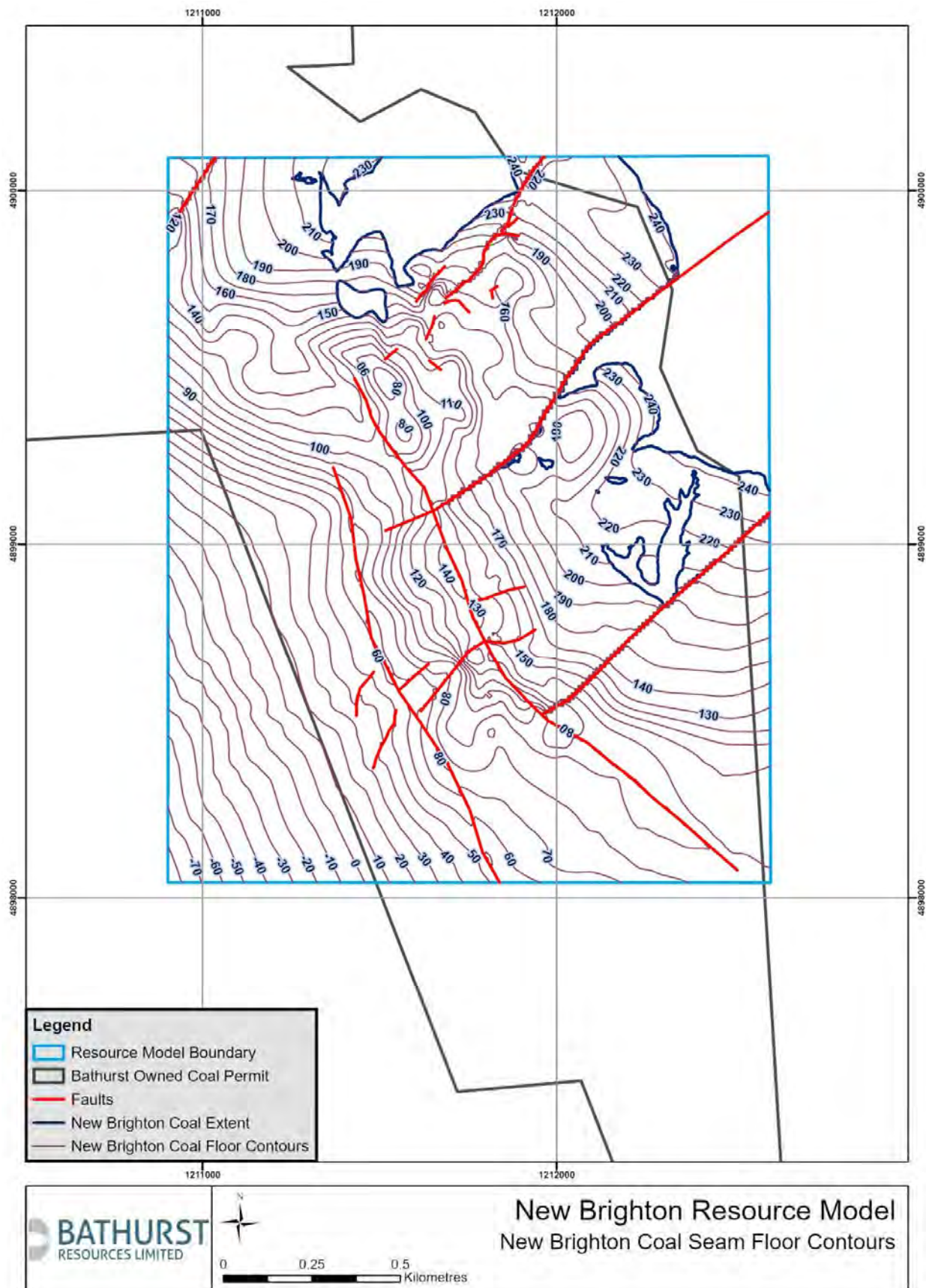
Figure 13: New Brighton (ON1 seam) coal floor contours
