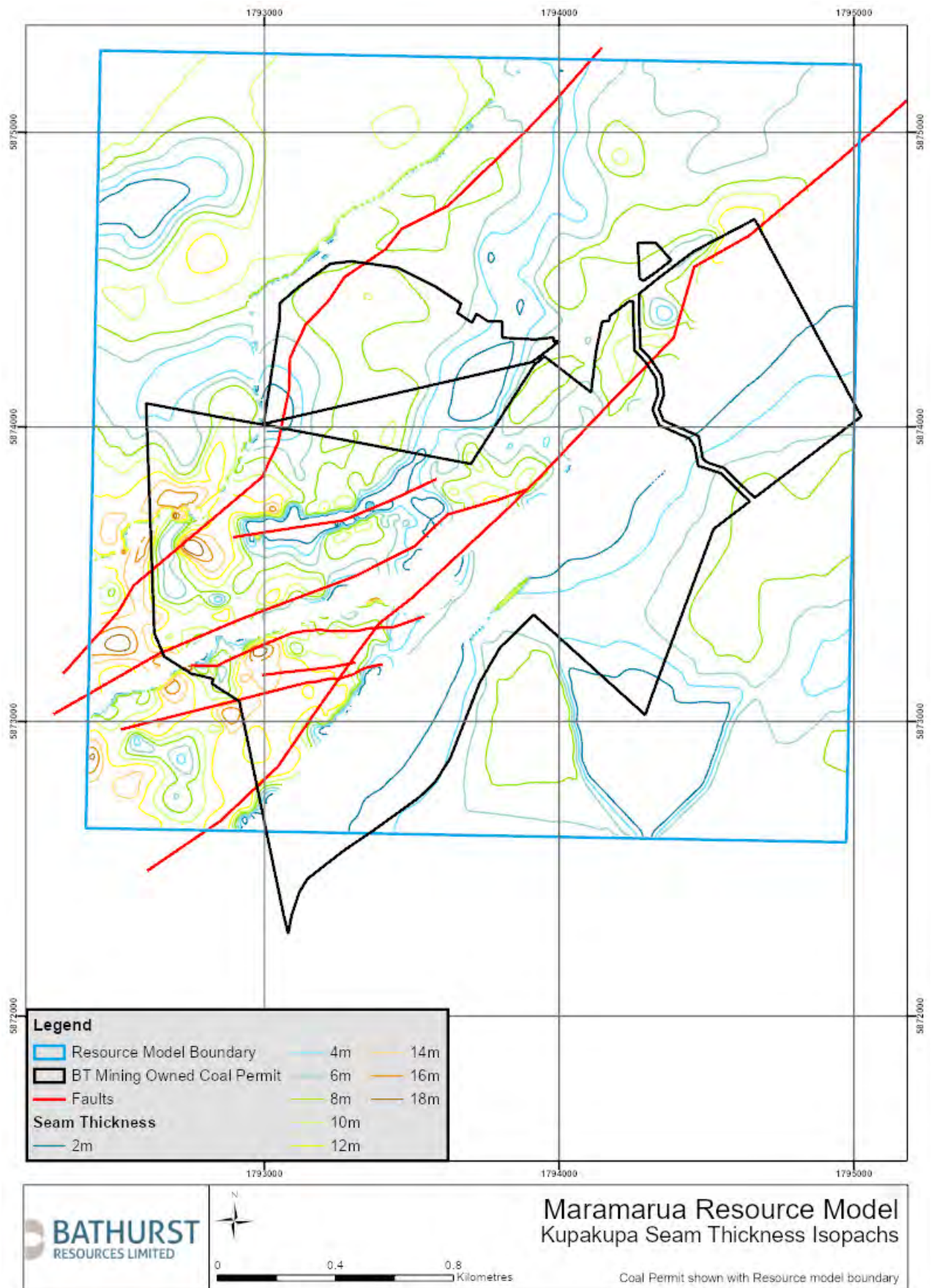
Figure 8: Plan showing full seam thickness contours over the model area
