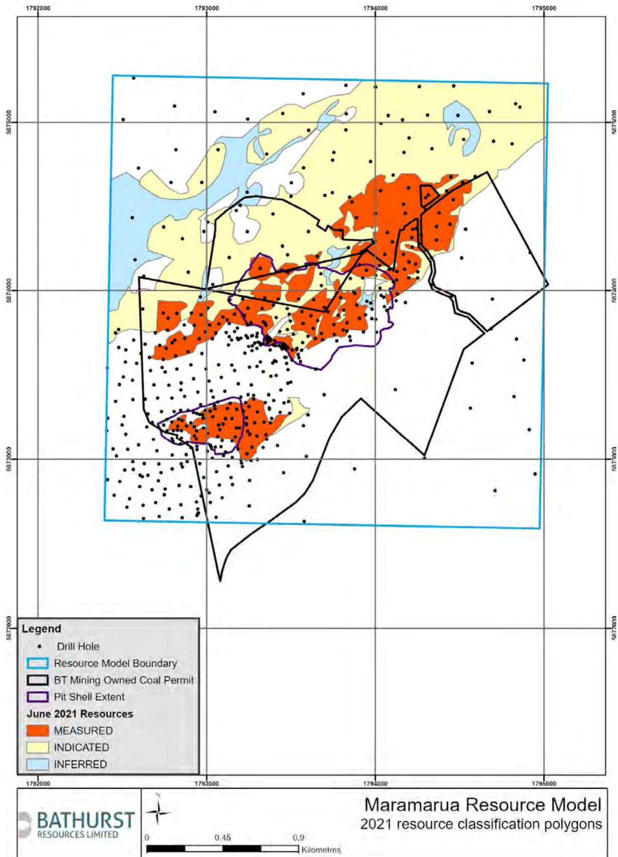
Figure 6: Plan showing the 2021 resource classification polygons
