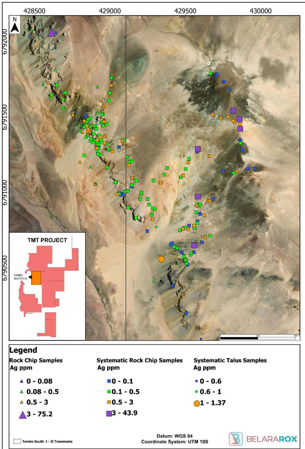
Figure 15: Silver results for rock and colluvium/talus samples from the Tambo South target. The isolated anomalous values in the northeastern part of the target are associated with rock float samples of silicified hydrothermal breccia.
