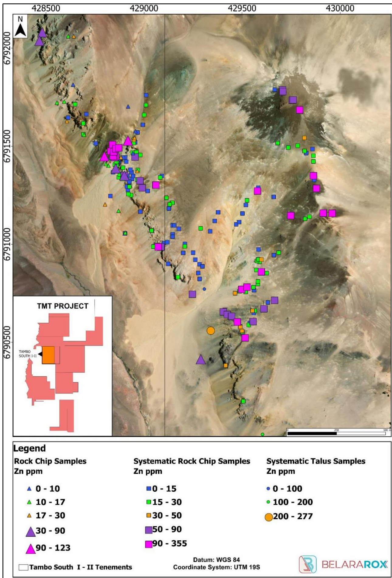
Figure 16: Map showing zinc (Zn ppm) in samples at the Tambo South target. The increased values to the east are consistent with metals deposition in the lower-temperature, peripheral portions of a porphyry system. The elevated Zn values in the more prospective northwestern area are inferred to indicate potential telescoping/overprinting of the porphyry centre by a lower-temperature (epithermal) event.
