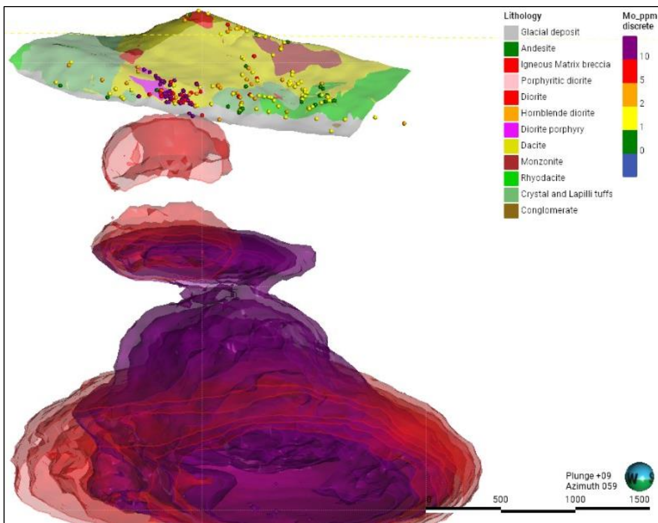
Figure 5: NW-SE longitudinal section (looking downwards 9° towards the east) showing Cohen (purple) and Halley (red) models generated from surface sampling at the Tambo South target. Both models suggest the presence of a porphyry-type system, with probabilities of \geq 0.14 starting at about 700m beneath surface.
