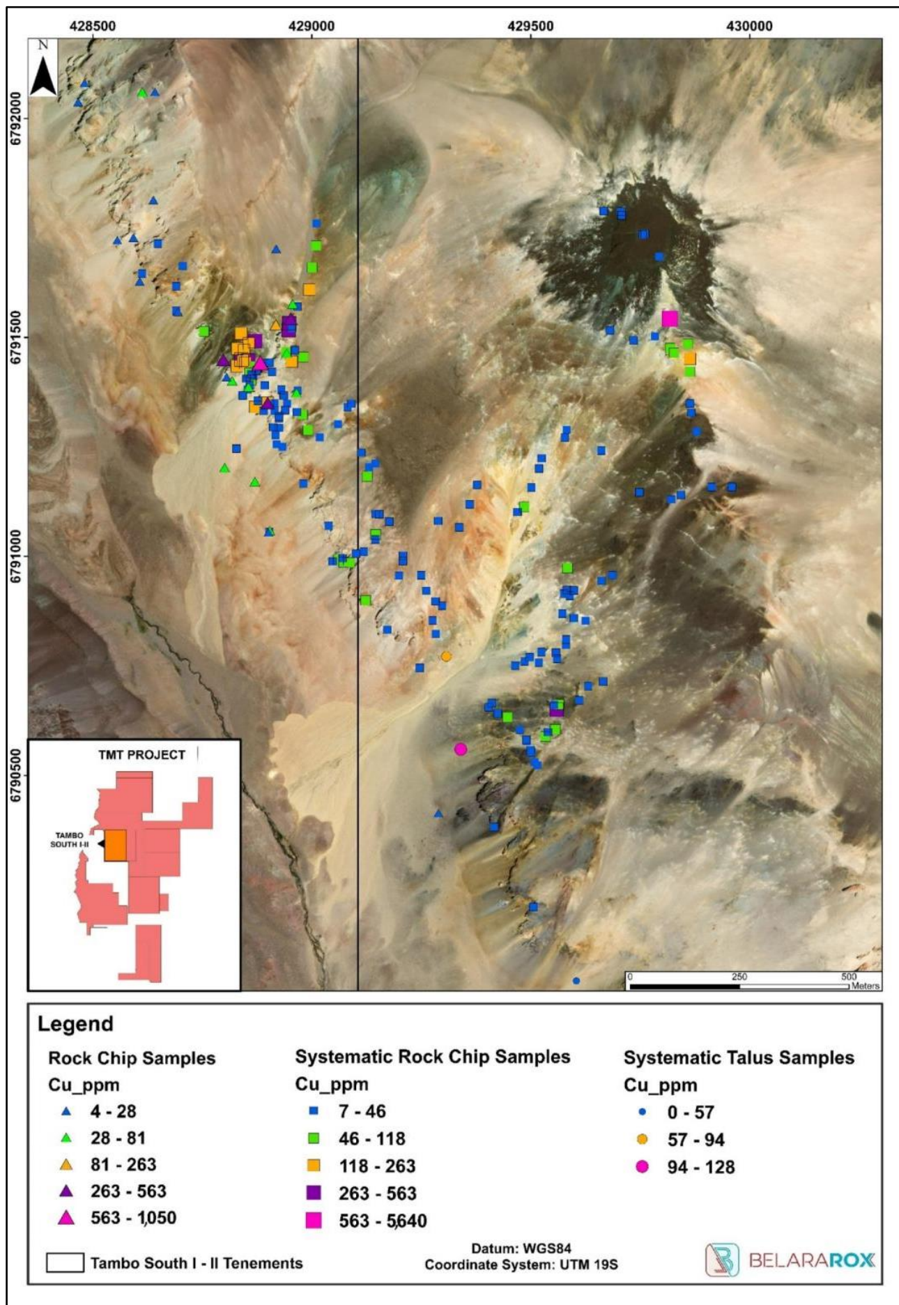
Figure 12: Copper results for rock and colluvium/talus samples from the Tambo South target, showing a concentration of higher values to the northwestern part of the system and isolated high values to the northeast.
