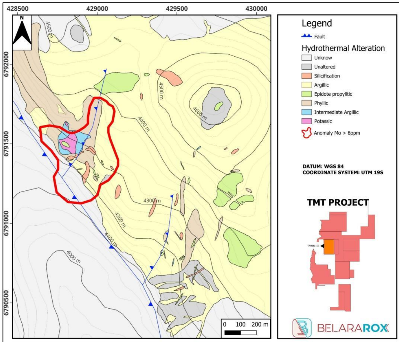
Figure 9: Interpretation of hydrothermal alteration in Tambo South outcrops. The expression of hydrothermal alteration covers an area of about 2 km by 1.3 km, remaining open to the east and south. The potassic (biotite-magnetite) and intermediate argillic (chlorite-sericite-clay) alteration zones extend approximately 230 meters by 200 meters. These zones contain 'M'-type magnetite veinlets and 'B'-type quartz veins that are flanked and overprinted by late-stage quartz veins. This zone of focused alteration and veining is interpreted as proximal to a porphyry centre that has been overprinted/telescoped by later-stage fluids. The surface molybdenum anomaly (Mo >6 ppm) coincides with the zones of potassic and intermediate argillic alteration and overprinting phyllic alteration near the intersection of major northwesterly- and northeasterly-trending faults.
