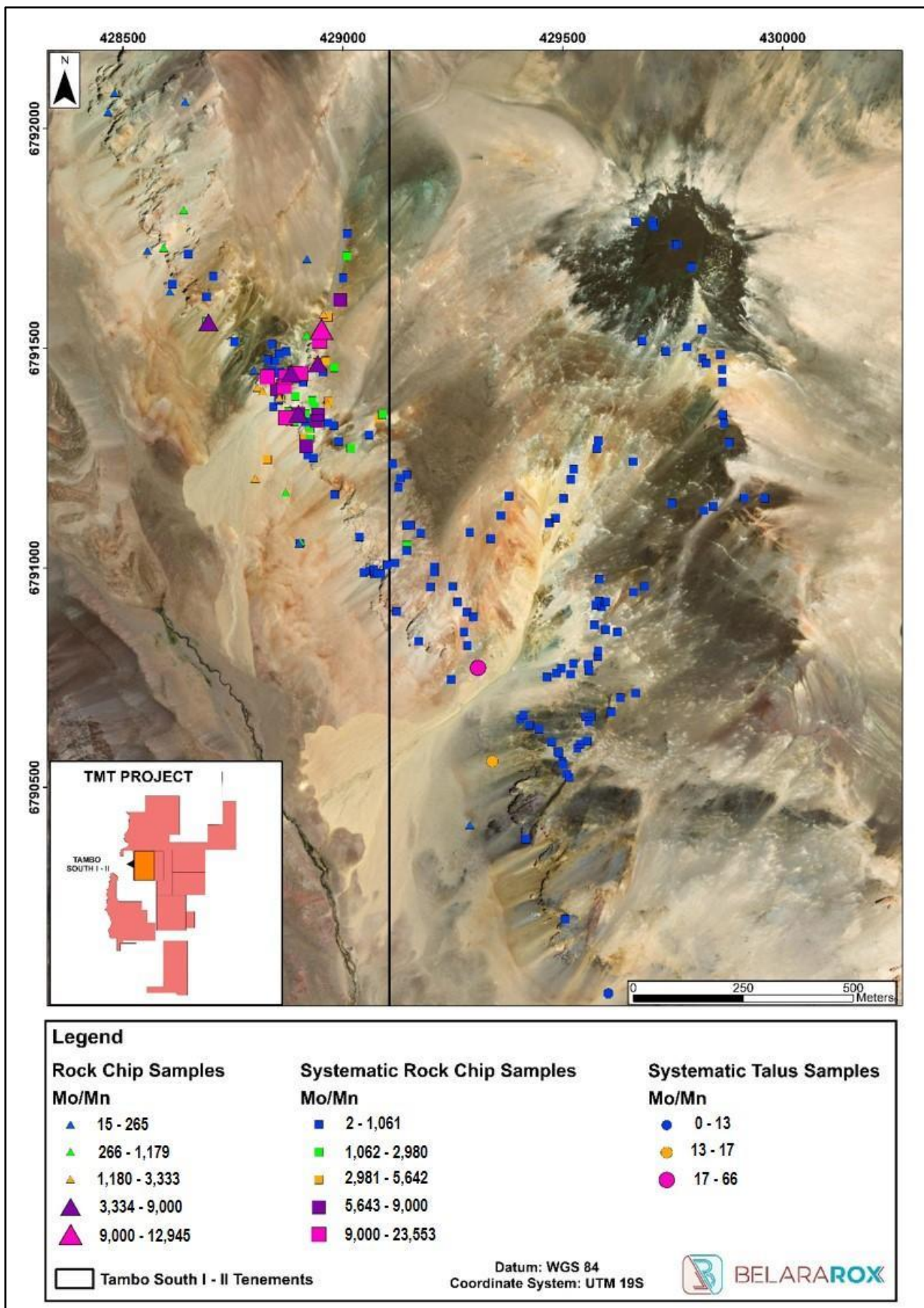
Figure 4: Geochemical results of molybdenum-manganese ratios of systematic rocks and talus samples from Tambo South. The highest Mo/Mn occurs in the northwestern part of the target, which is inferred to indicate proximity to a centre of porphyry-style mineralisation.
