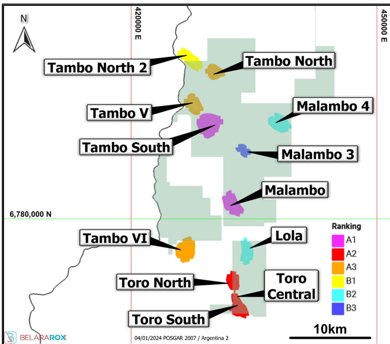
Figure 10: Twelve (12) prospective targets for hydrothermal alteration associated with porphyry mineralisation and/or epithermal mineral systems have been delineated in the TMT project, based on the study of satellite-deduced hydrothermal alteration [Modified from (Garwin, 2023)]
