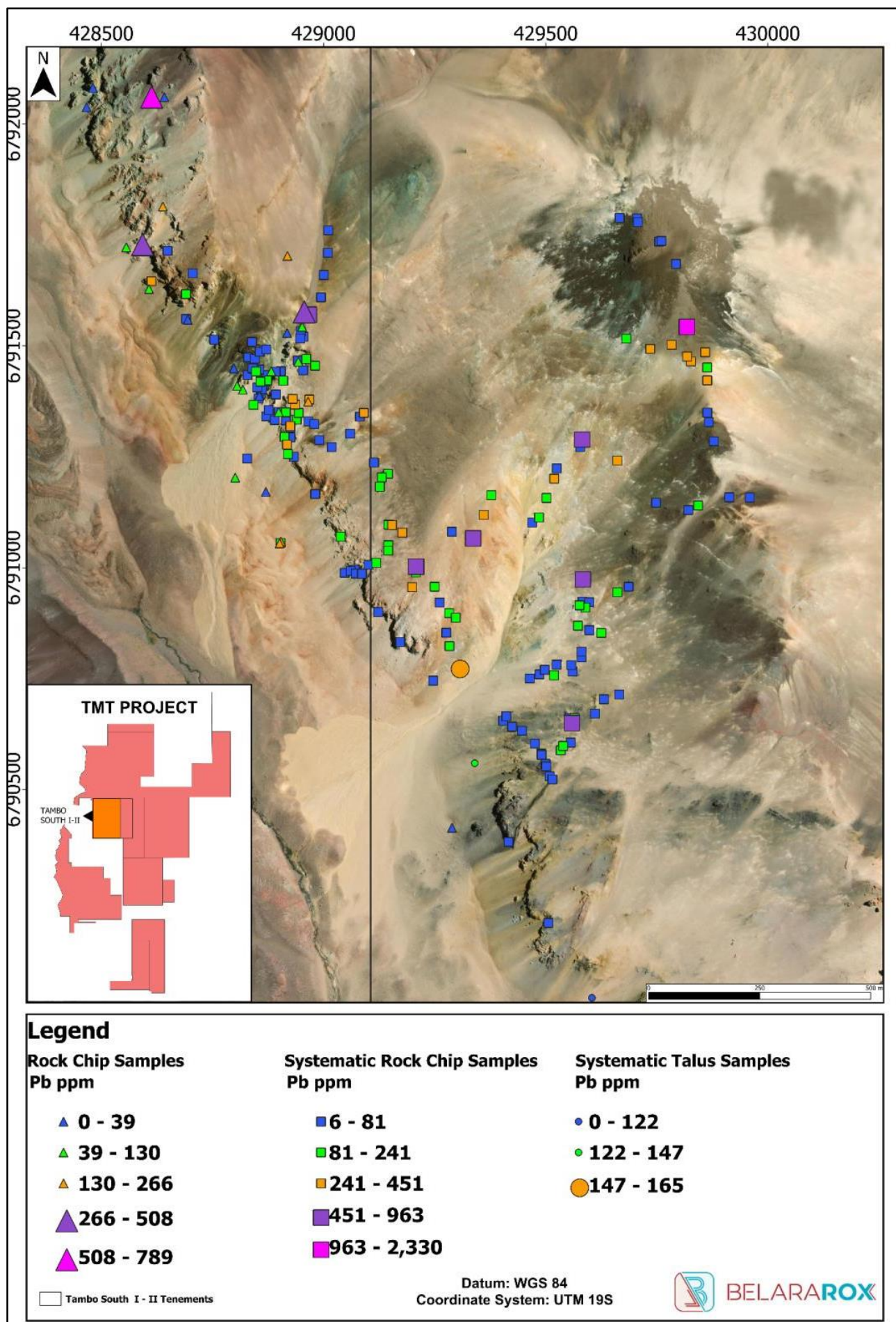
Figure 17: Map of lead (Pb ppm) results in samples at the Tambo South target. The elevated Pb values to the north, east and south of the Cu-Mo anomaly (c.f. Figures 12 and 13) are consistent with the deposition of Pb-bearing minerals in the lower-temperature, peripheral portions of a porphyry system.
