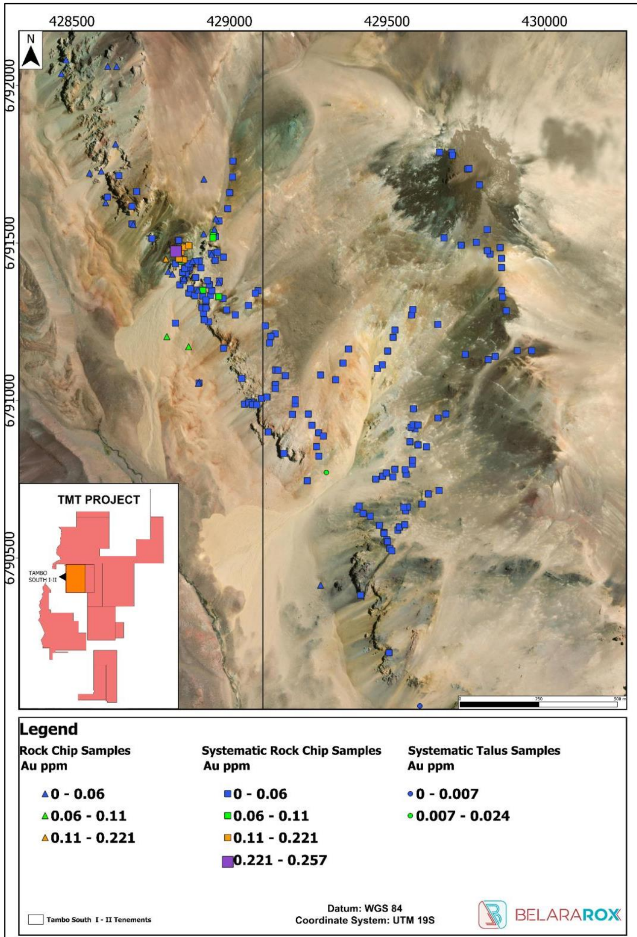
Figure 14: Gold results for rock and colluvium/talus samples from the Tambo South target. The best results to date occur in the northwest, which supports the anomalous Cu-Mo results.
