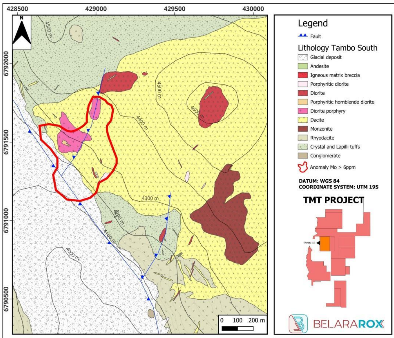
Figure 8: Tambo South interpretive surface geology. The Permo-Triassic rocks basement (conglomerate, tuffs and rhyodacite) are intruded by a Miocene dacite. The dacite is intruded by a prospective, porphyritic hornblende diorite (diorite porphyry – purple polygon) that hosts higher temperature veins ('M'- and 'B'-type), as well as potassic and intermediate argillic alteration. Subsequently, emplaced hydrothermal breccias (strong silicification) and late-stage intrusions of diorite and andesite traverse the entire sequence and are interpreted as post-mineralisation. The area is characterised by a complex fault system that juxtaposes the Permo-Triassic basement against the Miocene sequence and controls the emplacement and/or exhumation of prospective diorite porphyry and other intrusive stocks. The surface molybdenum anomaly ( \text{Mo} > 6 \text{ ppm} ) coincides with the distribution of the diorite porphyry near the intersection of major northwesterly- and northeasterly-trending faults.
