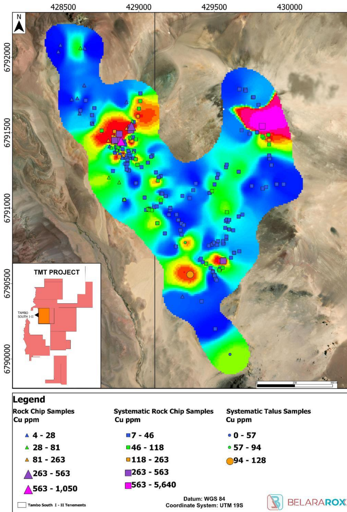
Figure 19: Heat map of Cu (ppm) in rock and colluvium/talus samples at the Tambo South target, showing a concentration of higher values in the northwestern portion of the target, coincident with the potassic alteration zone and molybdenum (Mo >6ppm) anomaly. The elevated values to the south and northeast of the target remain open and indicate an additional focus for exploration in the next field season.
