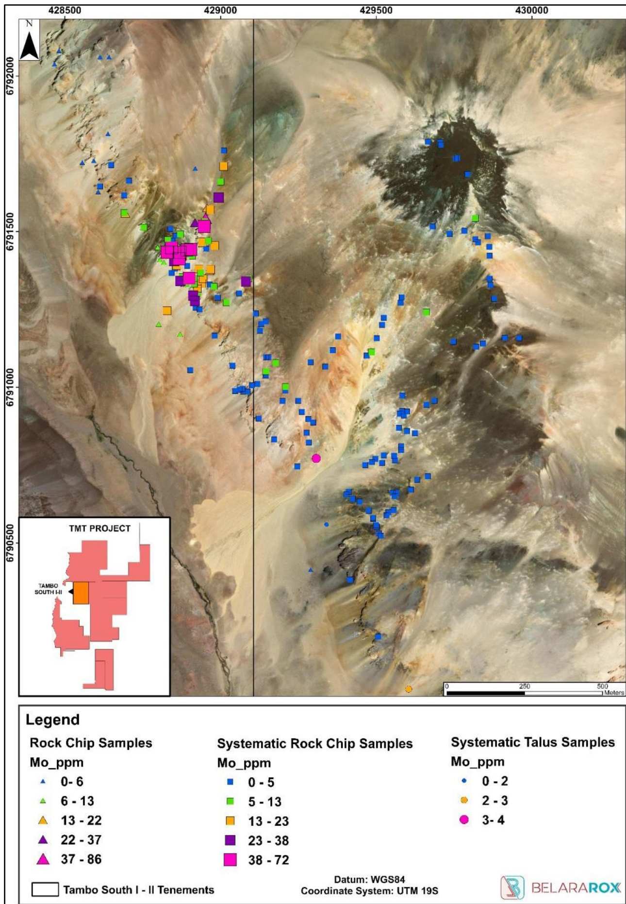
Figure 13: Molybdenum results for rock and colluvium/talus samples from the Tambo South target, showing a concentration of higher values to the northwest.
