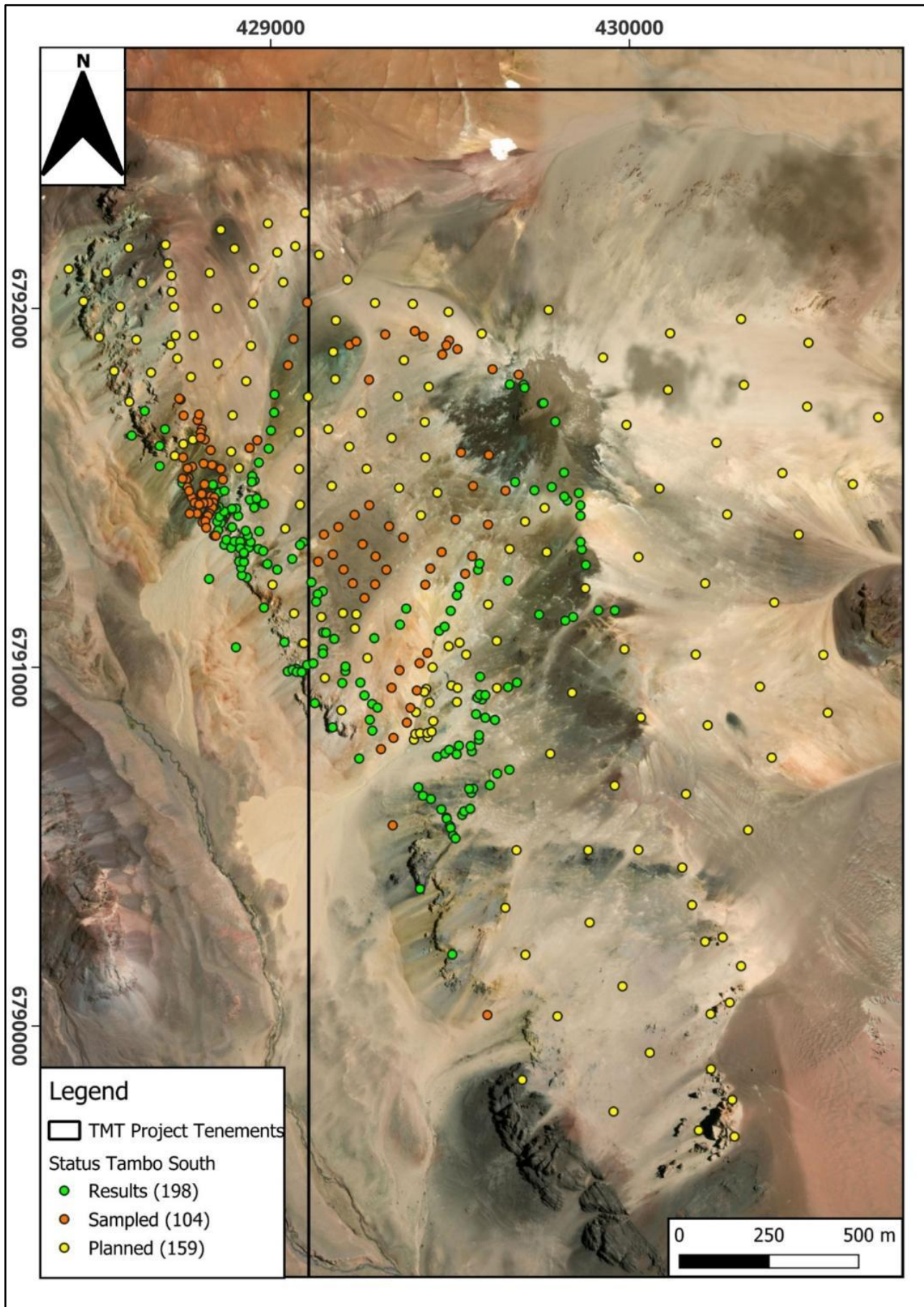
Figure 11: Map showing the distribution of existing and planned sample locations in the Tambo South target. A total of 198 rock and colluvium/talus samples have been analysed to date. An additional 104 samples will be sent to the lab in October 2024, and another 159 geochemical samples are planned to be collected to further assist in defining the porphyry system.
