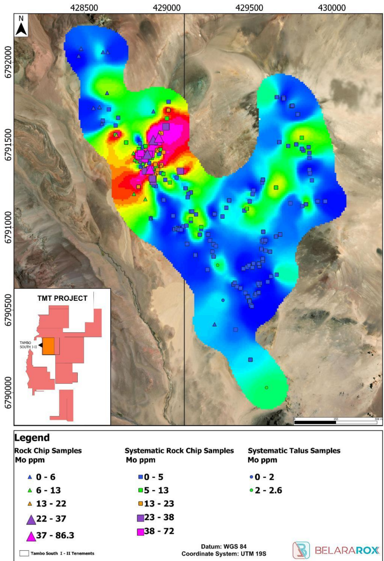
Figure 18: Heat map of Mo (ppm) in rock and colluvium/talus samples at the Tambo South target, showing a concentration of higher values in the northwestern portion of the target, which coincides with the zones of potassic and intermediate argillic alteration and overprinting phyllic alteration near the intersection of major northwesterly- and northeasterly-trending faults. (c.f. Figure 9).
