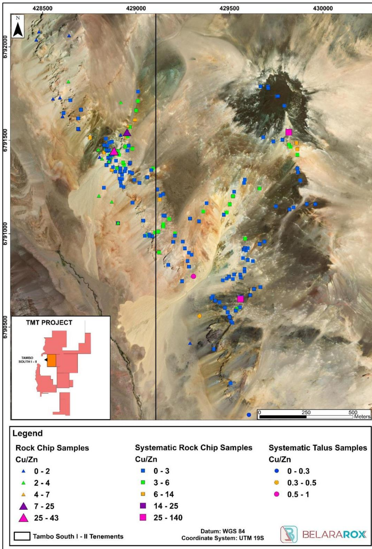
Figure 2: Geochemical results of copper-zinc ratios of systematic rocks and colluvium/talus samples from the Tambo South target. The highest values of Cu/Zn occur near the northwestern part of the Target within zones of potassic and intermediate argillic alteration, which is consistent with the higher temperatures of metal deposition that characterise the proximal portions of a porphyry system.
