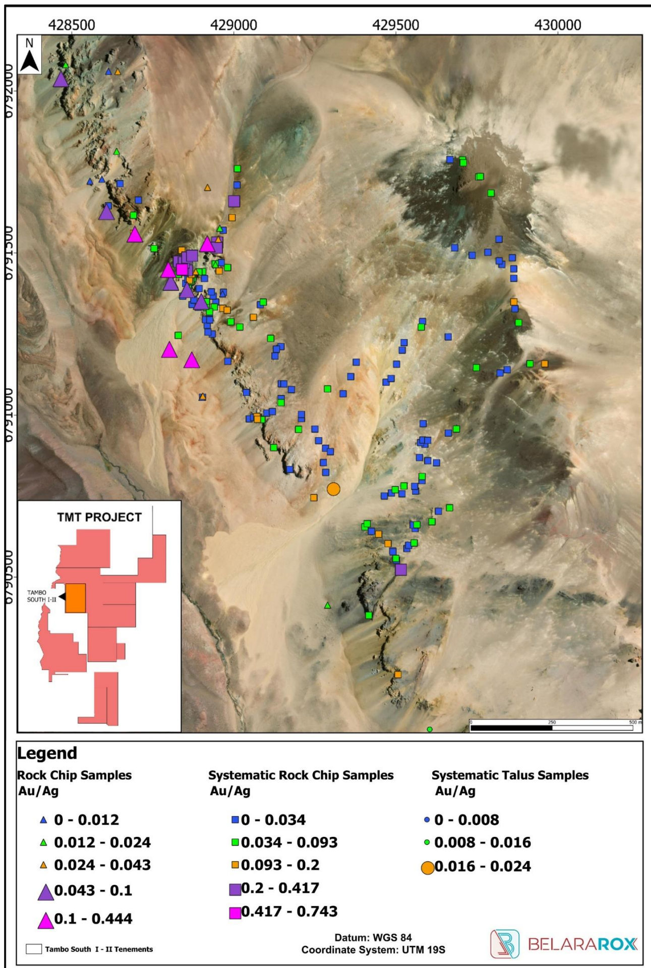
Figure 3: Gold- silver ratios for the geochemical results of systematic rocks and colluvium/talus in the Tambo South area. The highest Au/Ag values occur in the northwestern part of the target, which is inferred to indicate metal deposition at higher temperatures characteristic of increasing proximity to the porphyry centre.
