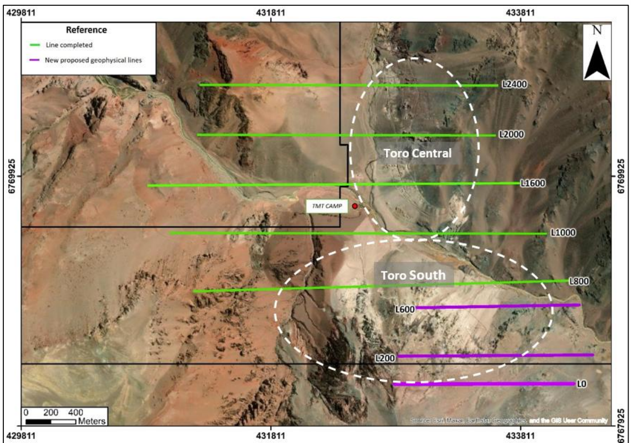
Figure 2: Completed survey lines (green lines) to date and proposed survey lines (purple lines) for the MT/IP geophysical survey over an area of approximately 2500m by 2500m covering the Toro South and Toro Central targets.
