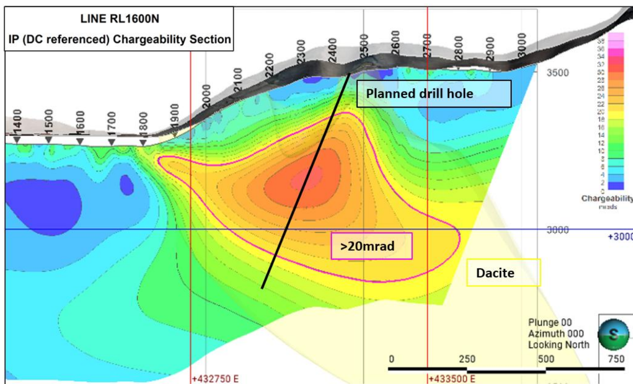
Figure 5: 2D IP chargeability section on line 1600 within BRX tenure (refer to Figure 2 for section location on plan view). Note the purple outline indicating a chargeability anomaly of >20mrad and its marked increase in size and intensity compared to line 2000.
