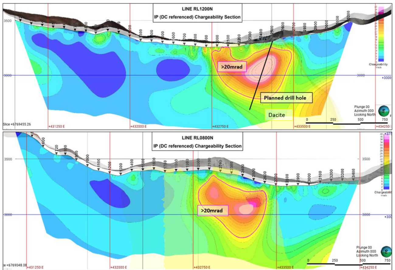
Figure 6: 2D IP chargeability section on line 1200 (top image) and 0800 (bottom image; refer to Figure 2 for section location on plan view). Note the purple outline indicating a chargeability anomaly of >20mrad and its marked increase in size and intensity compared to line 2000.
