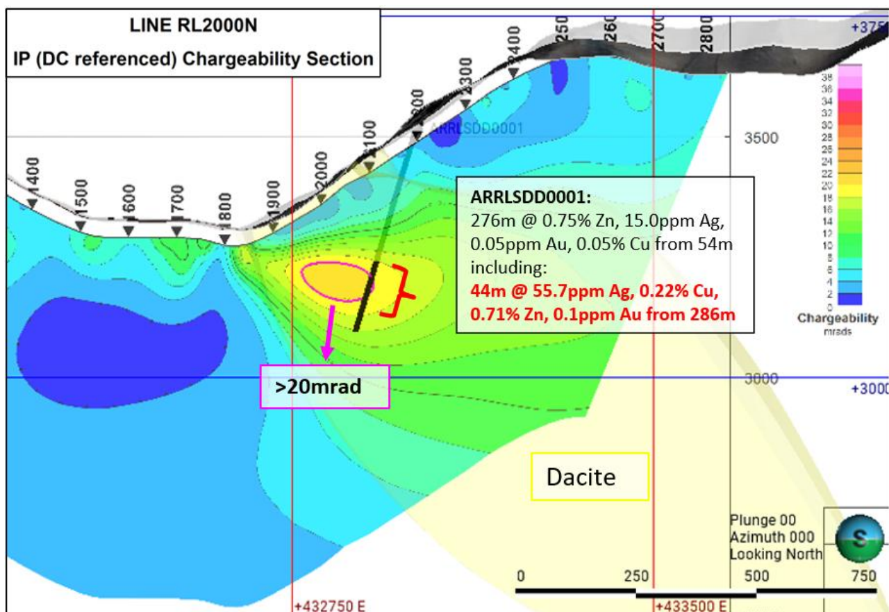
Figure 4: 2D IP chargeability section on line 2000 within BRX tenure (refer to Figure 2 for section location on plan view). Note the purple outline indicating a chargeability anomaly of >20mrad.
