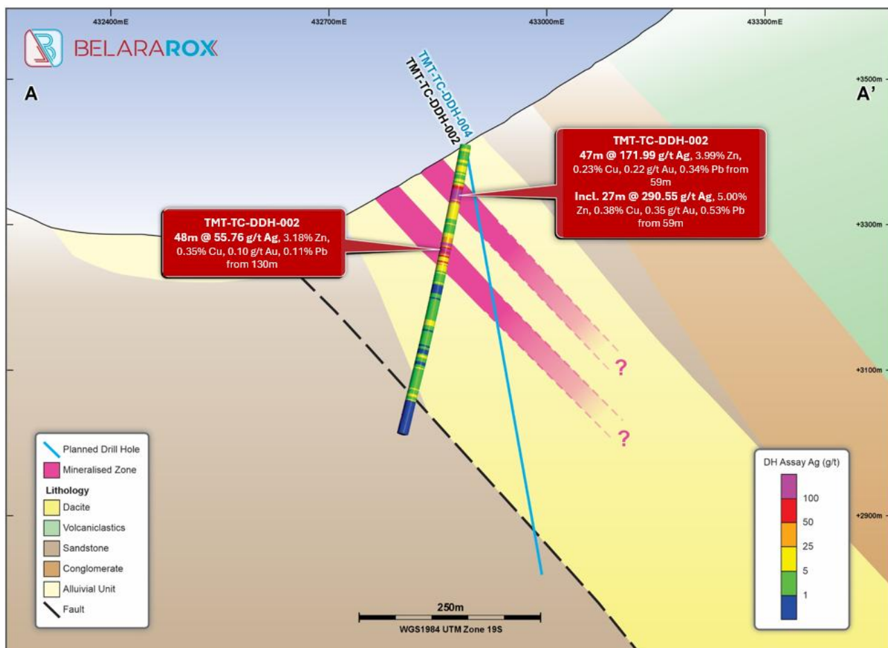
Figure 3: Cross-section looking north showing the results from TMT-TC-DDH-002 and the currently ongoing drill hole TMT-TC-DDH-004 targeting the down-dip extents of the mineralised zones.
