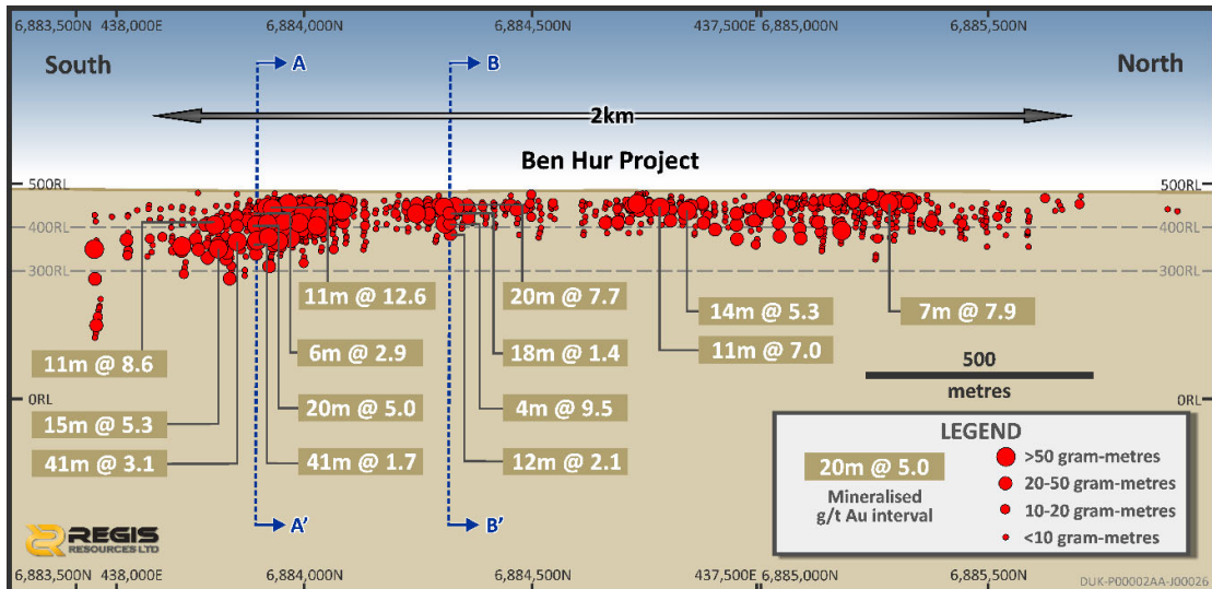
Figure 2: Ben Hur deposit long-section highlighting the better intercepts from within the resource
