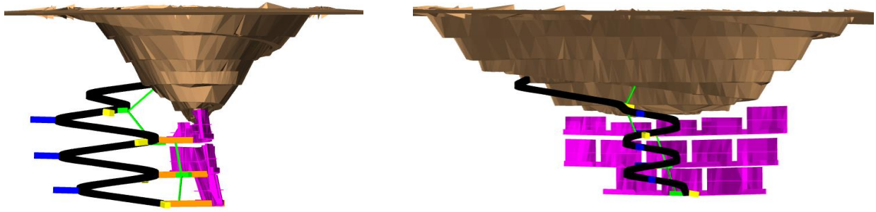
Figure 8 - Fish Underground Mine designs beneath existing open pit: Cross section looking north (left); long section looking east (right)
