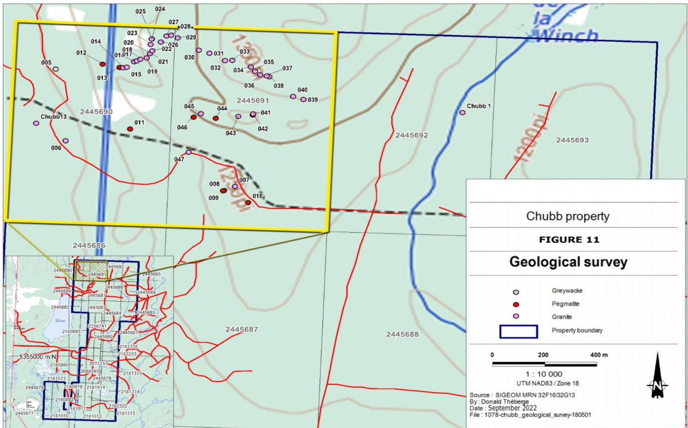
Figure 6: Mapping of Pegmatites in the NW sector of the Chubb Mineral Claims
