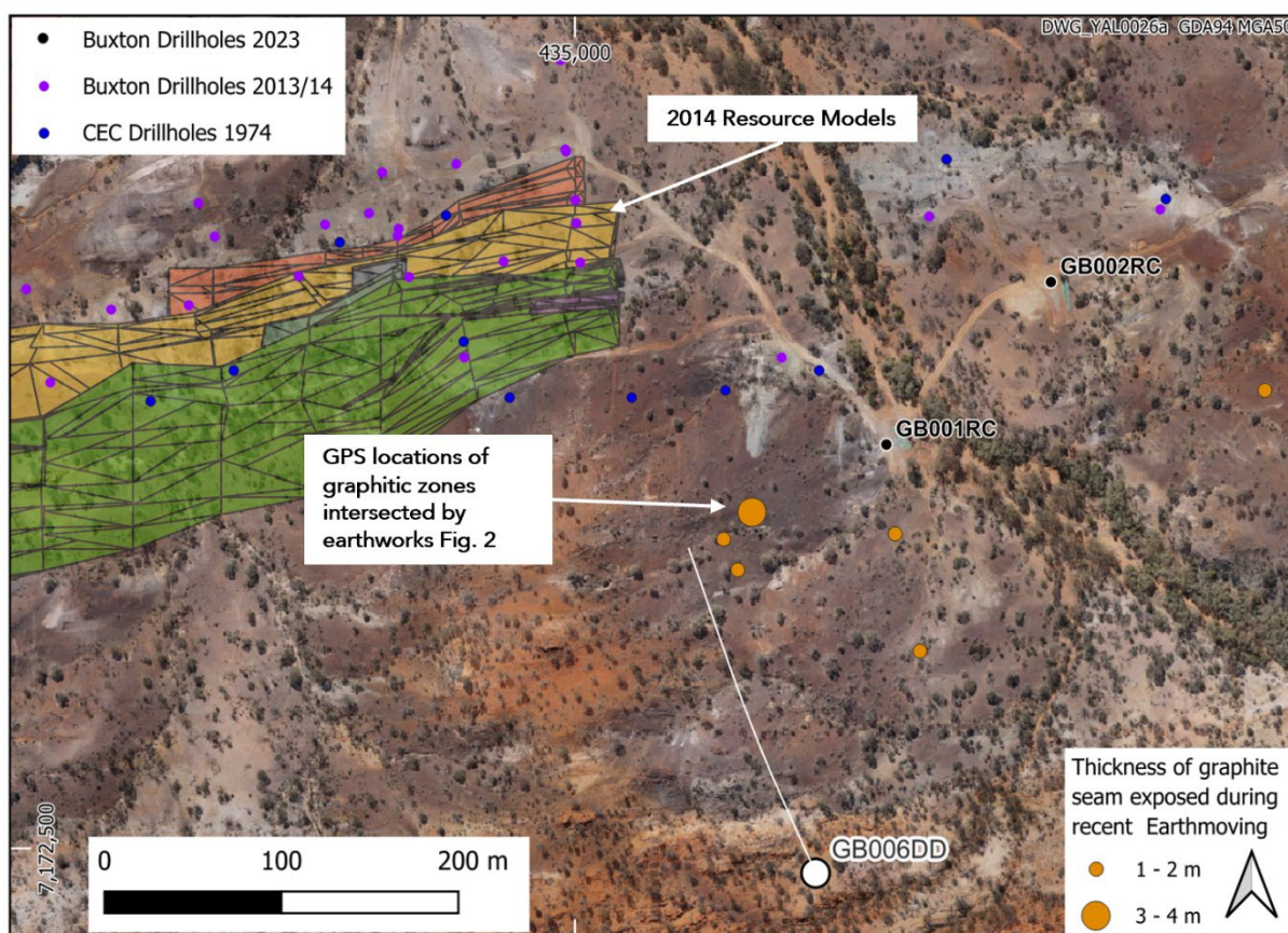
Figure 1: Current drill trace of GB006DD with the location of graphite seams intersected by earthworks (2014 Resource models of steeply South dipping graphitic lodes are projected to surface).
