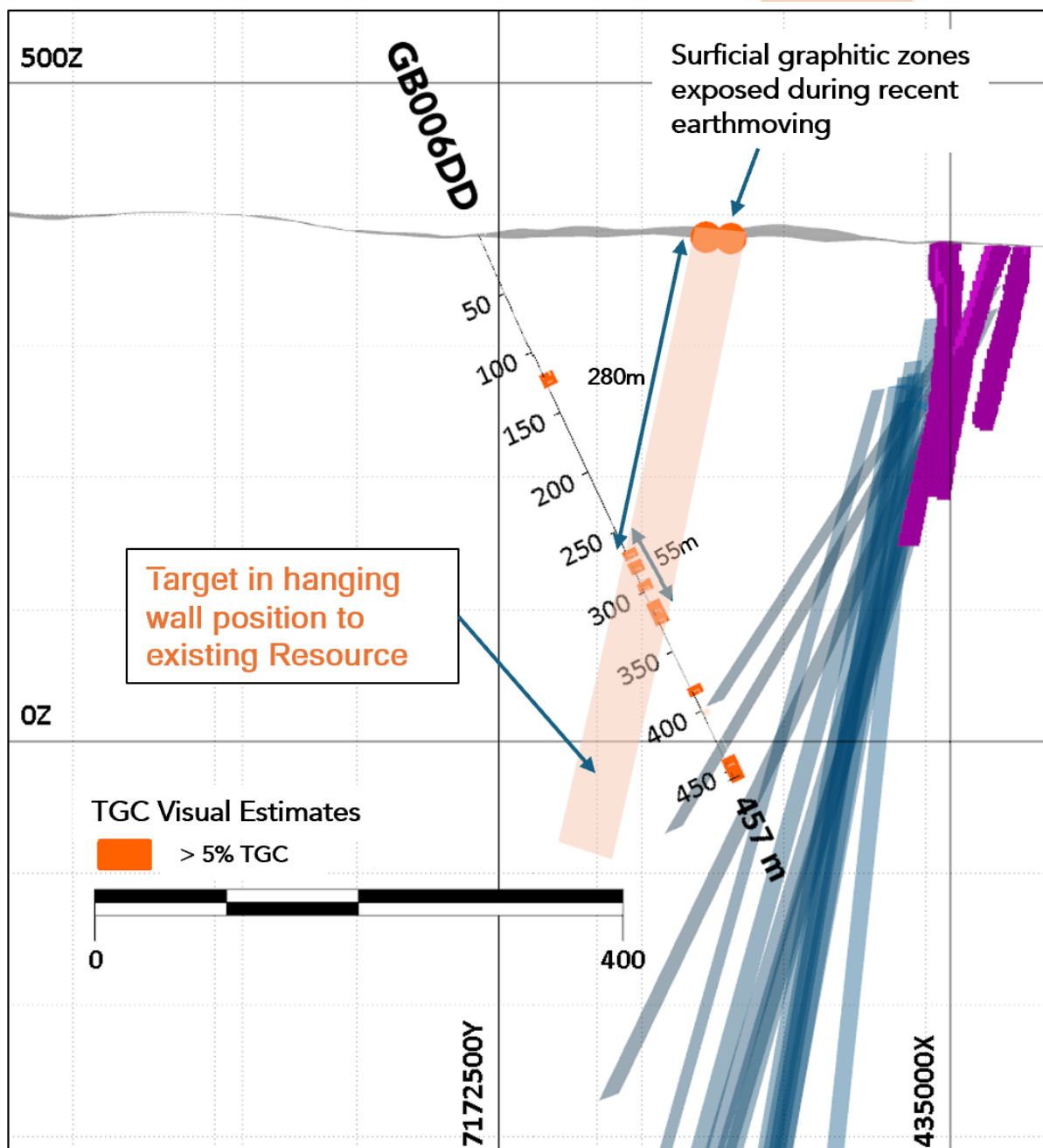
Figure 3: Cross section through deep diamond hole GB006DD (in progress) showing visual 2023 high power ground EM models and previous drilling.
