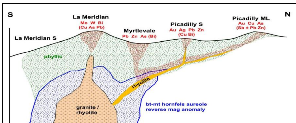
Figure 4:3 Schematic Model of Interpreted Intrusive Related mineral system
