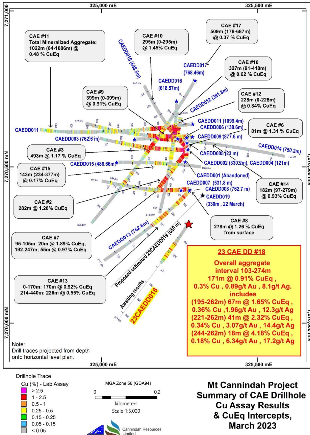
Fig 4. Plan view CAE Hole # 18 in relation to 2021-2023 CAE Drillholes Mt Cannindah. Downhole lab Cu plotted, CuEq intercepts annotated.
