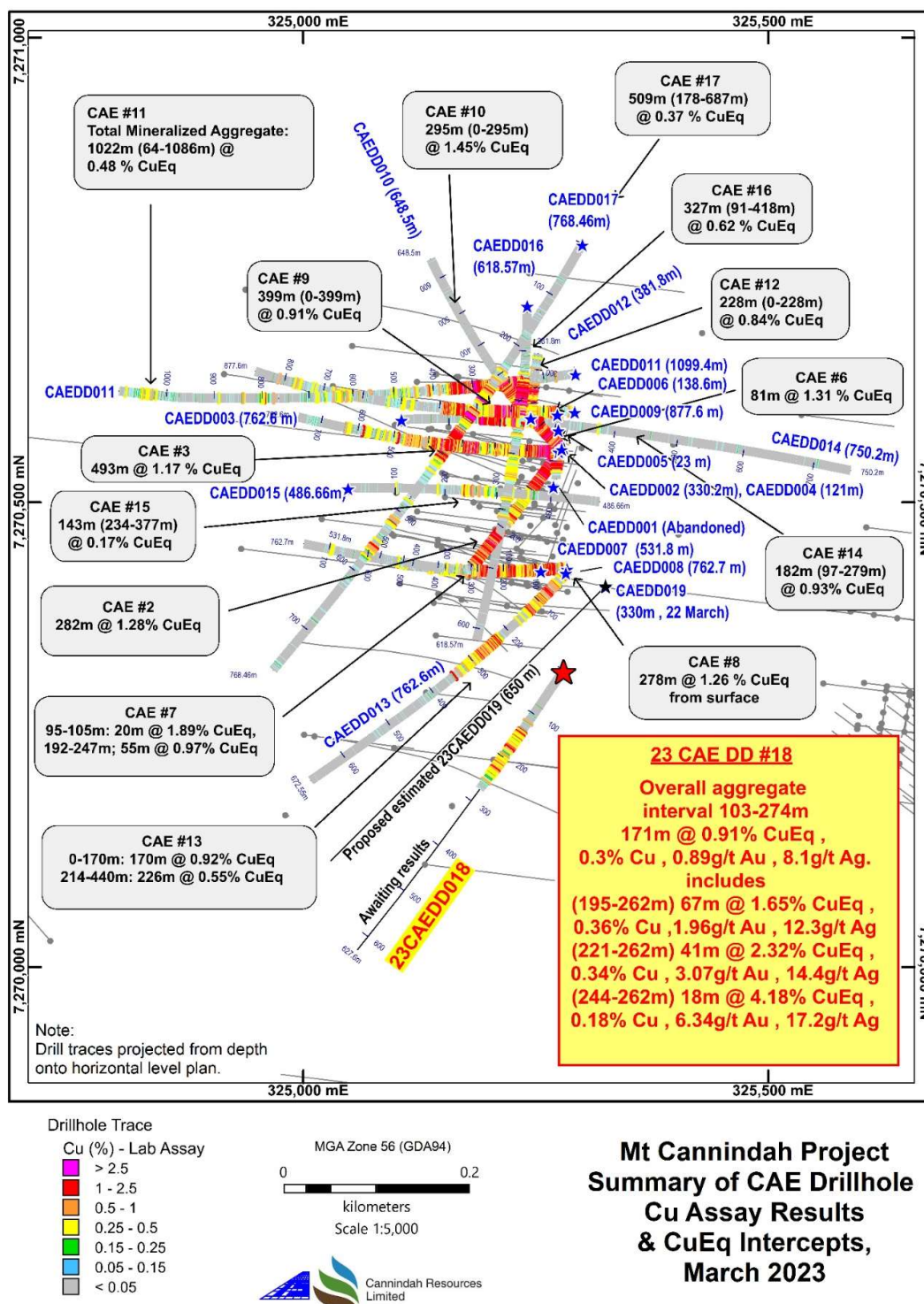
Fig App2.1 Plan view CAE Hole # 18 in relation to 2021-2023 CAE Drillholes and Historical holes at Mt Cannindah. Downhole lab Cu plotted, CuEq intercepts annotated.
