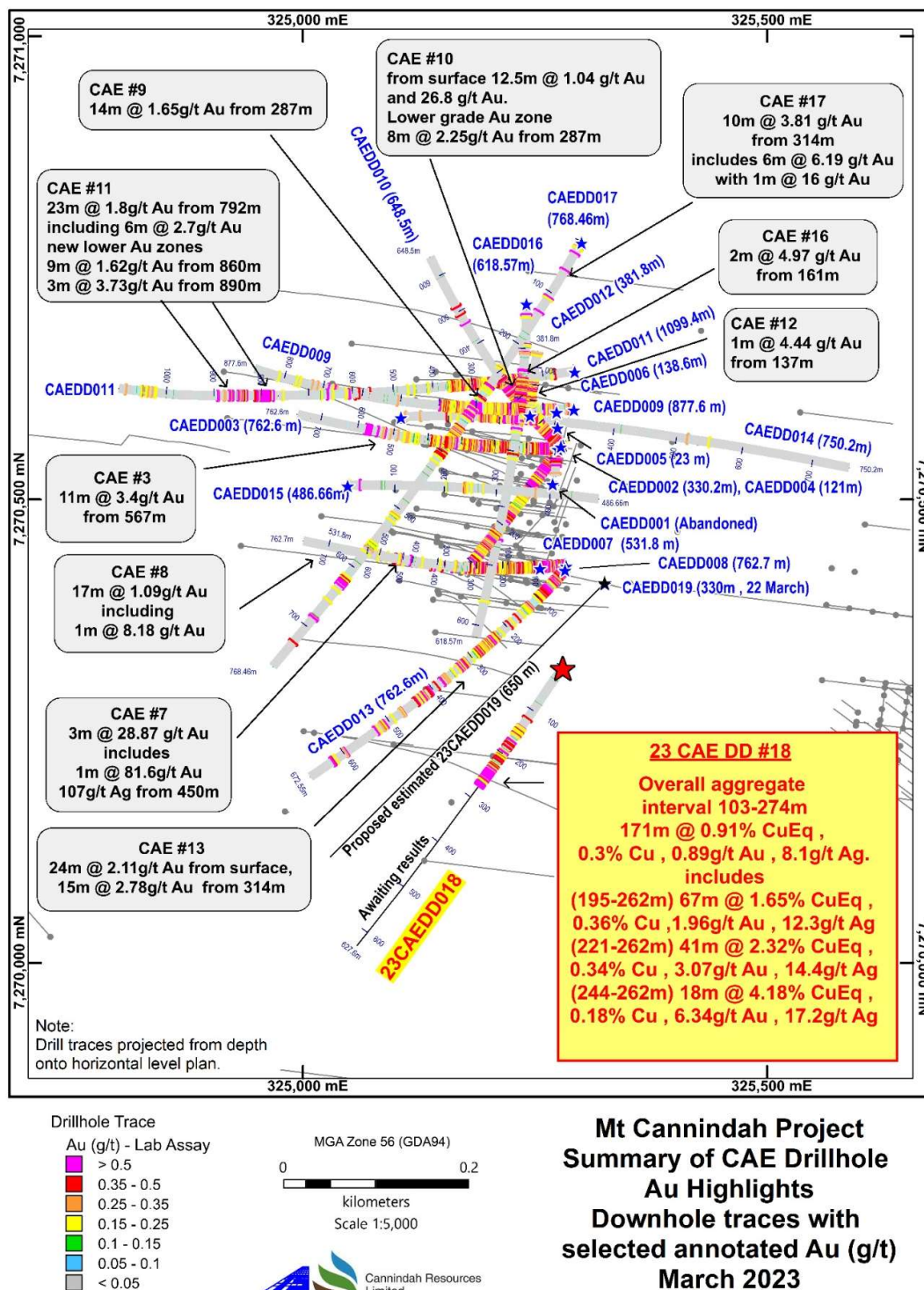
Fig App 2.2. Plan view CAE Hole # 18 in relation to 2021-2023 CAE Drillholes Mt Cannindah. Downhole lab Au plotted, Selected gold results annotated.
