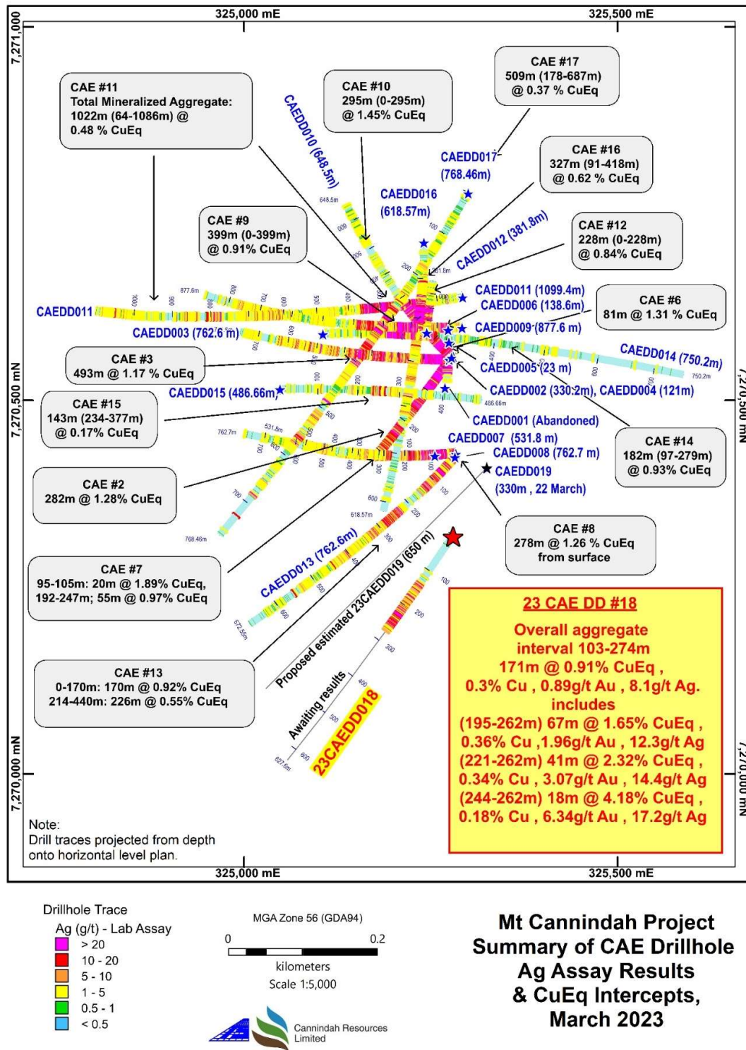
Fig 6 Plan view CAE Hole # 18 in relation to 2021-2023 CAE Drillholes Mt Cannindah. Downhole lab Ag plotted, CuEq intercepts annotated.
