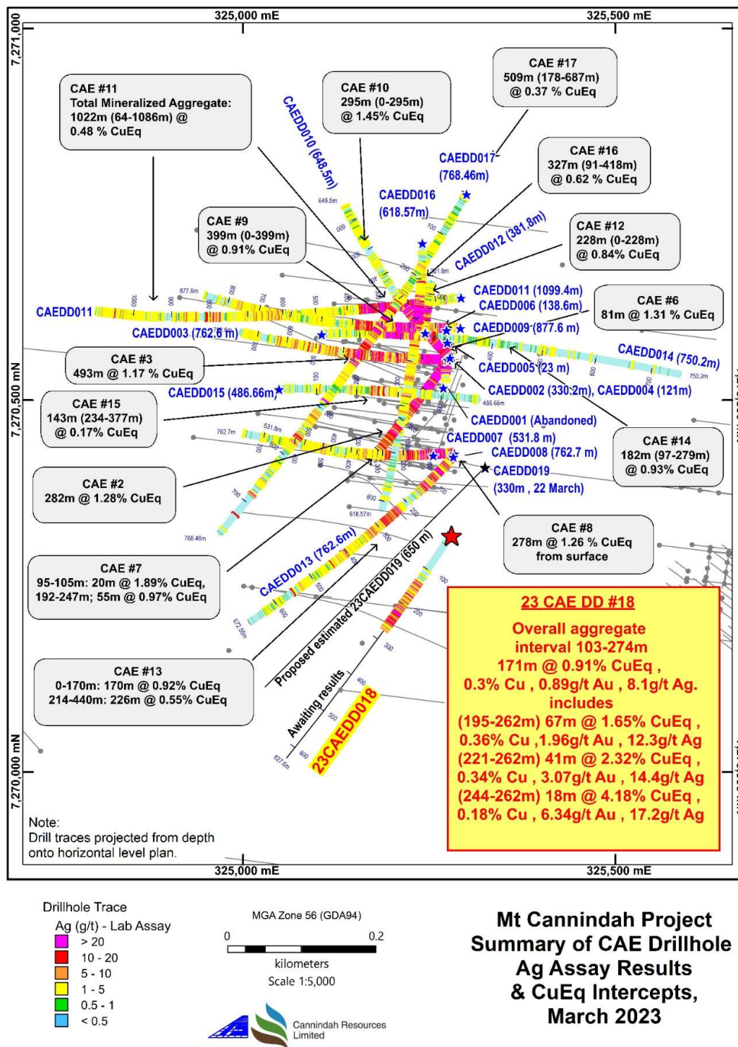
Fig App2.3. Plan view CAE Hole # 18 in relation to 2021-2023 CAE Drillholes Mt Cannindah. Downhole lab Ag plotted, CuEq intercepts annotated.
