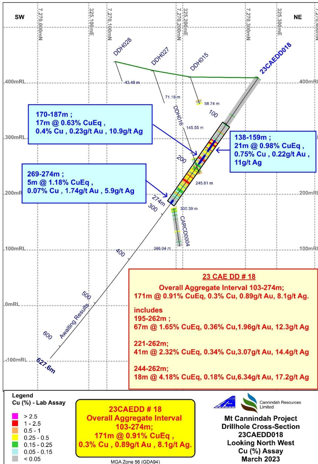
Fig 7. Cross section CAE Hole # 18 in relation to 2021-2023 CAE Drillholes and assayed historical holes at Mt Cannindah. Downhole lab Cu plotted, CuEq intercepts annotated.
