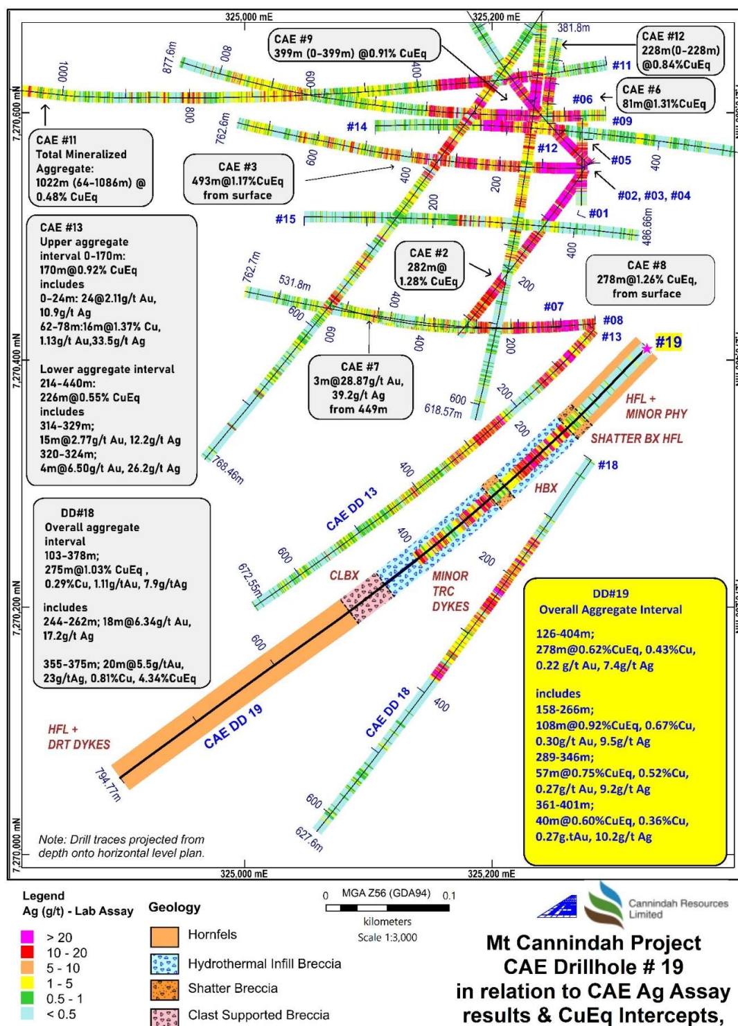
Fig 6. Plan view CAE Hole # 19 simplified geology in relation to 2021-2023 CAE Drillholes Mt Cannindah. Downhole lab Ag plotted, CuEq intercepts annotated for previous CAE holes.
