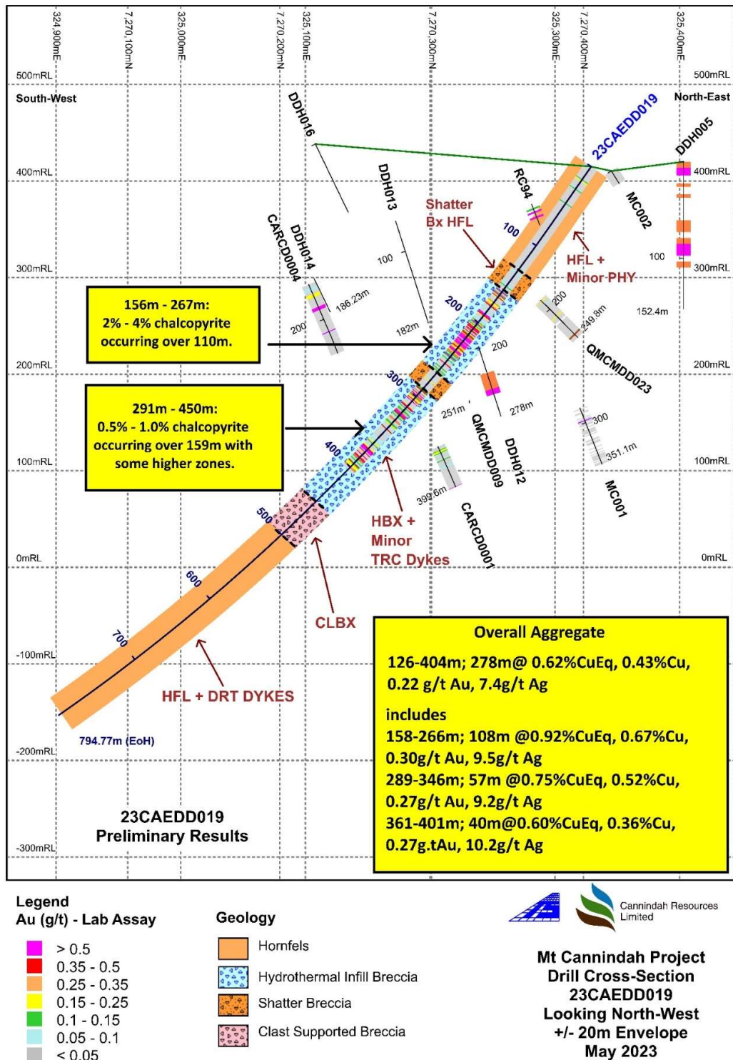
Fig 8. Cross section CAE Hole # 19, section line oriented south south west to north north east , looking north west, showing simplified geology ,extent of mineralised breccia and downhole gold results to 404m.
