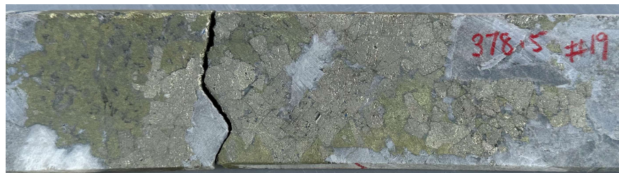
Semi-massive chalcopyrite, pyrite, calcite infill in breccia. CAE Hole 19, 378.5m. 1m interval 378m-379m : 1.90% Cu, 0.66 g/t Au, 83.7 g/t Ag, 6.45% S.
