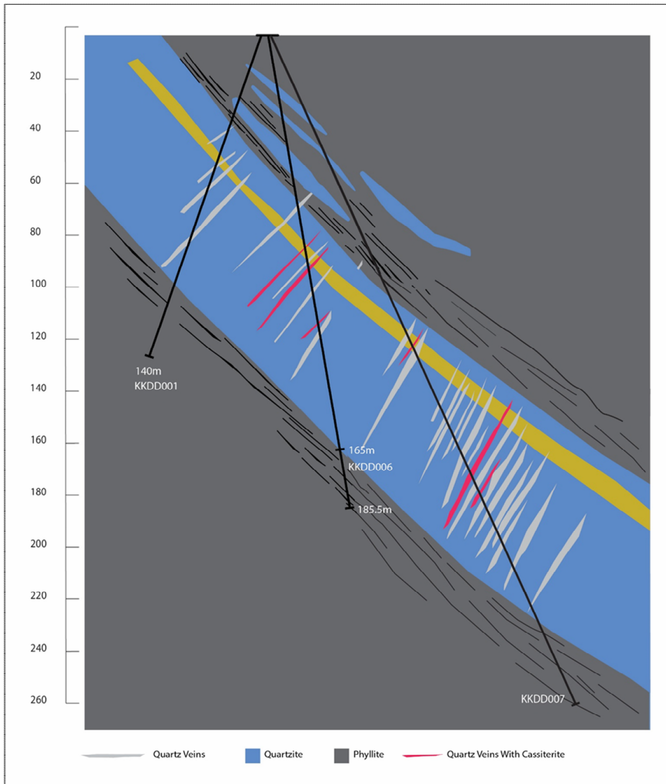
Figure 3 Interpreted cross section for holes KKDD001, 006 and 007 (Note that all the veins digitized are actual intersections that range in thickness from 0.3 to 2m.)
