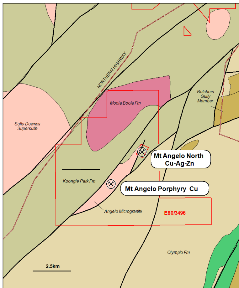
Figure 3: General geology of the Mount Angelo Area
