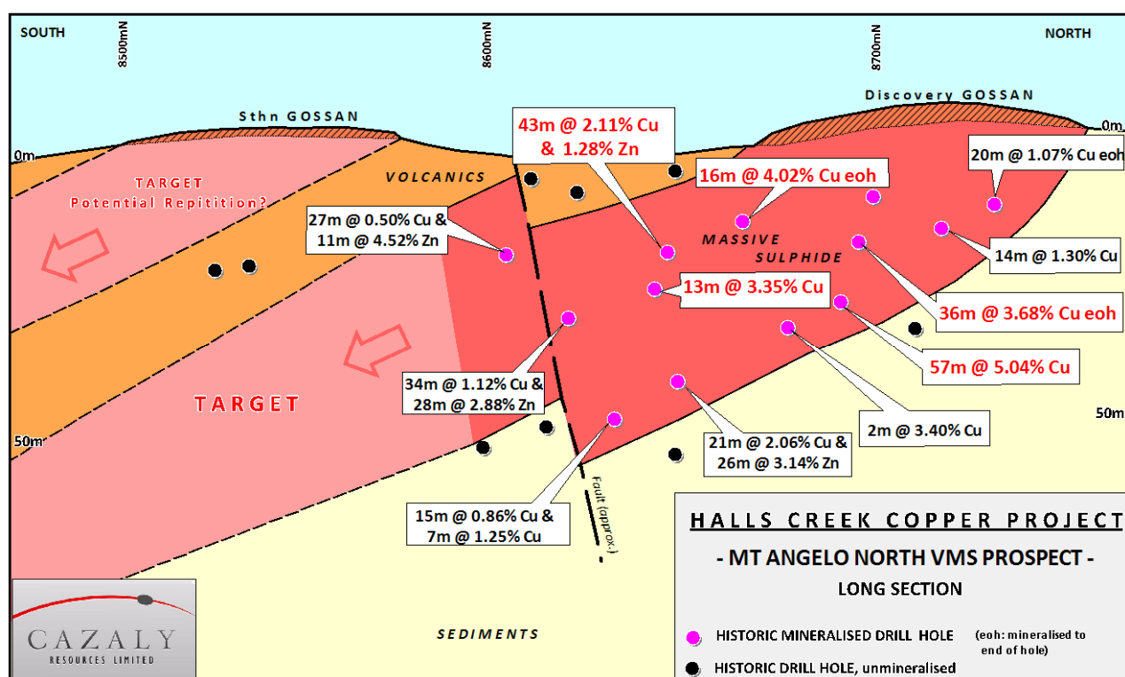
Figure 2: Long Section through the Mt Angelo North Deposit
