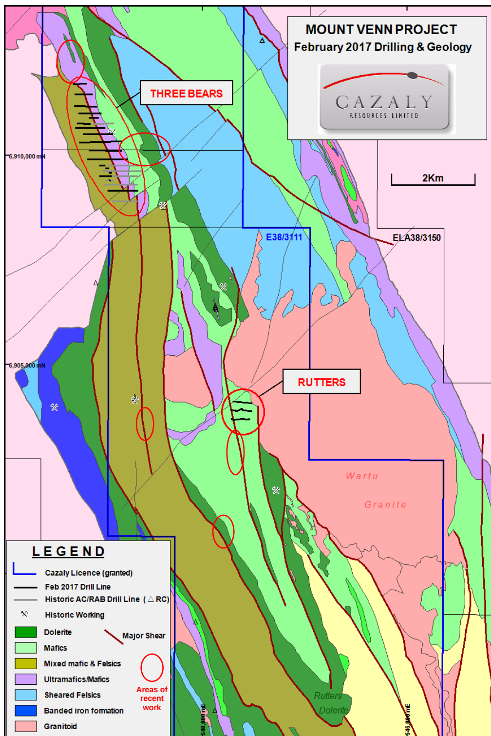
Figure 1: Geology & recent areas of work within the Mount Venn Greenstone Belt
