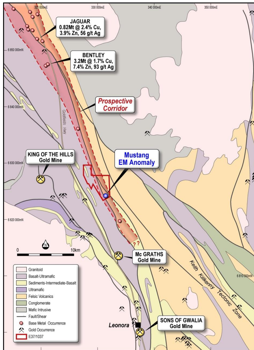
Figure 6: Regional geology and location of the Teutonic Project and Mustang Conductor showing proximity to the Jaguar and Bentley VMS deposits
