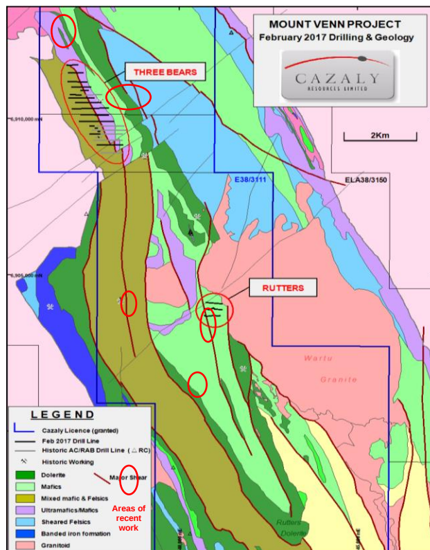
Figure 1: Yamarna Shear Zone & associated greenstone belts
