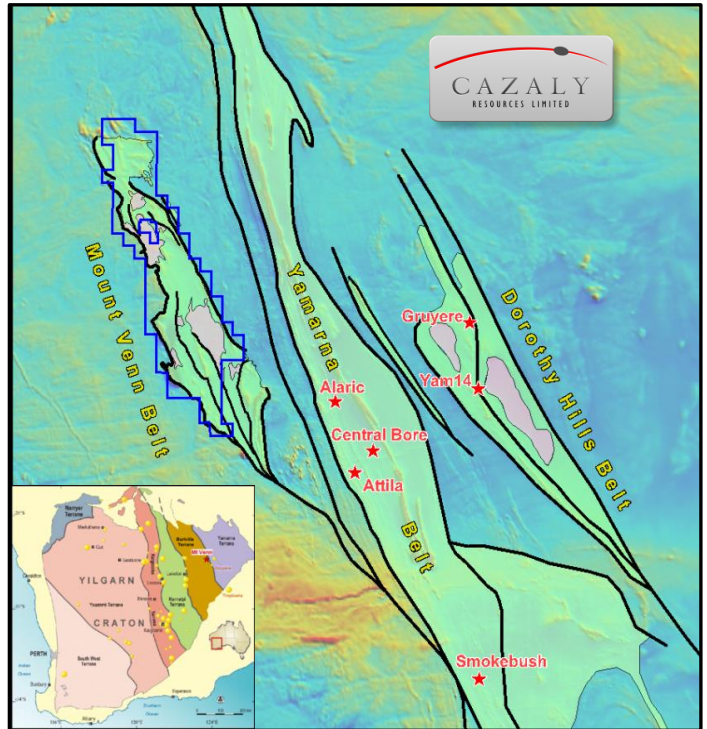
Figure 2: Geology and 2017 drill locations within the Mount Venn Greenstone Belt
