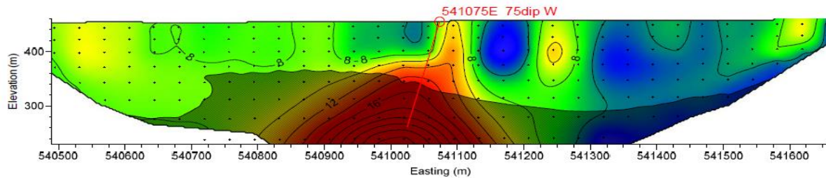
Figure 5: Ruffers Zinc-Gold Prospect, Dipole-Dipole IP anomaly, Line 2700mN
