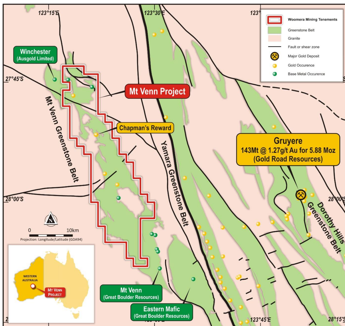
Figure 1: Mt Venn Project – Location and Regional Geology
