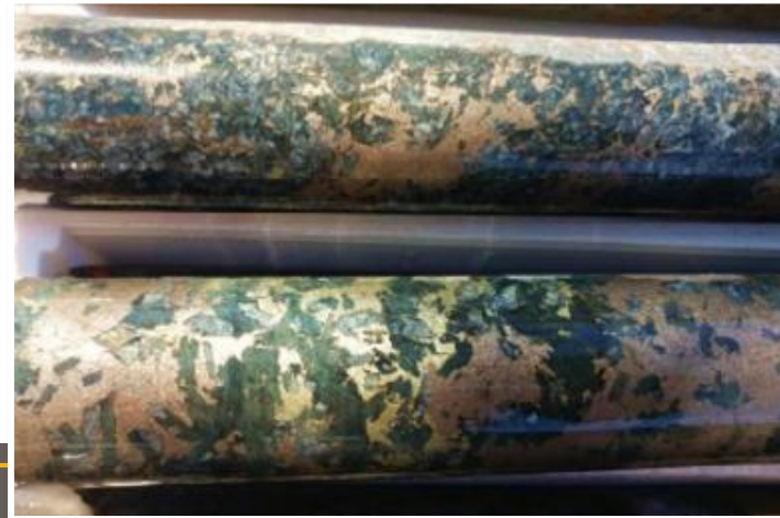
Semi-massive to massive pyo + cpy in core from Mt Venn (1)
