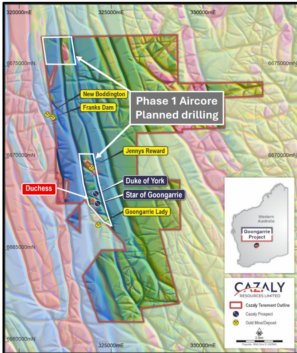
Figure 2. Initial aircore (AC) drilling is planned to test the Menzies-Boorara Shear corridor over high priority gold target areas.
