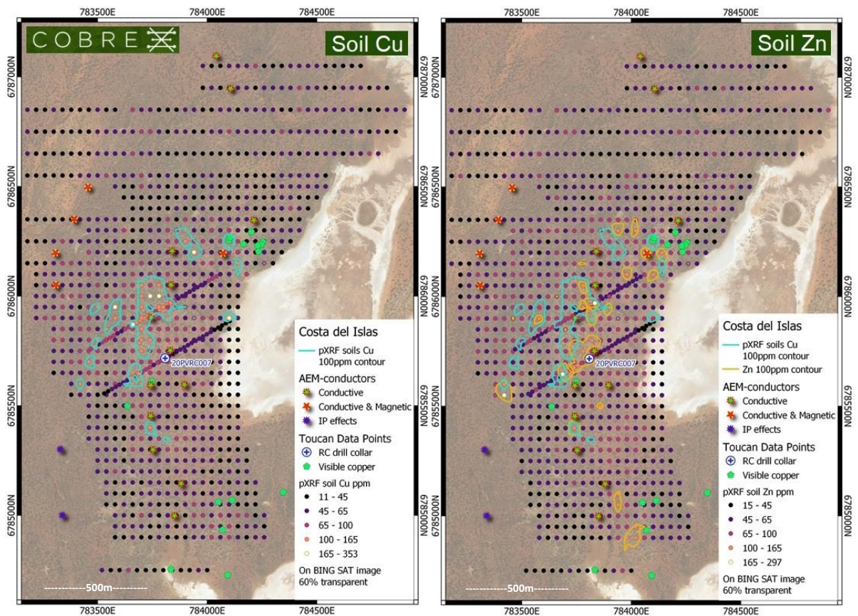
Figure 2: Costa del Islas Prospect exploration data comparing Cu and Zn soil responses (co-ordinates MGA94 Zone 50) Note: the left half of the above figure is included at higher resolution as Figure 3.
