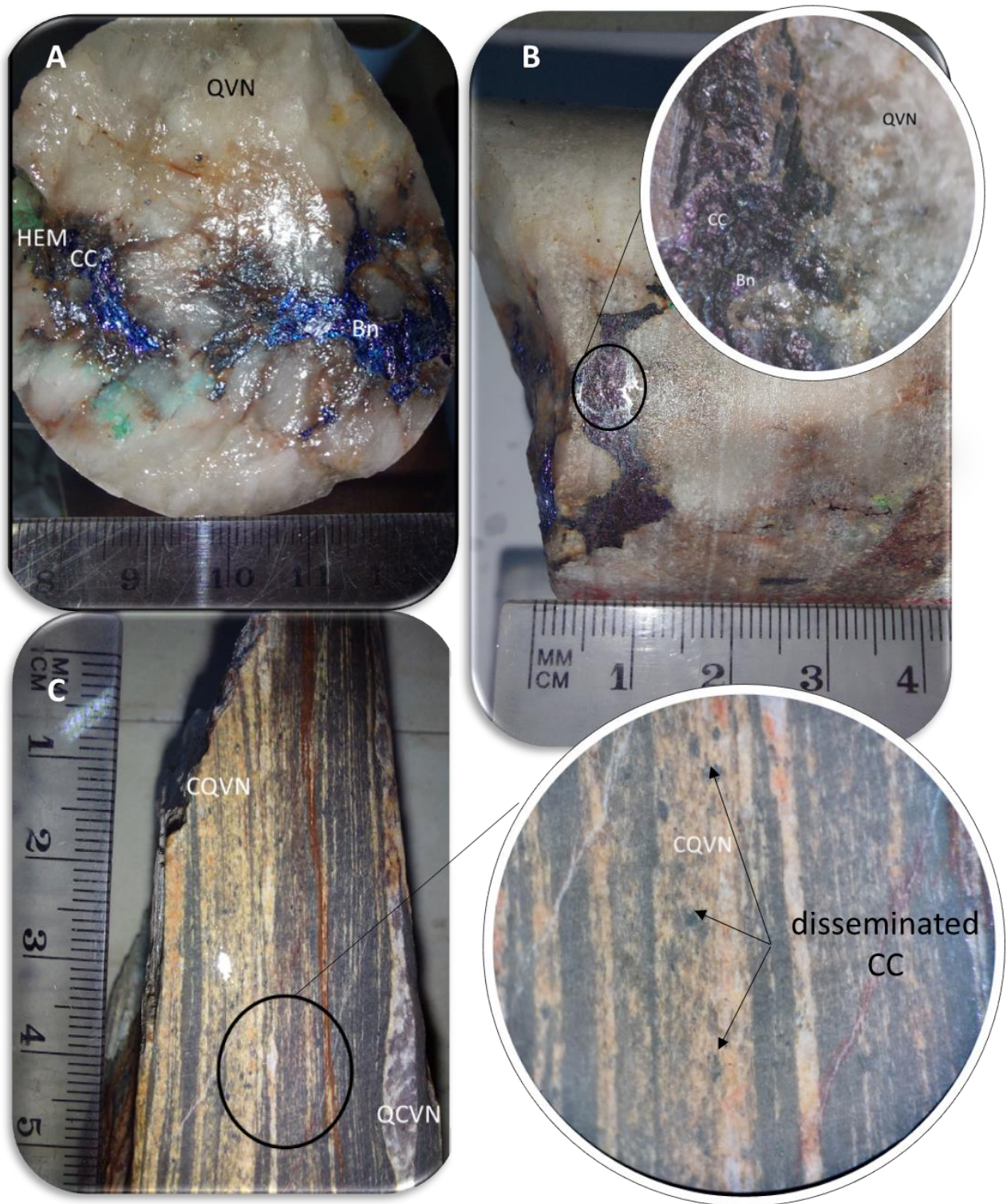
Figure 1. Examples of mineralisation intersected in NCP11-B. (A and B) Bornite (Bn) and chalcocite (CC) mineralisation hosted in a quartz vein, (C) Chalcocite mineralisation in carbonate (+ quartz) veins in the altered marl unit above the D'Kar – Ngwako Pan Formation contact.
