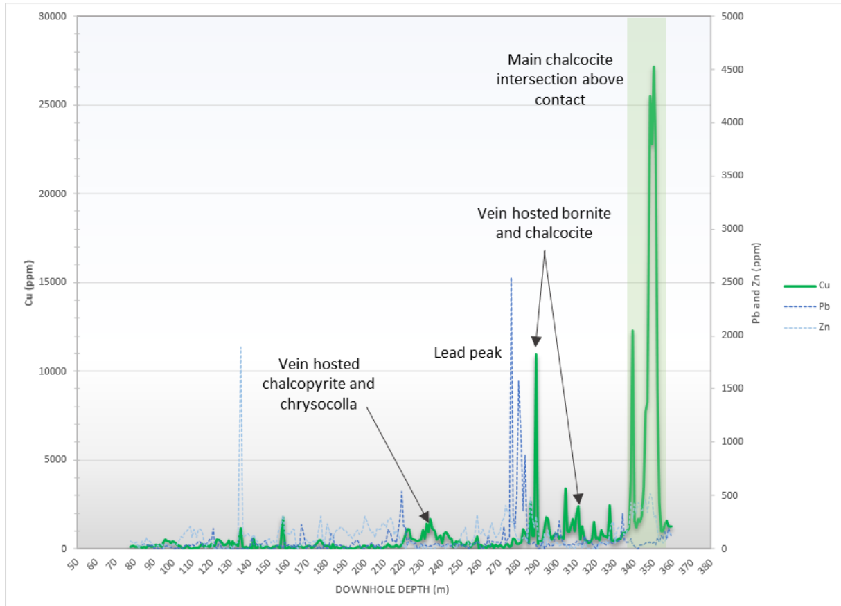
Figure 2. Graphical illustration of pXRF composite 1m sample measurements for the complete NCP11-B hole. Results confirm the abundance of visual copper mineralisation in drill logs. Distinct mineral zonation from chalcocite-bornite-chalcopyrite from the Ngwako Pan Formation contact is apparent.
