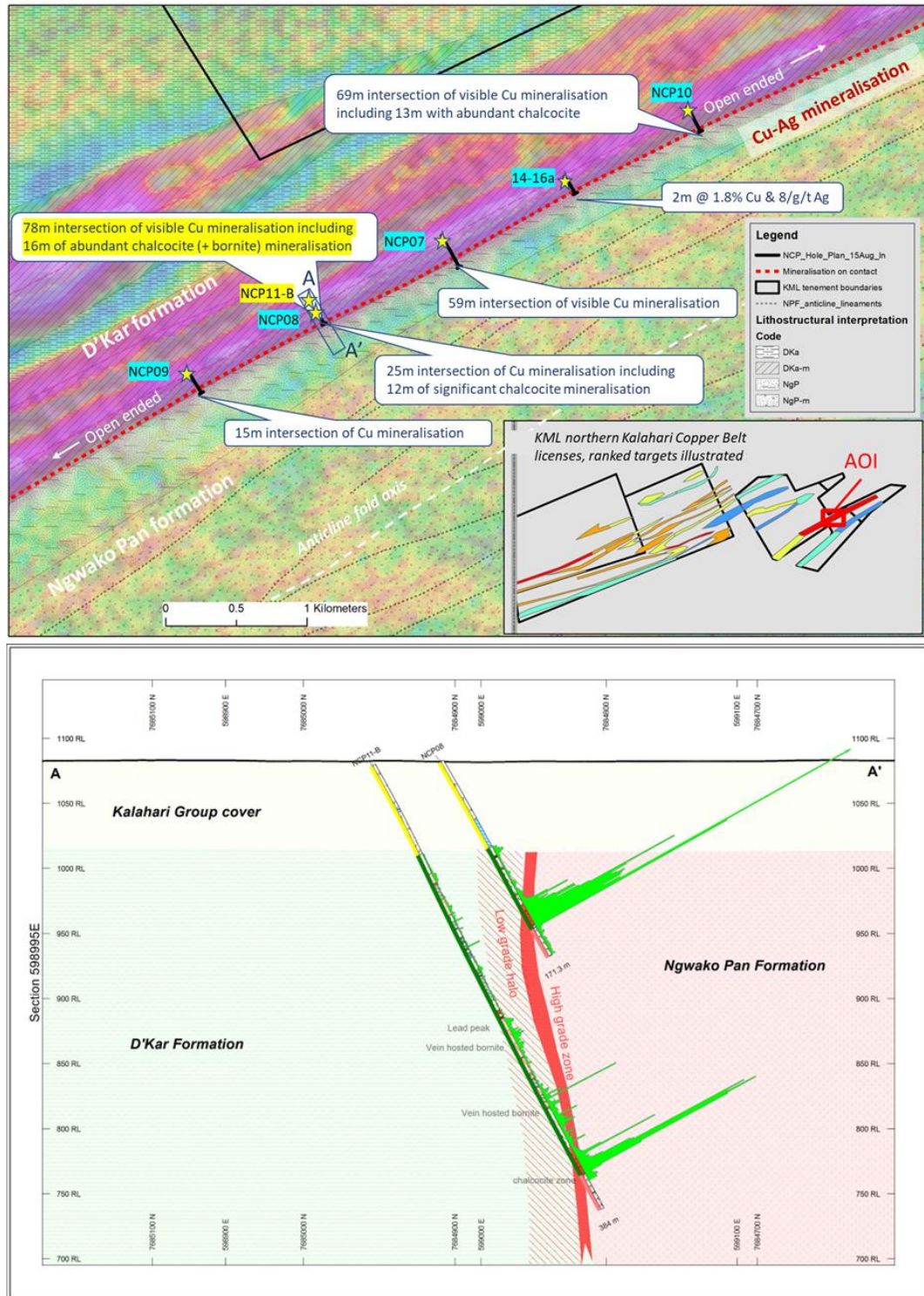
Figure 3. Plan view (above) illustrating drill positions on airborne magnetic data. Section (below) through NCP11-B and NCP08 illustrating mineralisation (green plot) related to the D'Kar / Ngwako Pan formation contact. Note the gentle folding of the contact interpreted from structural measurements of oriented core.
