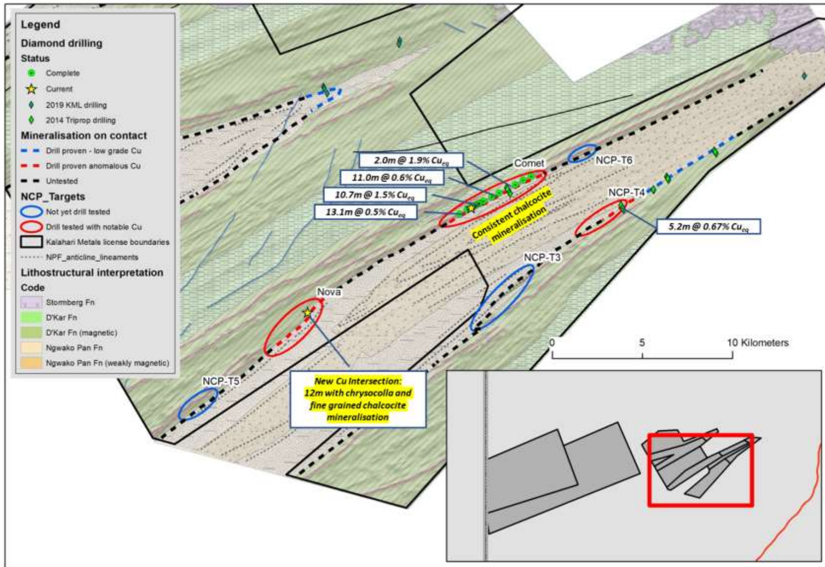
Figure 1. Plan map illustrating completed drill holes on lithological interpretation. Current and new targets along with notable drill assay results highlighted.
