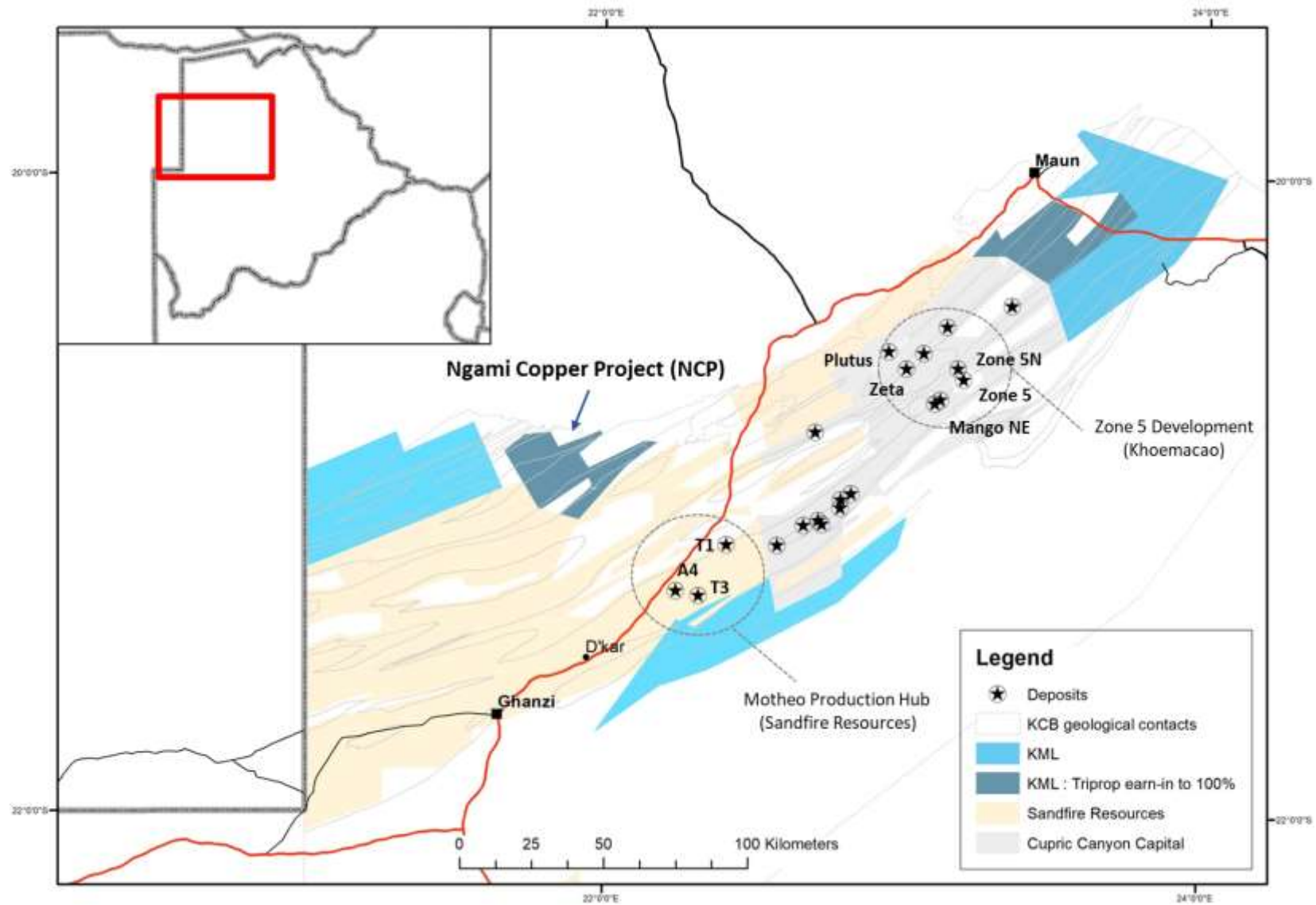
Figure 4. Locality map illustrating the position of KML's projects in the Kalahari Copper Belt.
