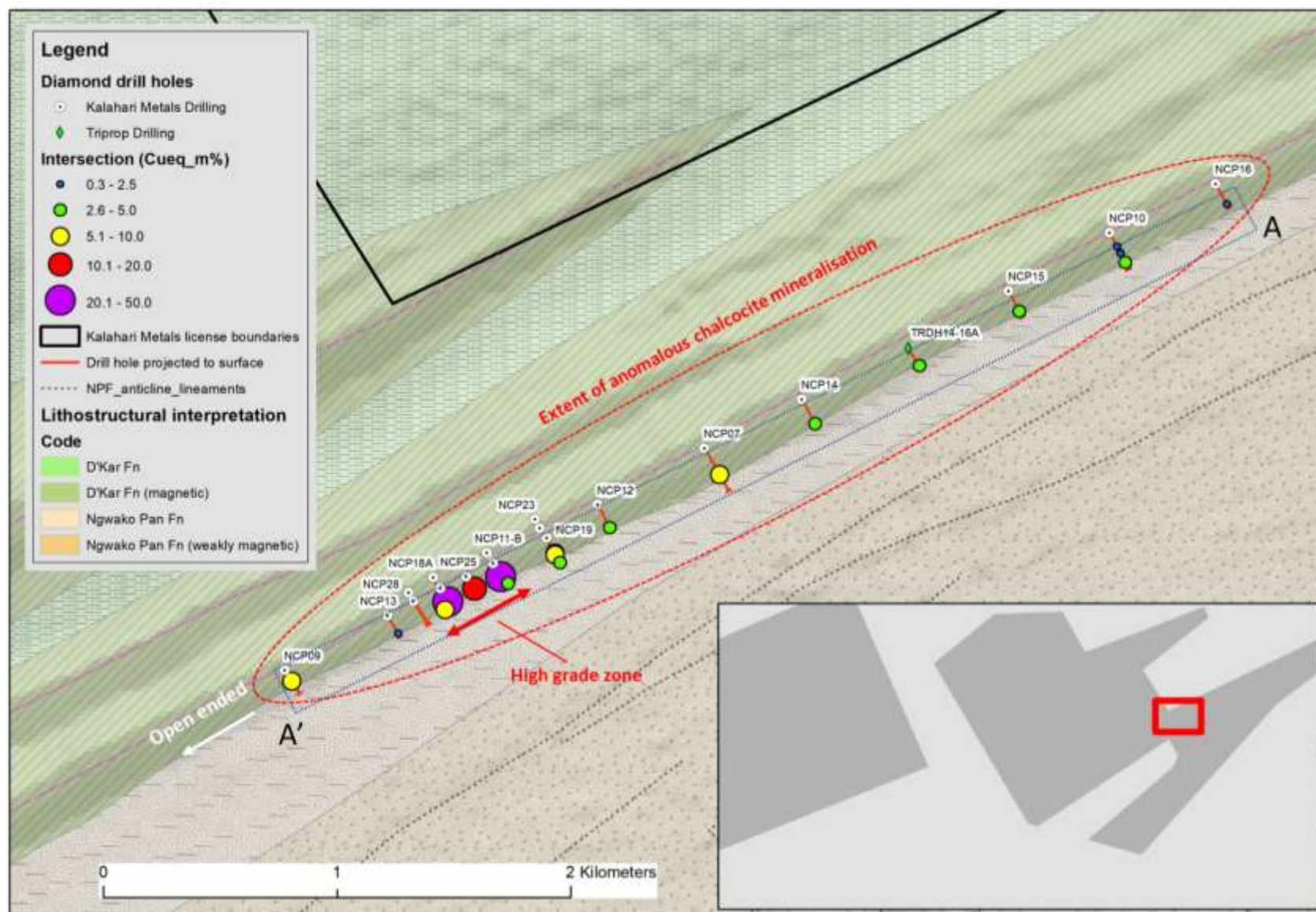
Figure 2. Plan map illustrating completed drill holes on lithological interpretation. Drill hole intersections are coloured by calculated Cu_{eq} m% which provides a useful method for comparing intersections. For holes where assays are pending, intersection Cu_{eq} m% has been estimated from pXRF and visual estimates. The location of the 3D long-section illustrated in Figure 2 is highlighted.
