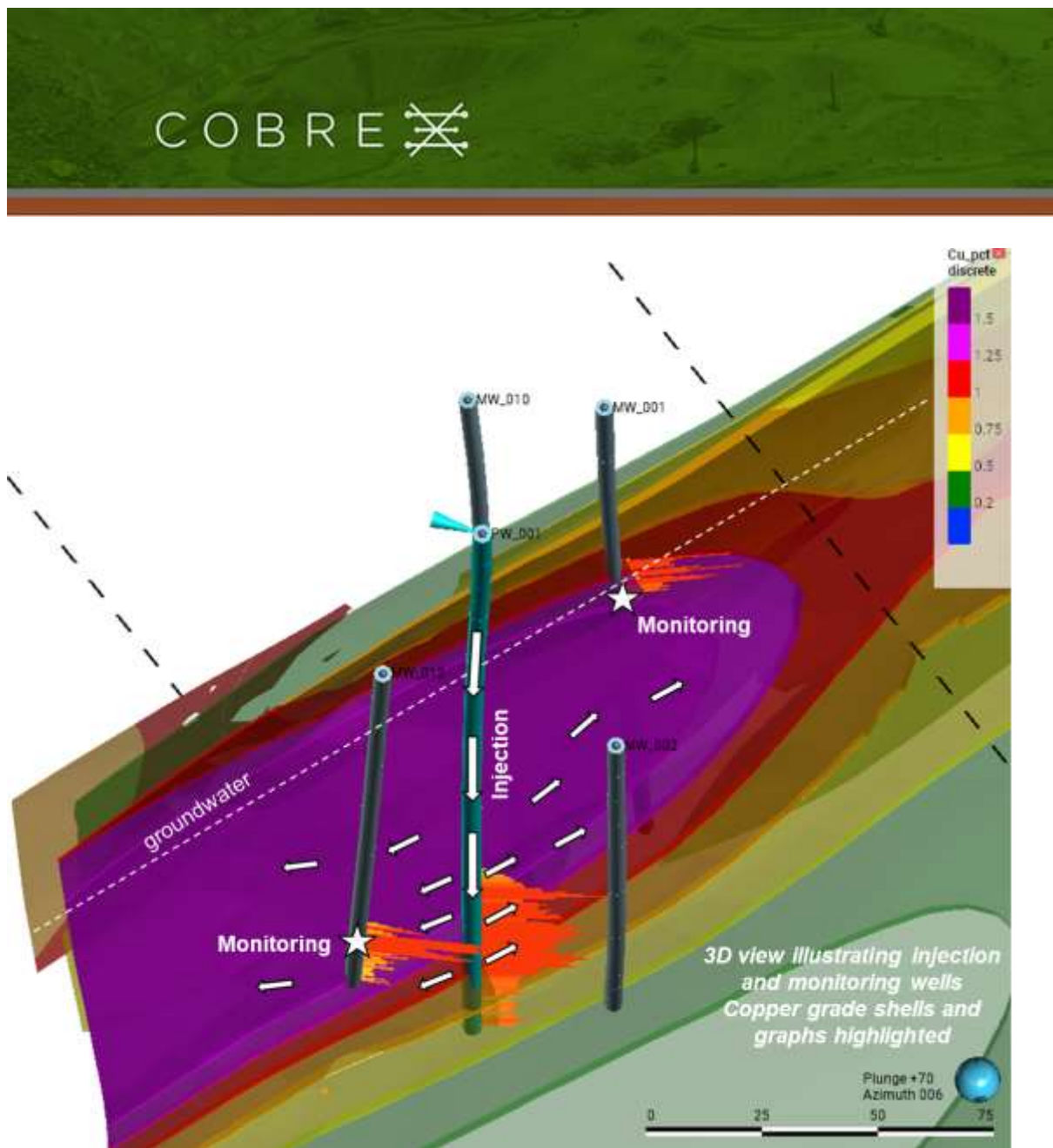
Figure 2. Oblique 3D view illustrating grade shells with injection and monitoring wells. Arrows indicate schematic flow of injected water relative to monitoring wells. A graphical log of intersected Cu grade is provided.
