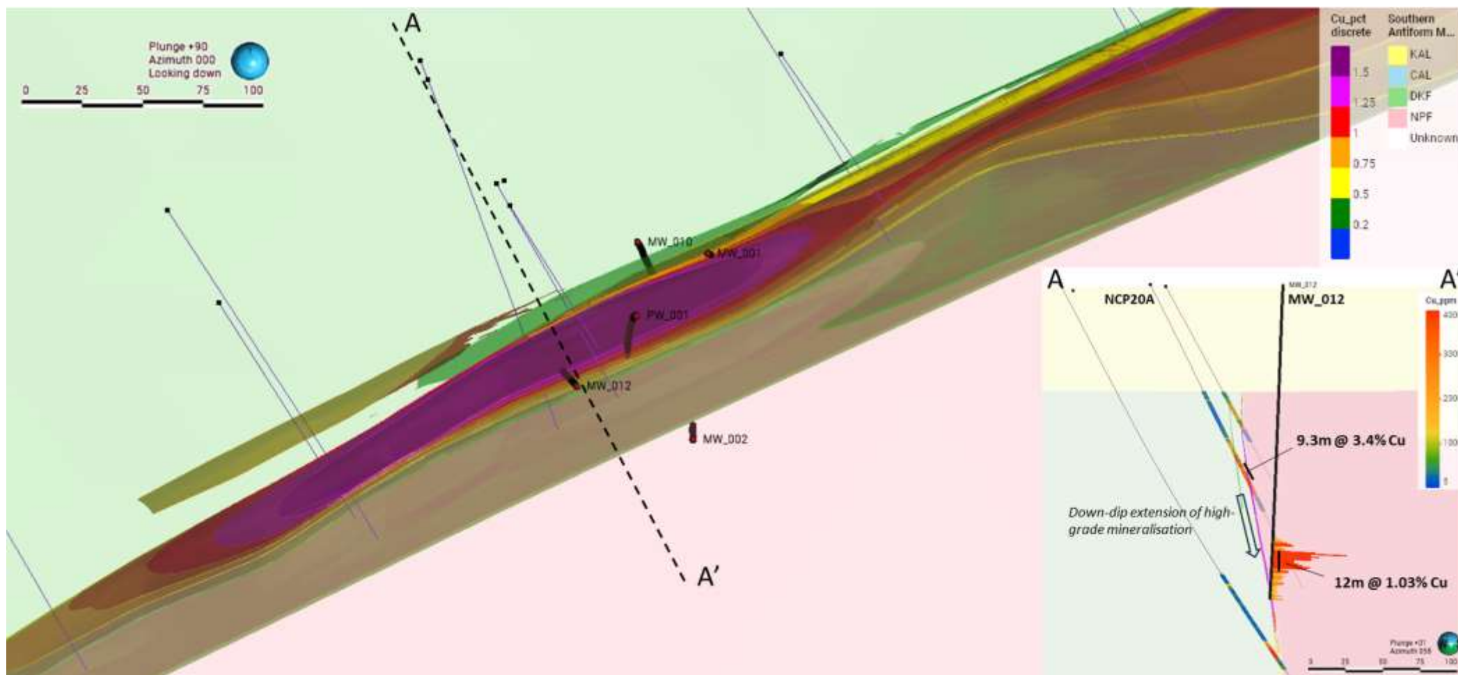
Figure 3. Plan view (looking down) of the geological and mineralisation model illustrating monitoring and injection wells. Section A-A' illustrates monitoring well MW_012 with Cu grade graphically illustrated. The copper grades intersected in this hole provide evidence for down-dip extension to high-grade mineralisation intersected in drill hole NCP20A.
