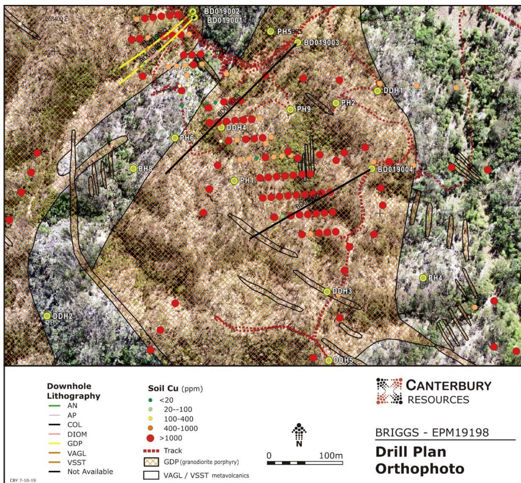
Figure 2 Briggs Drill Plan, Central Porphyry Zone
