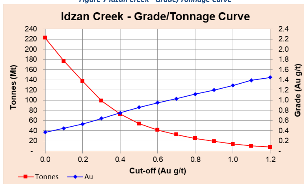
Figure 7 Idzan Creek - Grade/Tonnage Curve
