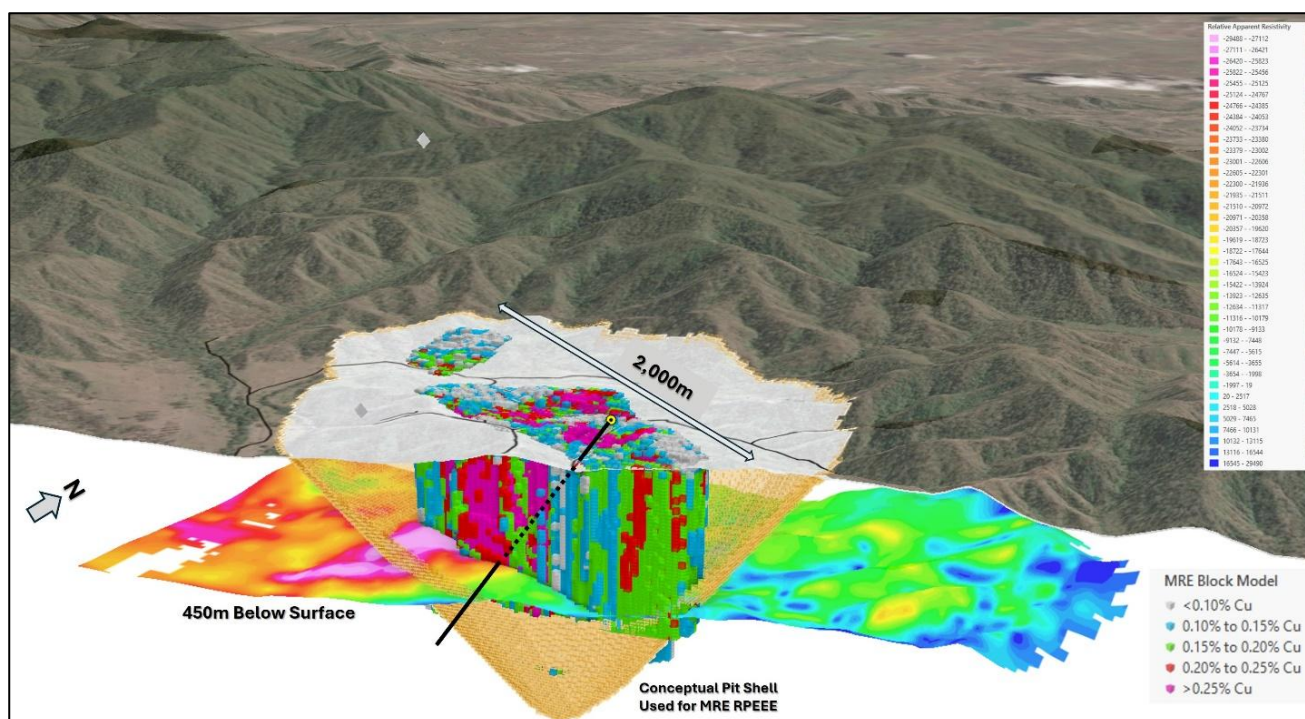
Figure 4 Oblique 3D view of Briggs showing Apparent Resistivity at 450m below surface and the juxtaposition of this anomaly with higher interpolated copper grades in the 2025 MRE block model.
