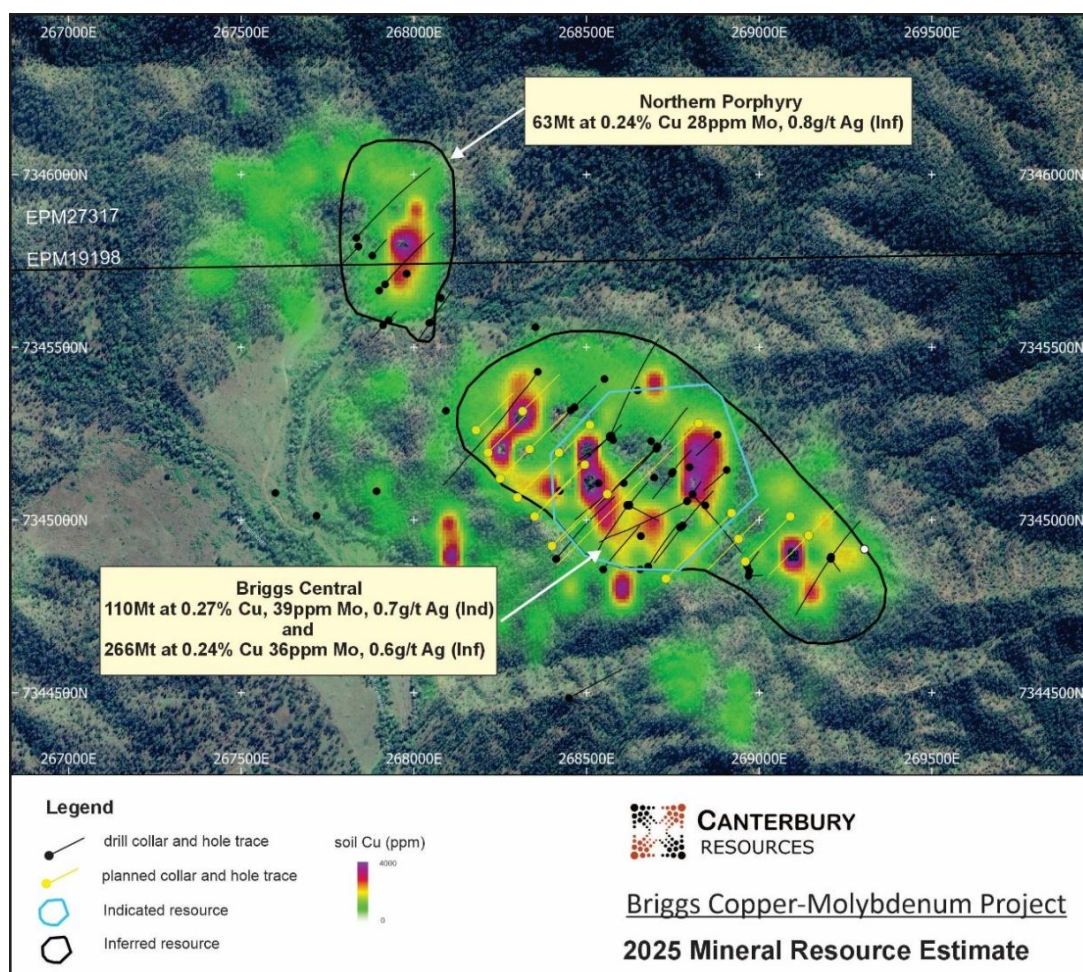
Figure 2 Plan of MRE outline, Cu-in-soil geochemistry, plus historical and planned drill holes
