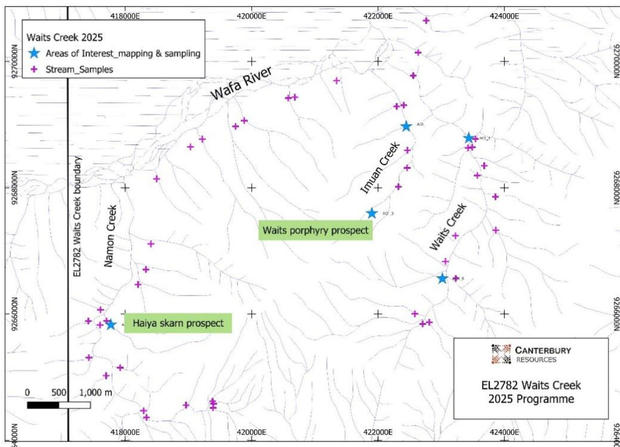
Figure 7 Waits Creek and Haiya Creek prospect areas and 2025 field program
