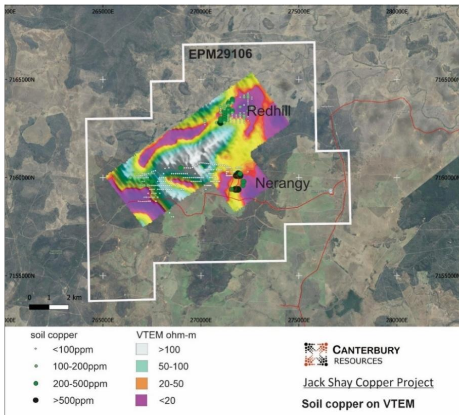
Figure 5 Plan of Jack Shay prospect locations, Cu in soil geochemistry and VTEM
