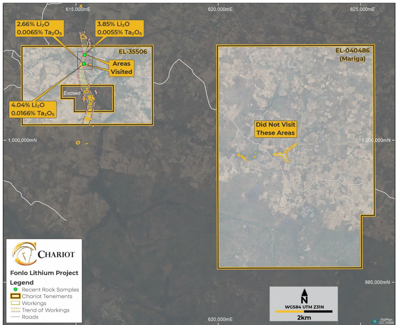
Figure 1: Fonlo project map showing areas visited and sample assay results.
