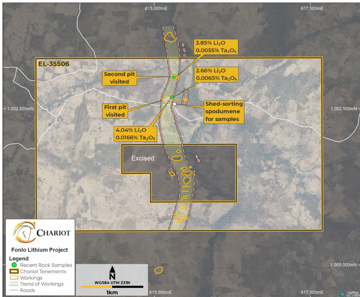
Figure 2: Fonlo project map showing pits visited and sample assay results.
