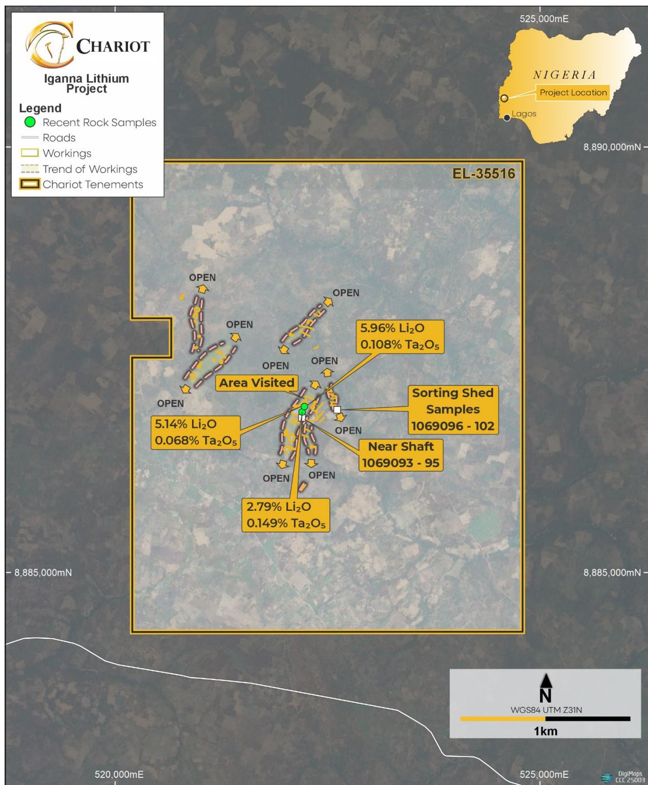
Figure 3: Iganna project map showing area visited and sample assay results.
