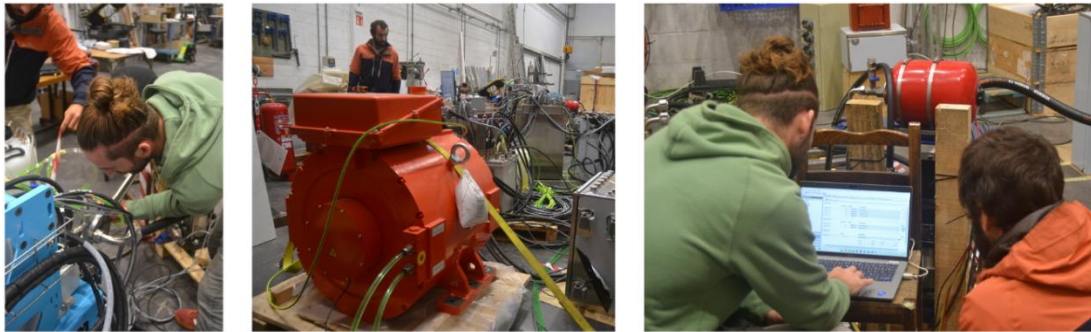
Integration testing of the electrical, control and cooling system prior to installation in the Electrical Module
