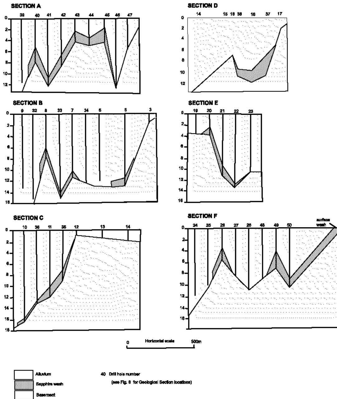
Fig. 7. Geological cross sections (A-F) showing alluvial overburden, sapphire wash and basement. Note - a horizontal datum is assumed.
