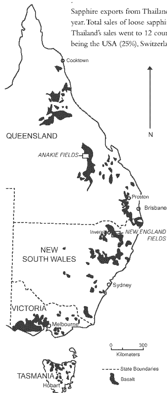
Figure 4 - Distribution of Cainozoic volcanic provinces in Eastern Australia. Economic deposits of sapphire have been mined in the Anakie Field and the New England Field. (Prepared by R.R.Coenraads)
