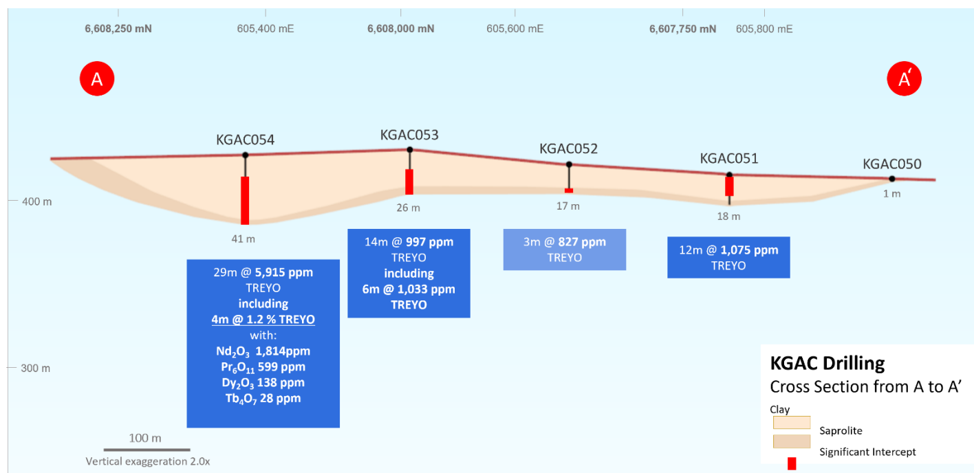
Figure 4. Cross-section (A - A') of drilling at the Karloning REE Project.
