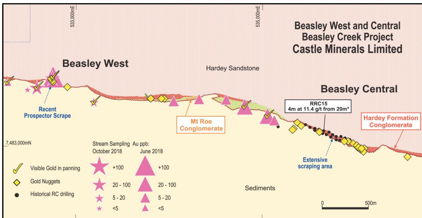
Figure 2: Beasley Creek targets, geology and sampling (Enlargement)
