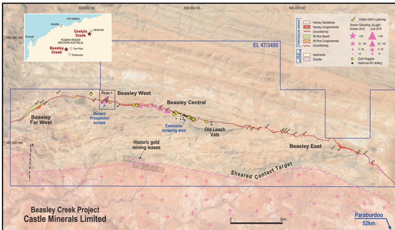
Figure 1: Beasley Creek targets, geology and recent sampling
