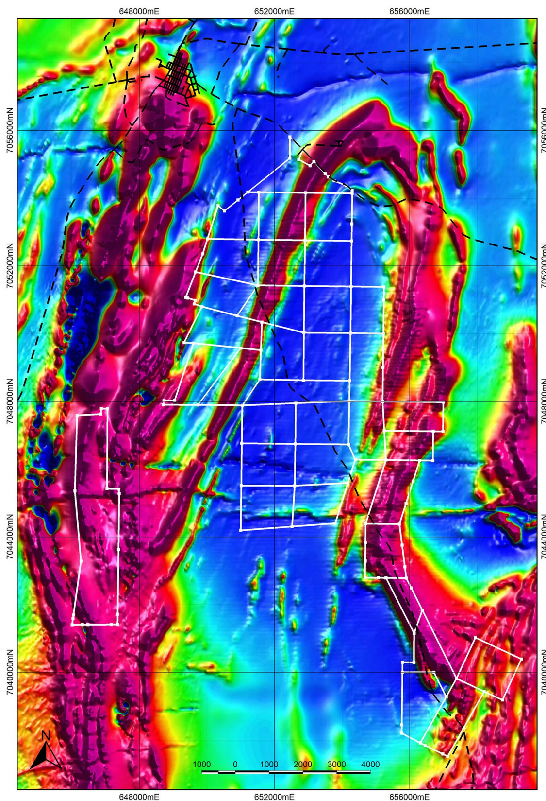
Figure 4: Magnetic anomalies identified at Westgold's (ASX:WGX) Murchison Gold Project and Meekasan's tenure identified by the white lines
