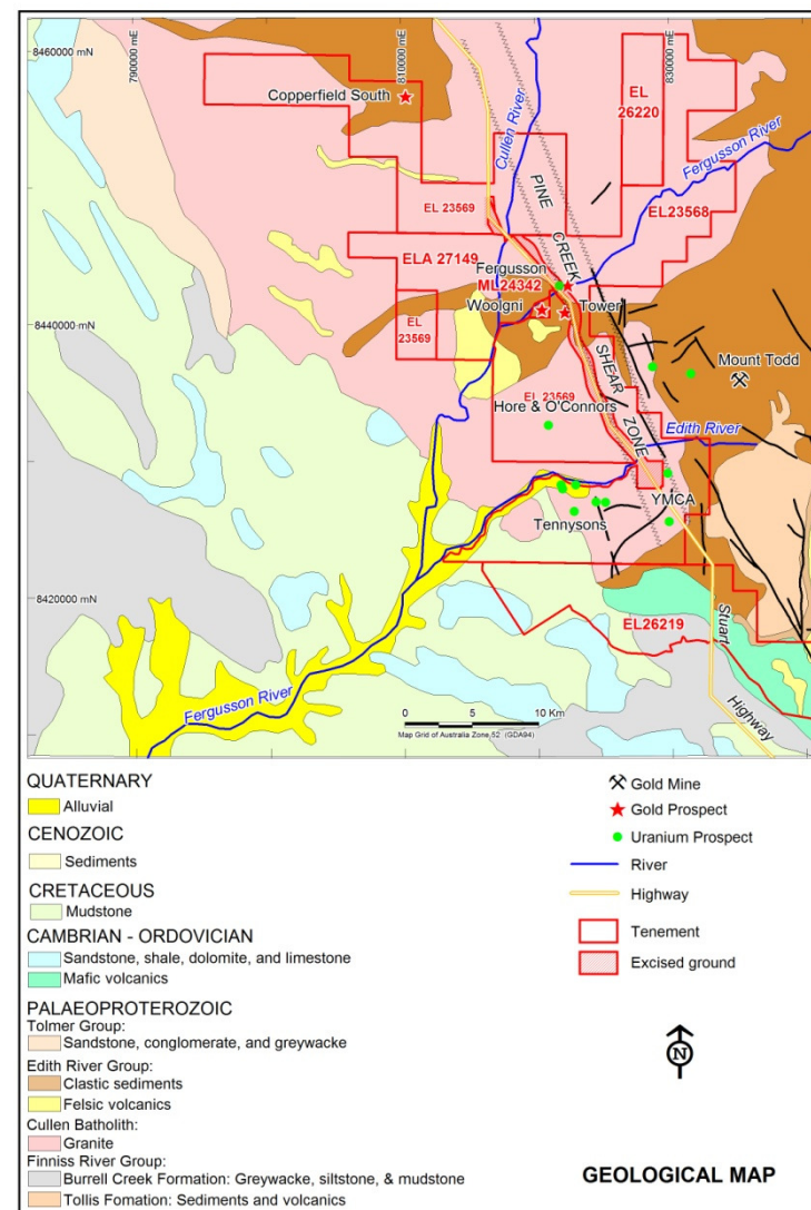
Figure 2: Woolgni-Edith River Project geology
