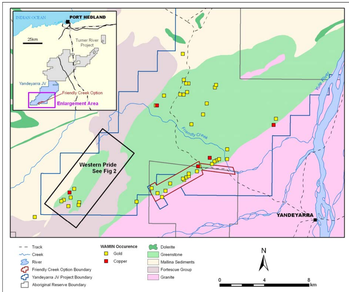
Figure 1: Location of rock sampling results and geological reconnaissance in the south west of the Yandeyarra Joint Venture Project
