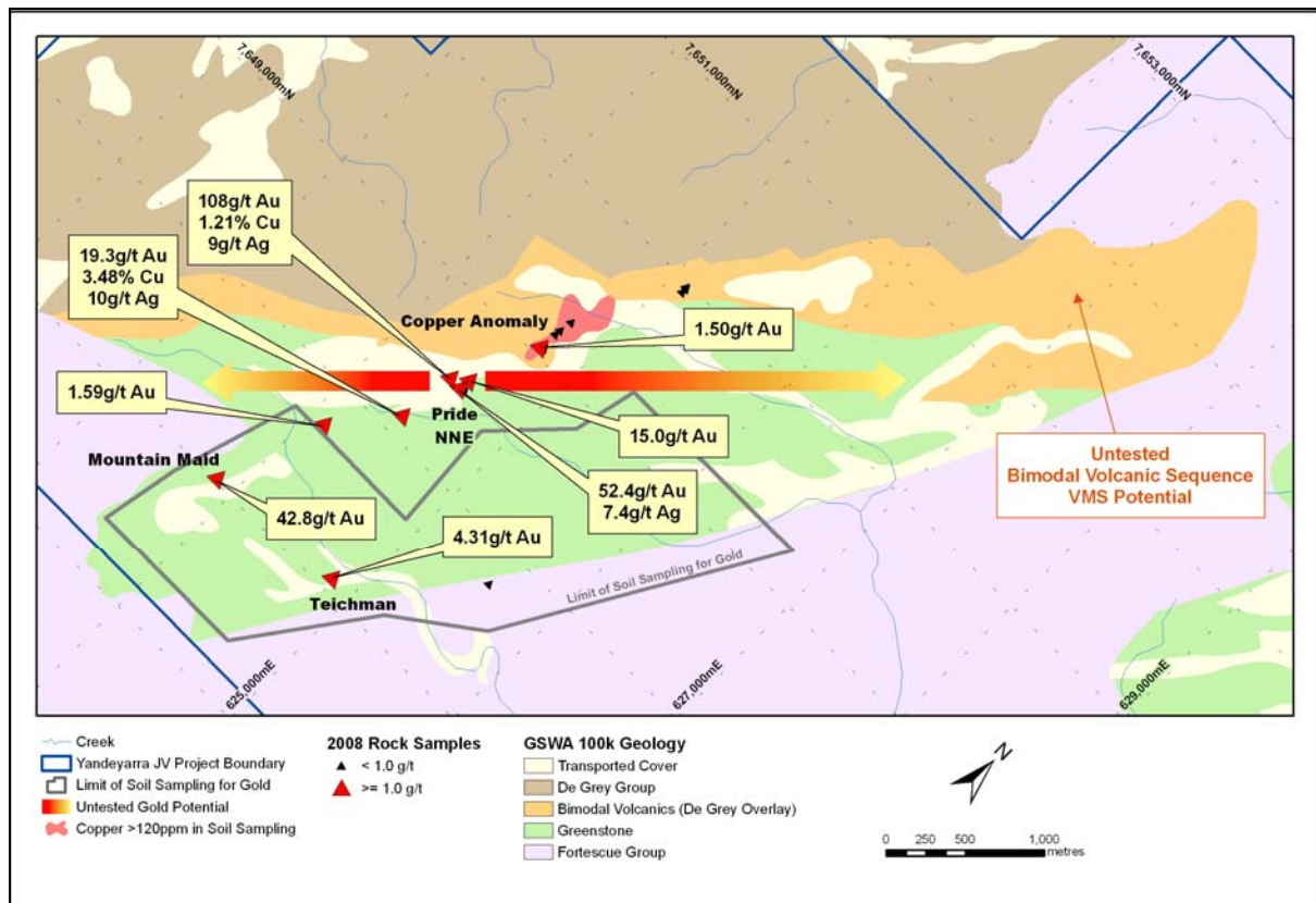
Figure 2: Rock sampling results and exploration targets in the Western Pride area, Yandeyarra Joint Venture Project
