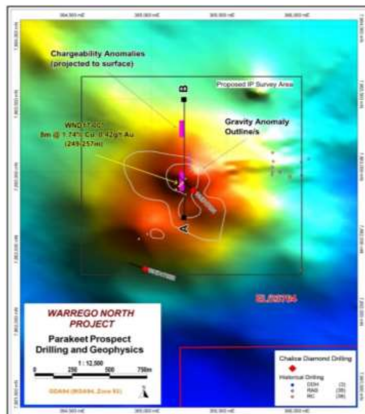
Figure 2. Parakeet aeromagnetic image with superimposed gravity, IP and drill collars.
