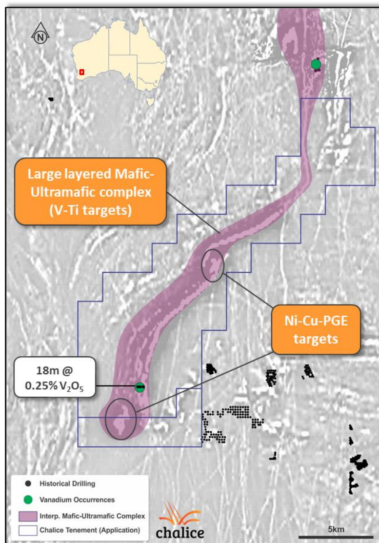
Figure 4. Priority Target Areas within Igneous Complex.
