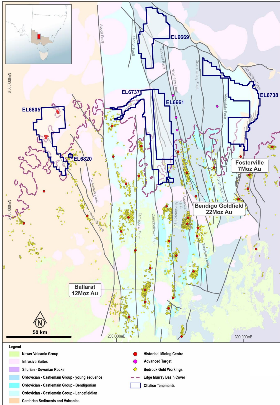
Figure 3. Interpreted geology of Central Victoria showing Chalice tenure
