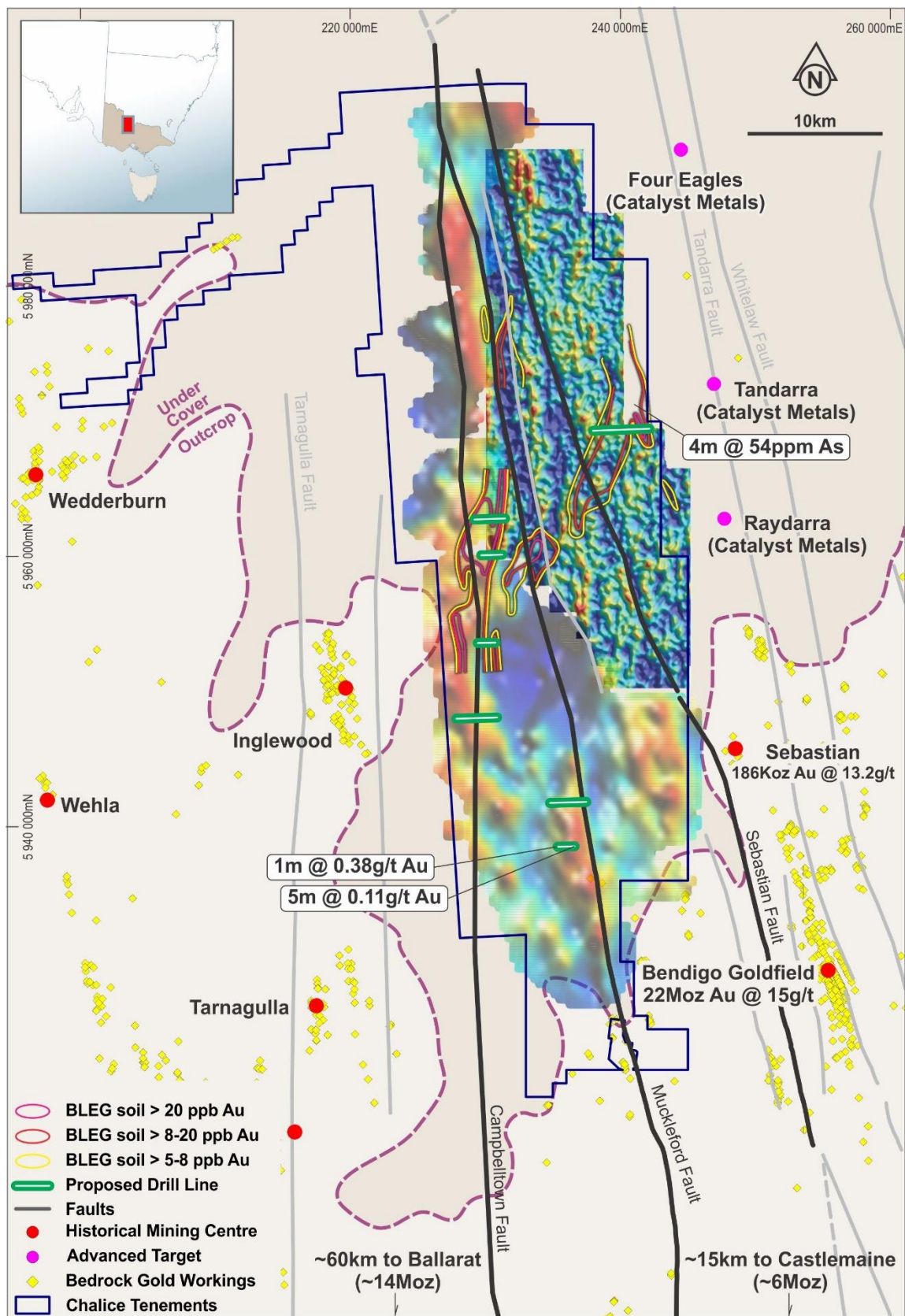
Figure 1. Planned RC/aircore drill traverses over first vertical derivative gravity with gold-in-soil anomaly contours
