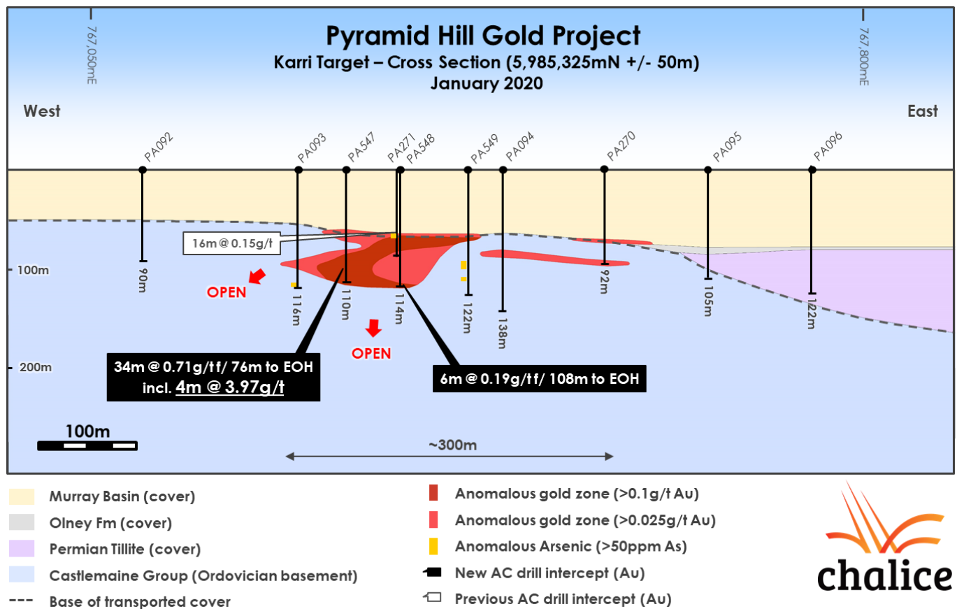
Figure 2. Karri Target Cross Section (5,985,325mN +/- 50m).
