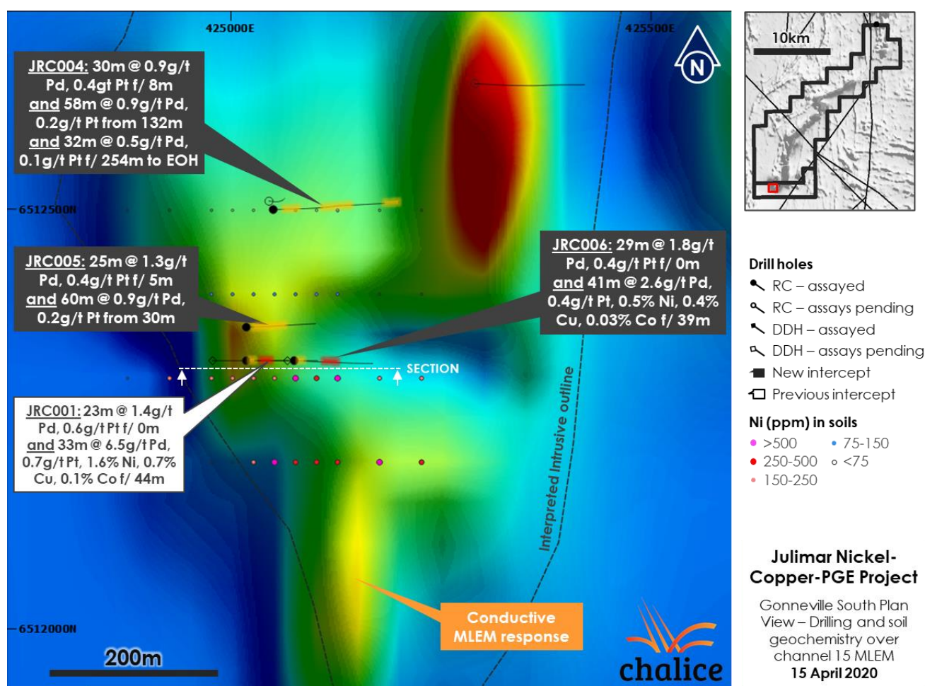
Figure 2. Gonneville South Plan View – Drilling and soil geochemistry over channel 15 MLEM.
