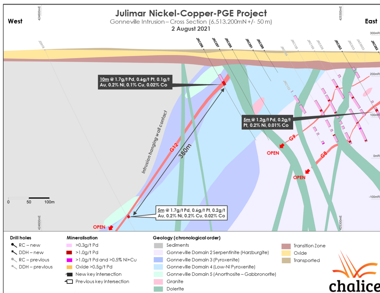
Figure 3. Gonneville G12 zone Cross Section 6,513,200mN +/- 50m.
