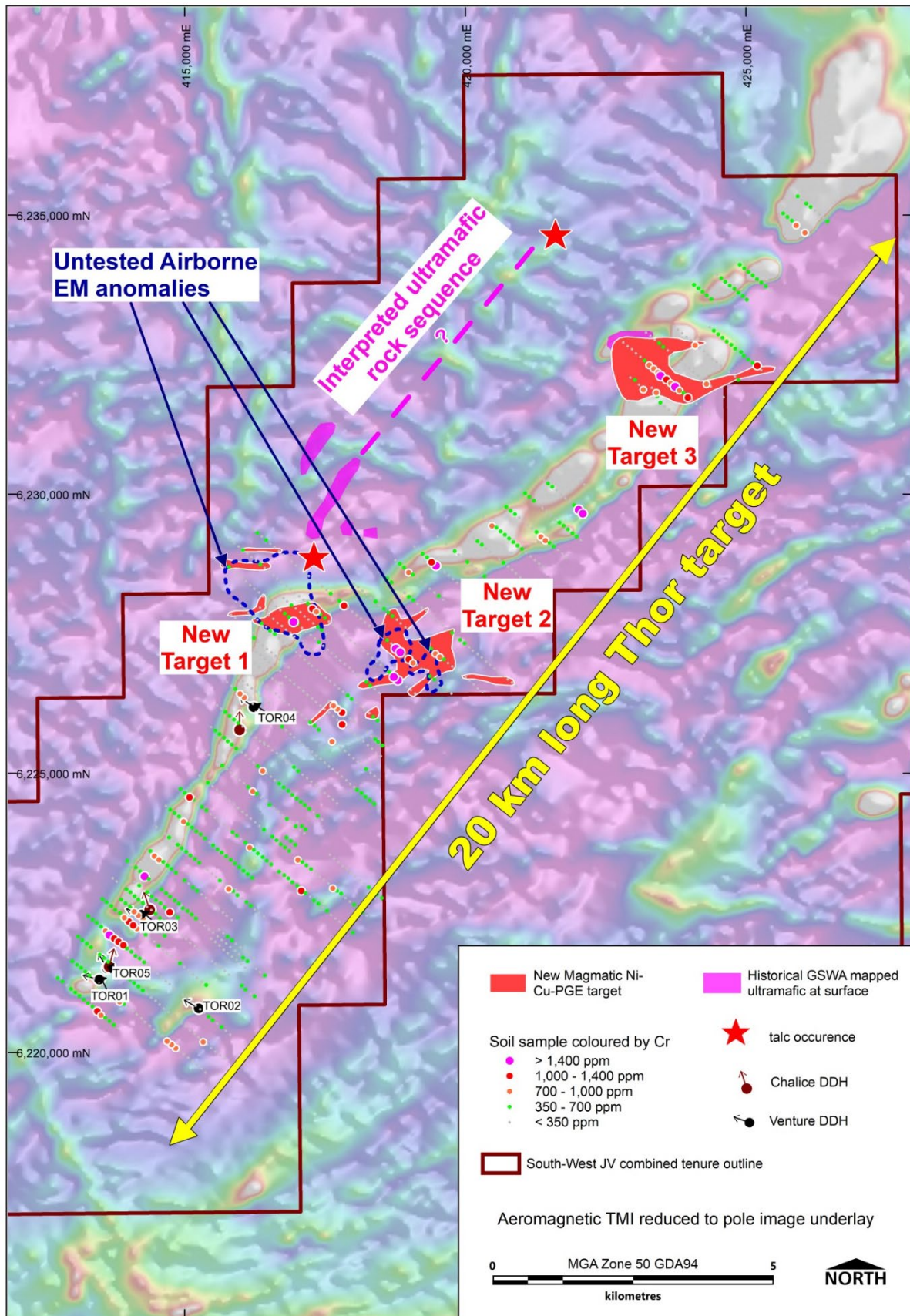
Figure One | South West Project - Chalice's Auger Surface Geochemistry Phase One and Two results on aeromagnetics over the Thor Target
