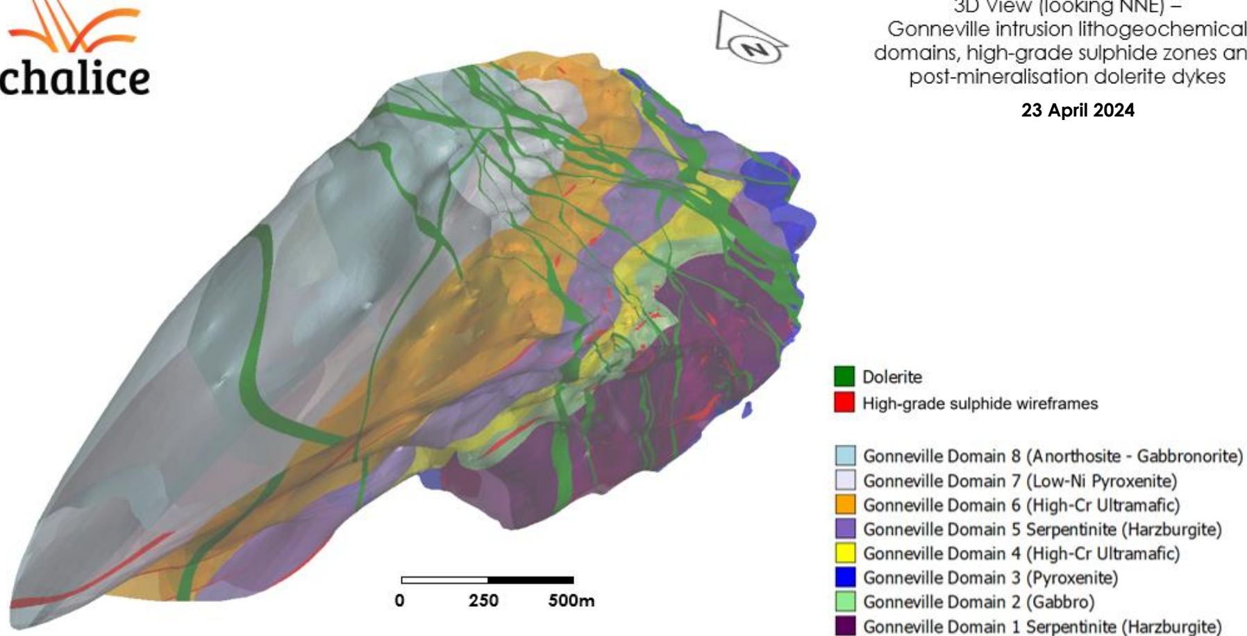
Figure 5. Gonneville 3D view (looking NNE) – lithogeochemical domains, high-grade sulphide zones and post-mineralisation dolerite dykes.
