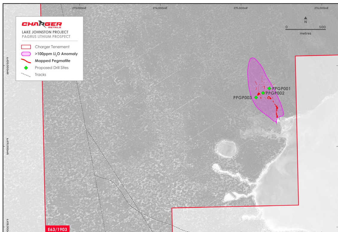
Figure 2. Pagrus Lithium Prospect showing the location of planned RC drill-holes in relation to outcropping pegmatites and lithium-in-soils anomaly.
