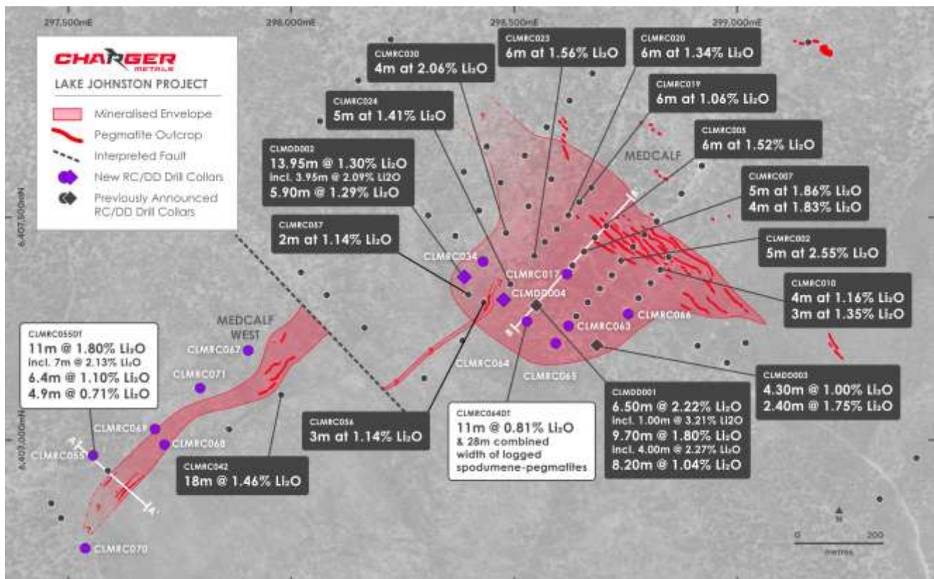
Figure 2. Medcalf Spodumene Deposit showing new RC and diamond drilling results relative to the spodumene-bearing pegmatite swarm and selected Diamond and RC drill results.
