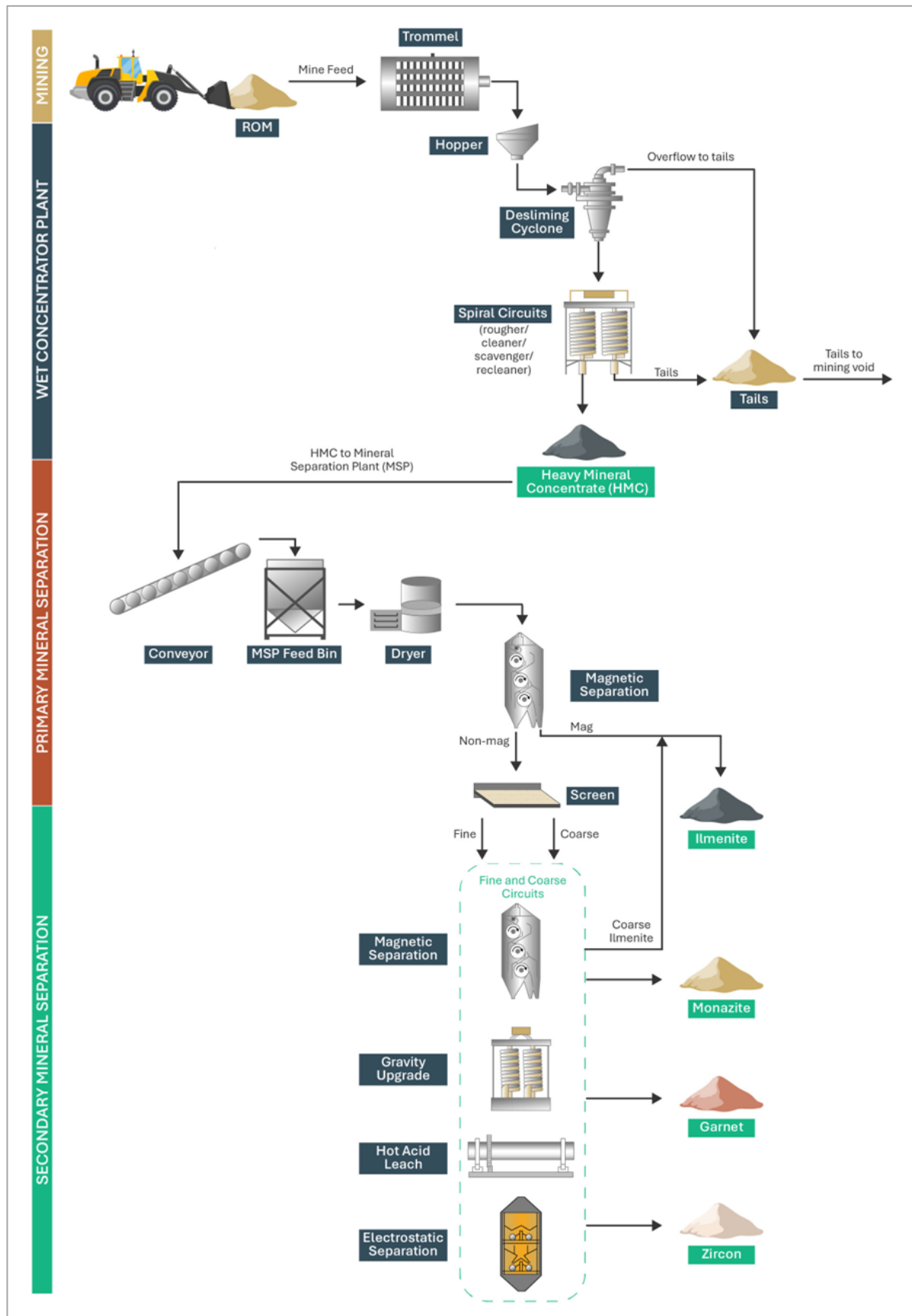
Figure 5: Preliminary summary flow sheet, based on standard Heavy Minerals Sands processing technologies to derive an ilmenite product with non -magnetic product streams.
