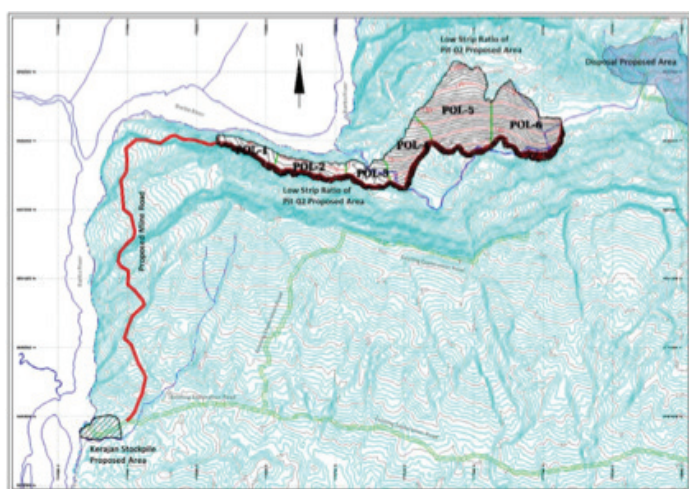
MINE LAYOUT MAP OF LOW STRIP RATIO PCI COAL
