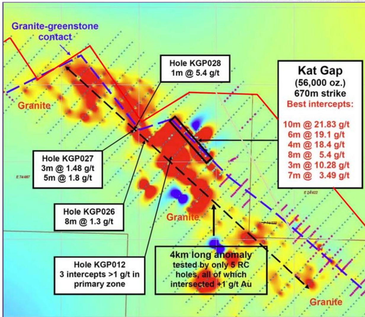
Figure 7 Drill results & gold geochemistry
