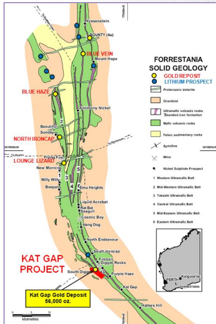
Figure 3 Main Gold Deposits-Forrestania Belt
