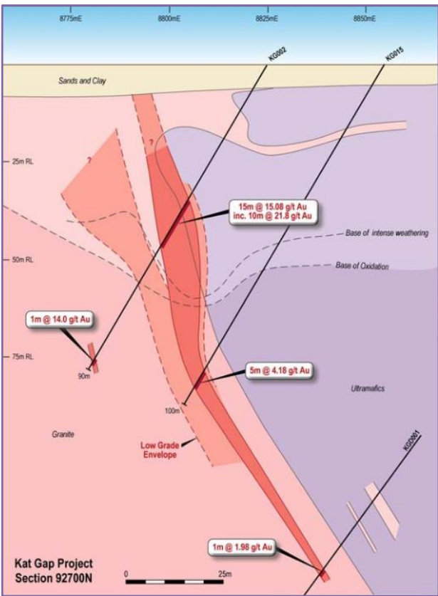
Figure 5 Drill Section 92700N
