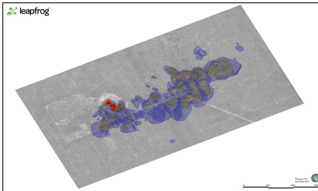
Figure 5 Implicit model showing both Lady Ada and Lady Magdalene extent of mineralisation after Phase I drilling ( July 2017 )
