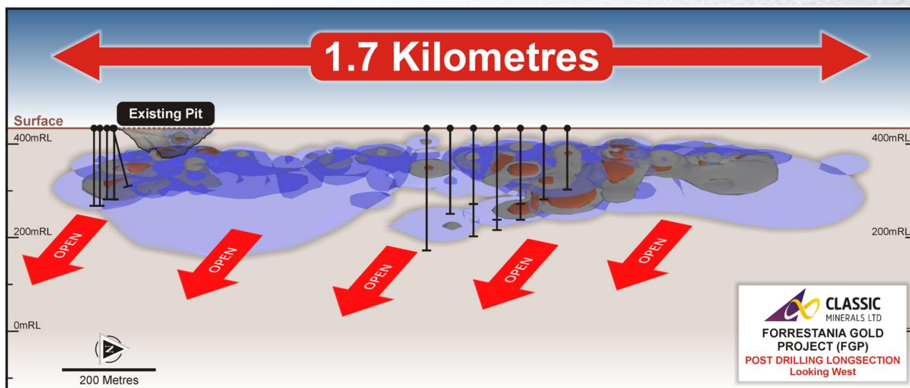
Figure 6 S-N Long-section showing both Lady Ada and Lady Magdalene with recent drillholes and current extent of mineralisation
