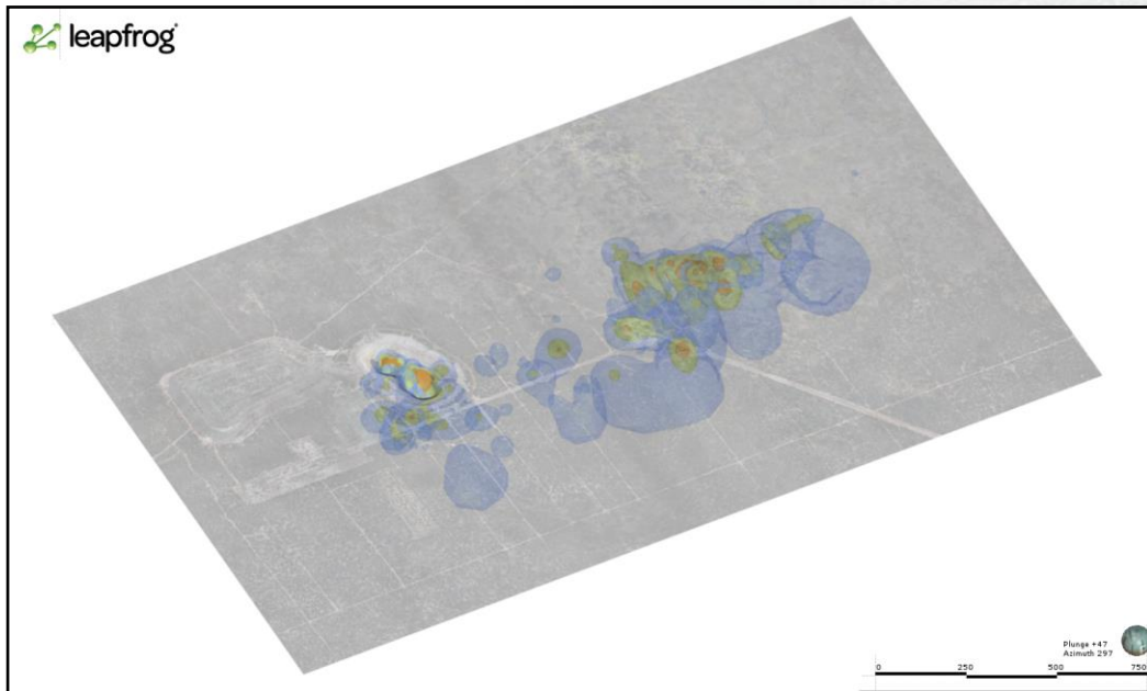
Figure 4 Implicit model showing both Lady Ada and Lady Magdalene extent of mineralisation before Phase I drilling ( May 2017 )
