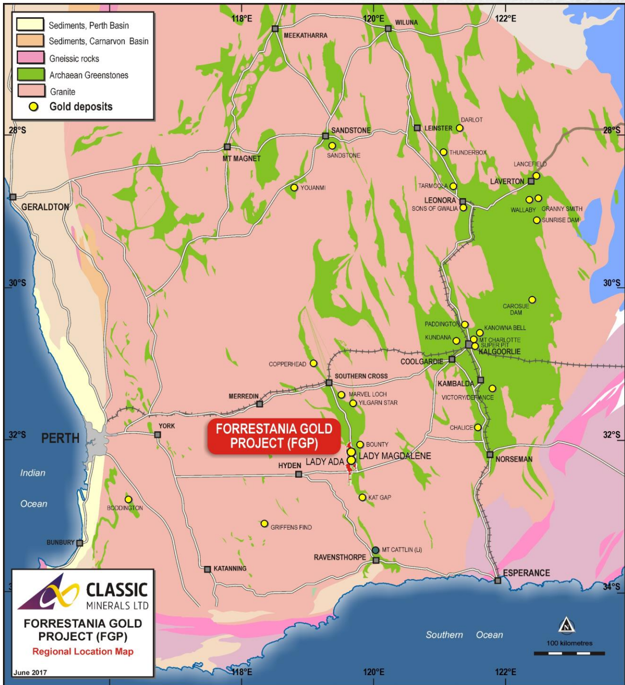
Figure 7 Location of the Forrestania Gold Project
