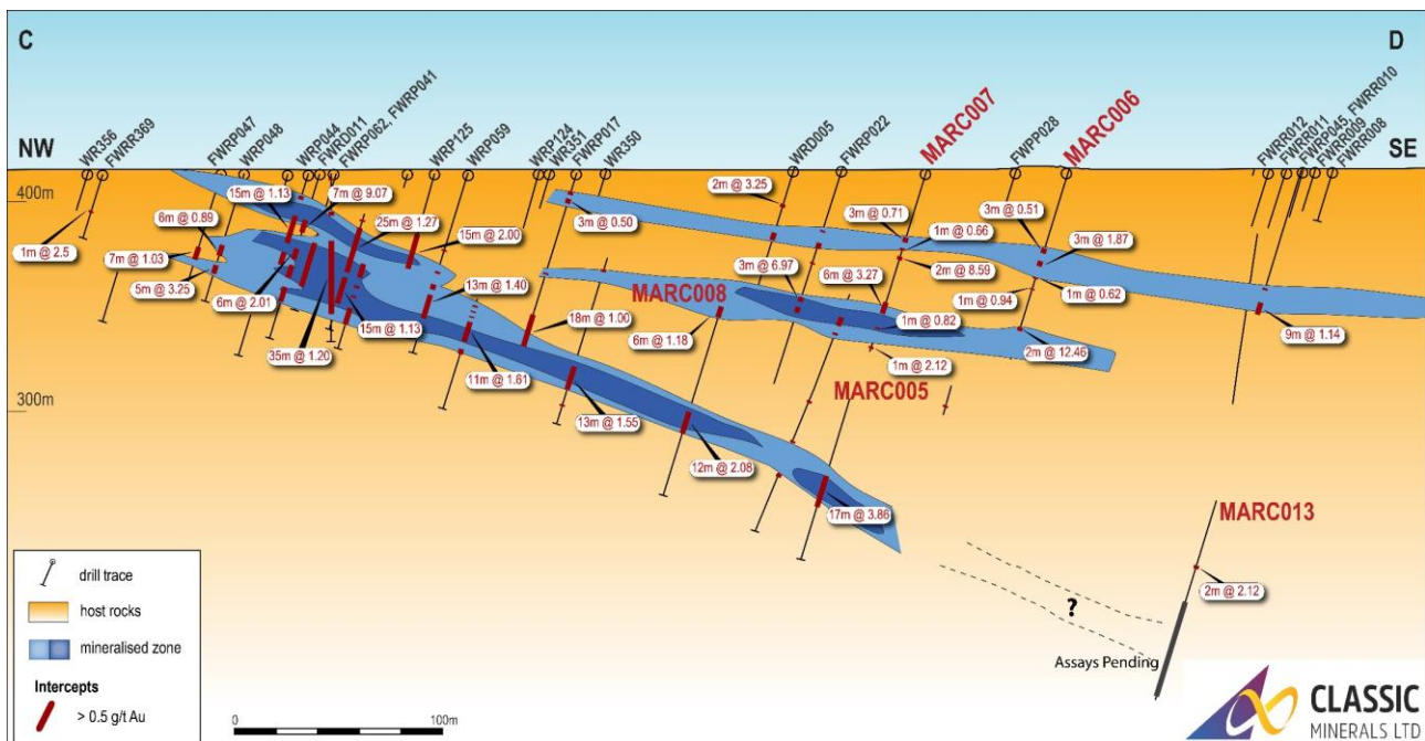
Figure 3 NW-SE section through Lady Magdalene, Showing results for MARC005, 006, 007, 008, and 0013
